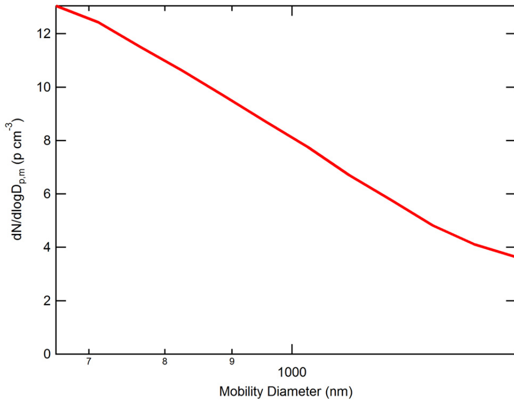
Figure S1. The average supermicron size distribution from the APS at T0 used to estimate the large particle contributions during the “missing” data period. Note that the f(\text{RH}) and \gamma model calculations are not particularly sensitive to the shape of this distribution because the scattering efficiency Q starts to reach an asymptotic limit in this size range.
