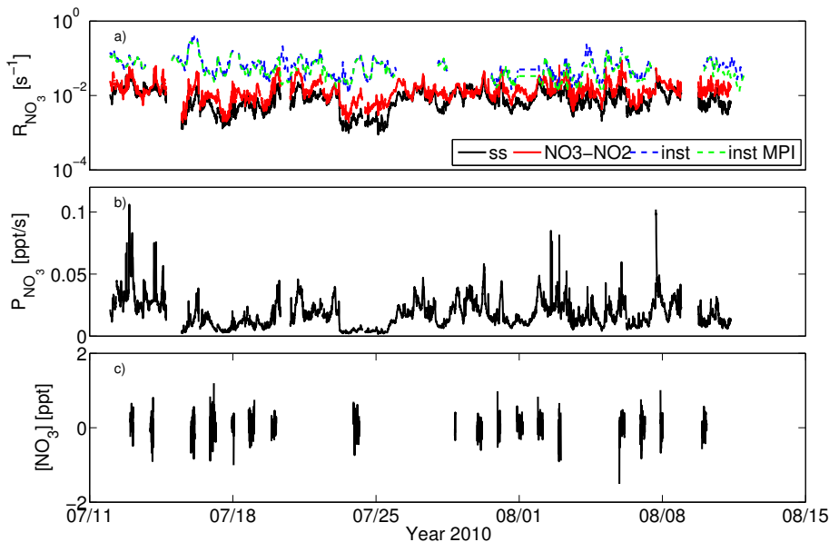
Figure 10. (a) The steady state (ss, in black) and instantaneous (inst, in dashed blue, when using SMEAR II \text{NO}_x concentrations, inst MPI, in dashed green, when using MPI \text{NO}_x concentrations) \text{NO}_3 -reactivity ( R_{\text{NO}_3} ) together with the the corrected steady state reactivity where also the reactions of \text{NO}_3 with \text{NO}_2 have been taken into account ( \text{NO}_3\text{-NO}_2 , in red), (b) the production term ( P_{\text{NO}_3} = k_6[\text{NO}_2][\text{O}_3] ) of \text{NO}_3 , and (c) the measured concentration of \text{NO}_3 ( [\text{NO}_3] ). Please note the log scale in the a section.
