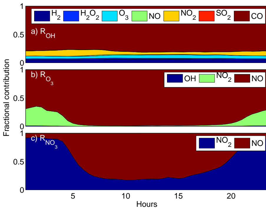
Figure 8. The daily averaged fractional contribution of individual inorganic compounds to the total inorganic reactivity of OH (a), O_3 (b) and NO_3 (c) at 18 m.
