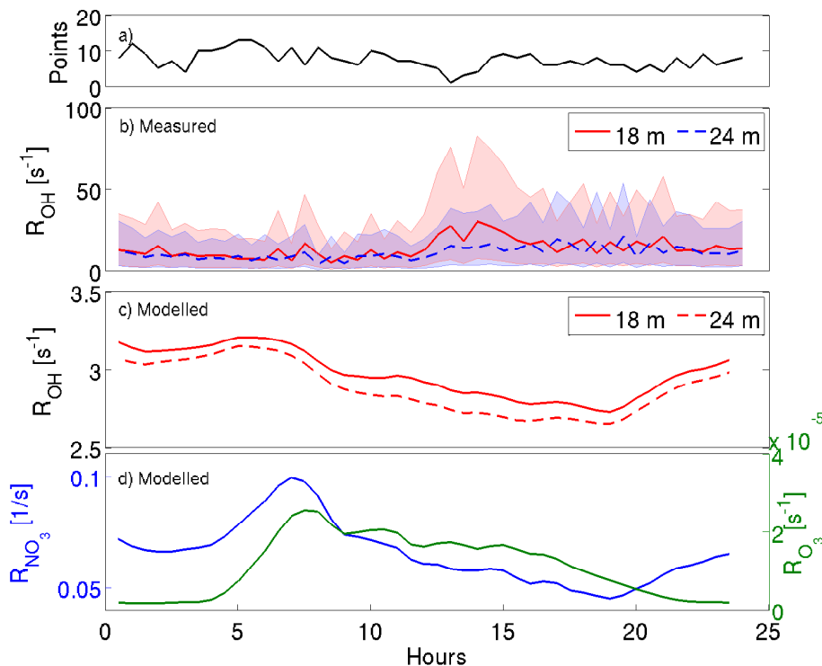
Figure 7. Daily averaged measured and modelled total OH-reactivity together with daily averaged modelled total O 3 - and NO 3 -reactivity. (a) indicates the amount of measured half hour data points that has been used for the averaging of the measured reactivity, (b) measured OH-reactivity at 18 (solid red line) and 24 m (dashed blue line), where the shaded areas are the 75 and 25 percentiles, (c) modelled OH-reactivity at 18 m (solid red line) and at 24 m (dashed red line), and (d) modelled reactivities of NO 3 (blue line, left sided y axis) and O 3 (green line, right sided y axis).
