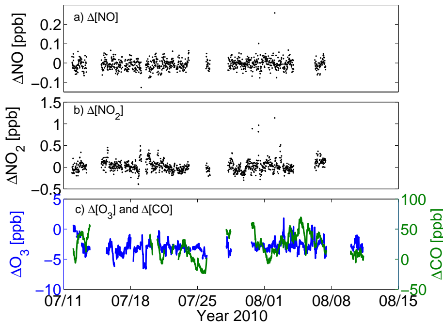
Figure 5. Difference in measured gas concentration of (a) NO, (b) NO 2 , and (c) O 3 (blue, left hand side) and CO (green, right hand side). The difference is calculated by subtracting the campaign measured concentrations by the SMEAR II obtained concentrations.
