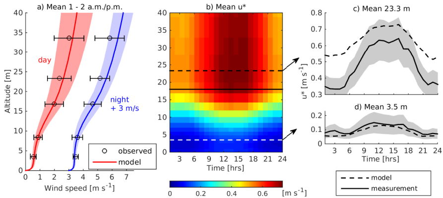
Figure 4. Average wind speed profile \pm SD at 1–2 a.m. and p.m. (a). Red and blue lines and area are simulated values for day and night (3 \text{m/s} added for clarity), respectively, black from measurements. Simulated diurnal mean friction velocity ( u^* ) (b). The top of the canopy is shown with a solid line and the measurement heights of the eddy covariance systems with dash lines. Observed and simulated mean friction velocity in (d) and above the canopy (c) . The shaded areas in the (c) and (d) represents the estimated uncertainty of \pm 20\% (c) and \pm 50\% (d) , respectively.
