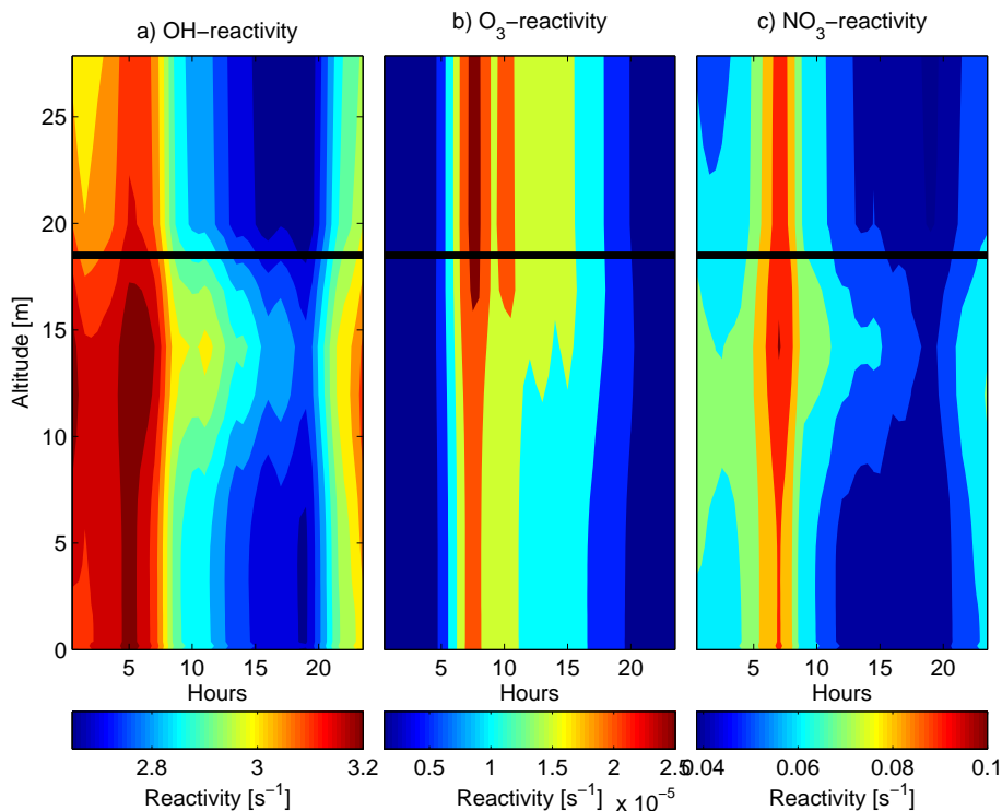
Figure 9. Daily averaged vertical total reactivity of OH (a), O 3 (b), and NO 3 (c). The top of the canopy is indicated by a black solid line.
