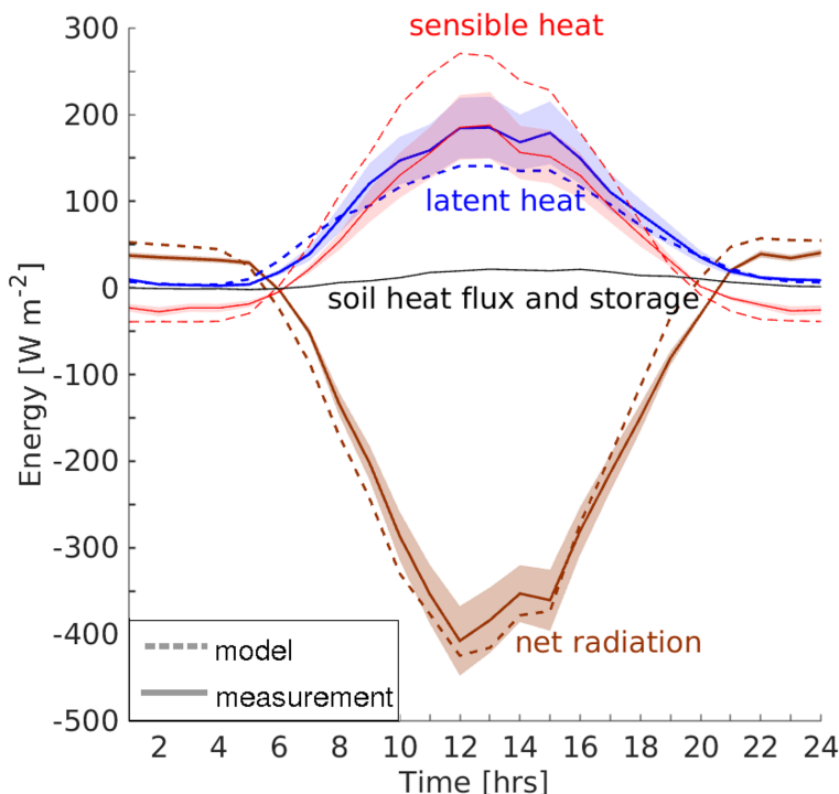
Figure 3. Diurnal averages of the components of the surface energy balance. Net radiation: sum of all radiation components in the model (the direct and diffuse global radiation, atmospheric thermal radiation, PAR and NIR reflected and emitted by the vegetative canopy, and the thermal radiation by the soil surface) compared to the net radiation measured for 300–40 000 nm above the canopy. Heat flux and storage in the soil is the average of four heat plates, and observed values were used as model input. Turbulent fluxes of sensible and latent heat measured with an eddy covariance system at 23.3 m. The shaded areas represents the uncertainty on the measurements which are estimated to be \pm 20\% for the heat fluxes and \pm 10\% for the net radiation.
