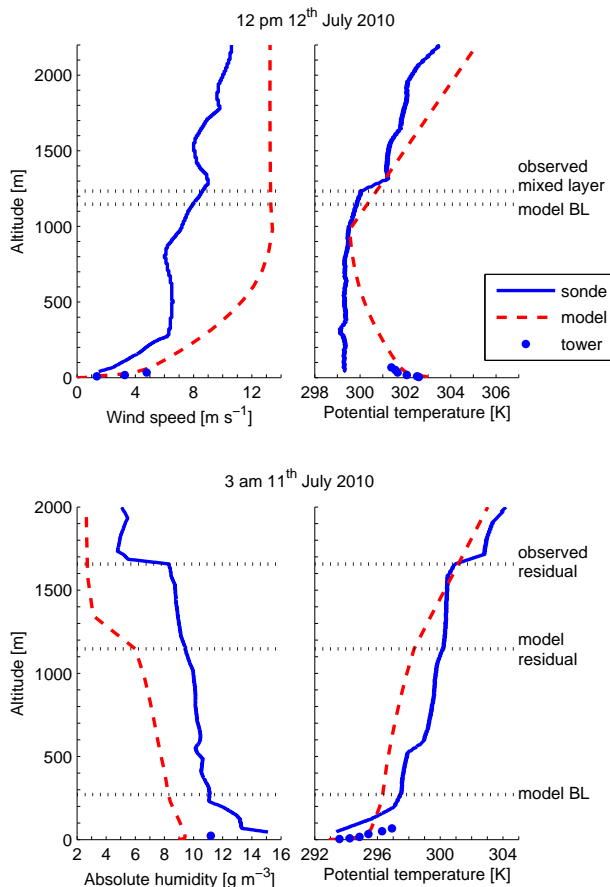
Figure 2. Examples of modelled and observed vertical profiles at 12 p.m. on 12 July (top) and 3 a.m. on 11 July (bottom). Solid lines are data obtained from radiosonde observations, and the dots are 30 min averages from the SMEAR II tower. The model values are representing the 30 min during which the soundings were made.
