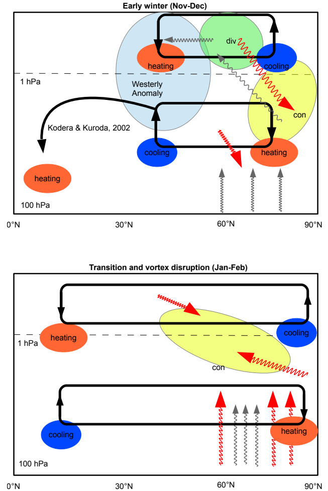
Figure 7. Solar cycle modulation of the winter circulation: schema of the related mechanisms. The upper and lower figure show early and later winter respectively. The heating and cooling anomalies are drawn with red and blue boxes. The EP flux divergence and convergence are drawn with green and yellow boxes. The wave propagation anomaly is expressed as a wavy red arrow in contrast to the climatological average drawn by a wavy grey arrow. The induced residual circulation according to the quasi-geostrophic approximation is highlighted by the bold black lines.
