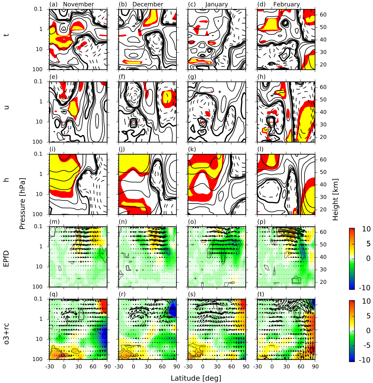
Figure 5. The monthly averaged response of the solar signal in the MERRA zonal-mean temperature t (a)-(d), unit: [K], contour levels: 0, \pm 0.25 , \pm 0.5 , \pm 1 , \pm 2 , \pm 5 , \pm 10 , \pm 15 , \pm 30 ; zonal wind u (e)-(h), unit: [m/s], contour levels: 0, \pm 1 , \pm 2 , \pm 5 , \pm 10 , \pm 15 , \pm 30 ; geopotential height h (j)-(l), unit: [gpm], contour levels: 0, \pm 10 , \pm 20 , \pm 50 , \pm 100 , \pm 150 , \pm 300 ; EP flux divergence EPfD (m)-(p), unit: [m/s/day]; together with EP flux vectors scaled by the inverse of the pressure, unit: [kg/s 2 ]; and ozone mixing ratio, unit: percentage change per monthly mean; with residual circulation o3+rc (q)-(t), units: [m/s; -10^{-3} Pa/s] during northern hemispheric winter. The response is expressed as a regression coefficient (corresponding units per S_{max} minus S_{min} ). The statistical significance of the scalar fields was computed by a t-test. Red and yellow areas in Figs. (a)-(l) and grey contours in Figs. (m)-(t) indicate p-values of < 0.05 and 0.01 respectively.
