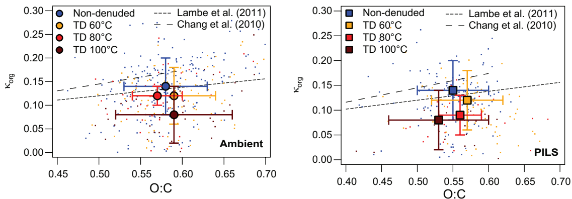
Fig. 5. Variation in \kappa_{\text{org}} with O:C for ambient aerosol at s = 0.20\% and PILS aerosol at s = 0.40\% for non-denuded and thermally-denuded conditions. Small colored dots indicate all measured points while larger circles and squares indicate the averages for while errors. Errors bars indicate one SD standard deviation in measured values for ambient and PILS aerosol, respectively. Also shown are dashed lines indicating the parameterizations of \kappa_{\text{org}} with O:C from Lambe et al. (2011) and Chang et al. (2010).
