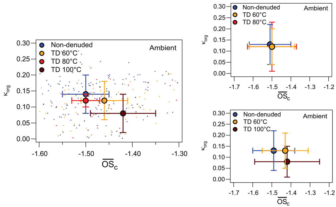
Fig. 6. Variation in \kappa_{\text{org}} with \overline{\text{OS}}_c for ambient aerosol at s = 0.20\% for the total study period (left) and for 80 and 100°C measurement periods only (right top and bottom, respectively). Small colored dots indicate all measured points while larger circles indicate measurement averages and errors bars indicate a single SD in measured values.
