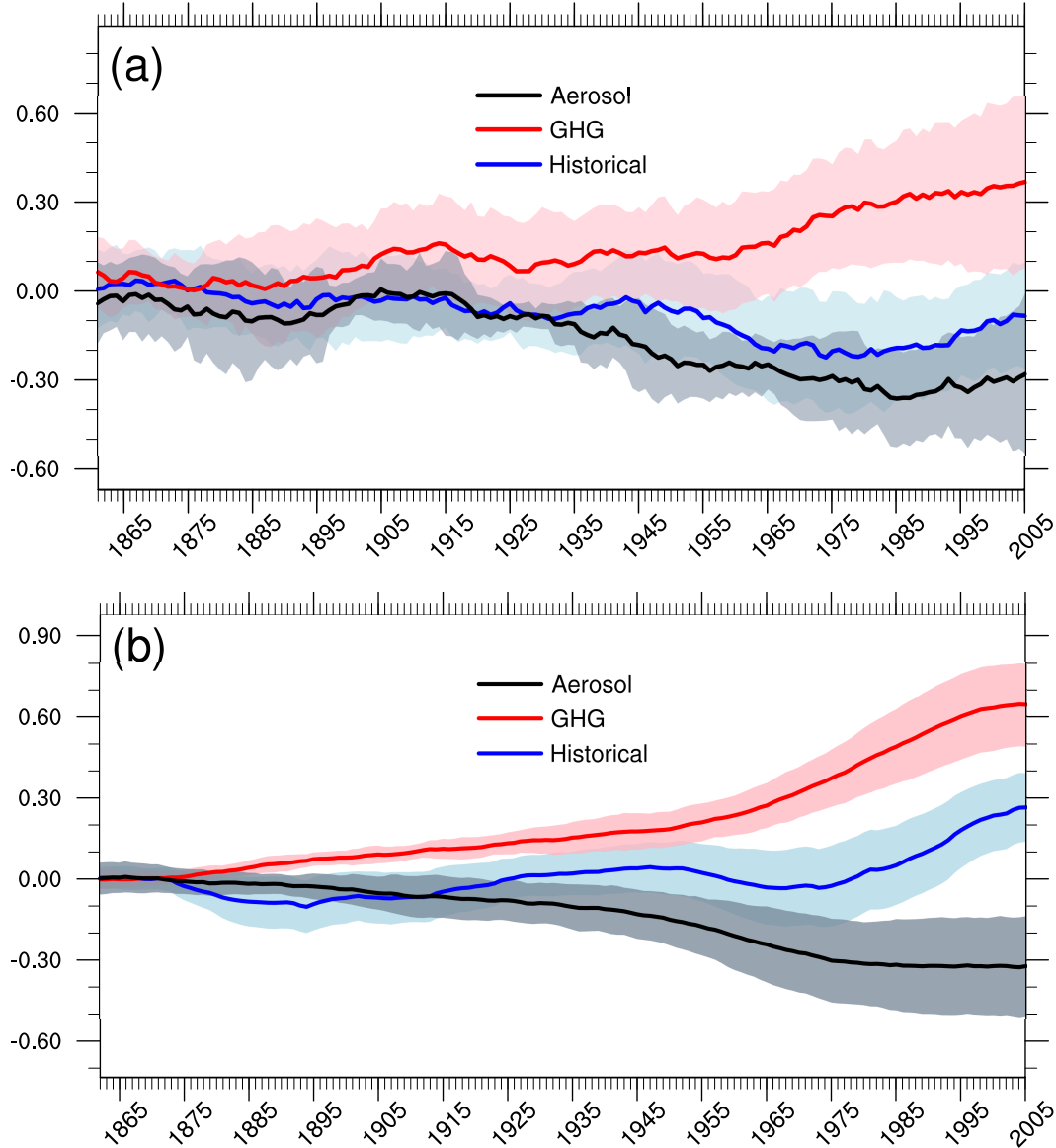
Figure 1. (a) JJAS rainfall from 1861–2005 averaged over South Asia ( 10\text{--}35^\circ\text{N} , 70\text{--}90^\circ\text{E} ) in the CMIP5 all-forcings historical experiment (blue), GHG-only historical experiment (red) and the aerosol-only historical experiment (black). The thick lines show MME-means with a 21-year running mean applied, while the pale envelope indicates the \pm 1\sigma range from the mean. Only eight models are used in constructing this figure (see Section 2): CanESM2, CCSM4, CSIRO-Mk3.6.0, GFDL-CM3, GFDL-ESM2M, HadGEM2-ES, IPSL-CM5A-LR & NorESM1-M. The curves are centred around zero by removing the mean rainfall from pre-industrial control runs ( piControl ) of the same models. Units are \text{mm day}^{-1} . (b) Same as (a) but for the global mean and annual mean land-sea surface temperature contrast from 1861–2005. Units are K.
