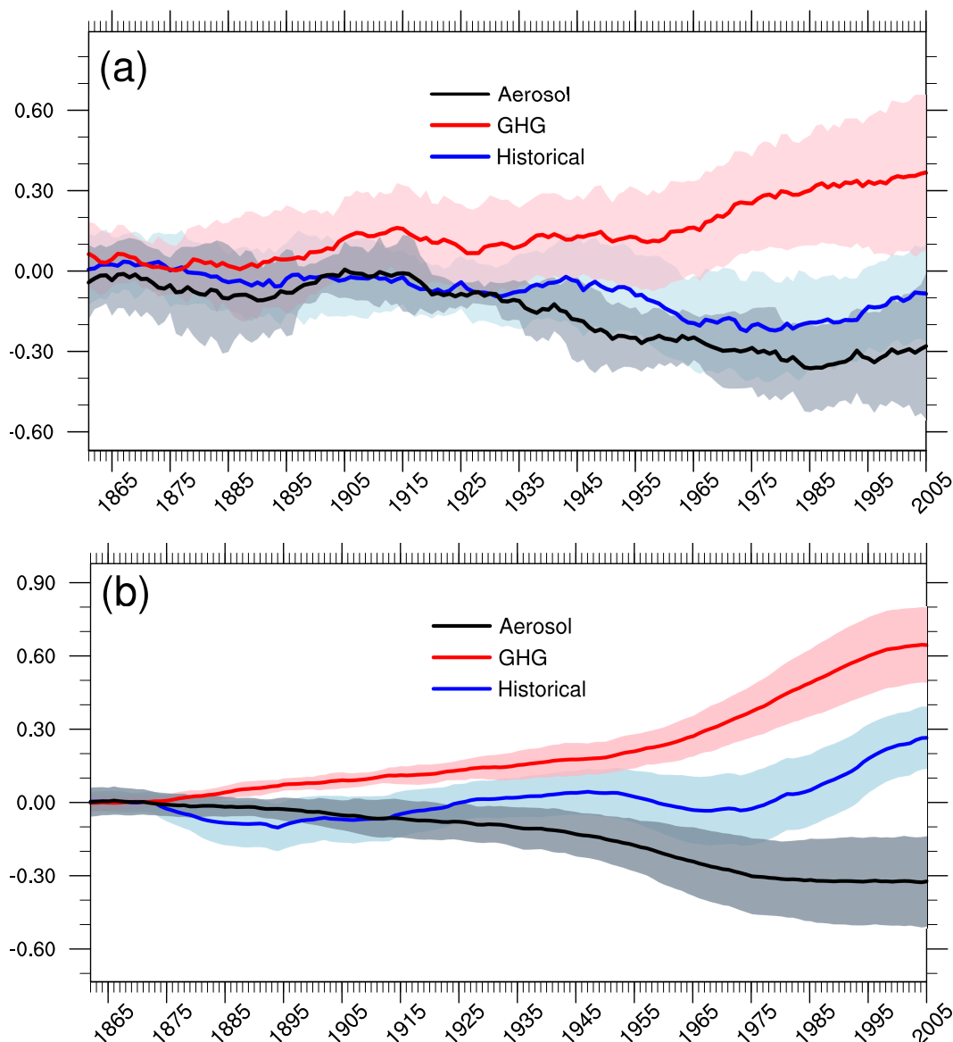
Figure 1. (a) JJAS rainfall from 1861–2005 averaged over South Asia (10–35°N, 70–90°E) in the CMIP5 all-forcings historical experiment (blue), GHG-only historical experiment (red) and the aerosol-only historical experiment (black). The thick lines show MME-means with a 21-year running mean applied, while the pale envelope indicates the \pm 1\sigma range from the mean. Only eight models are used in constructing this figure (see Section 2): CanESM2, CCSM4, CSIRO-Mk3.6.0, GFDL-CM3, GFDL-ESM2M, HadGEM2-ES, IPSL-CM5A-LR & NorESM1-M. The curves are centred around zero by removing the mean rainfall from pre-industrial control runs ( piControl ) of the same models. Units are \text{mm day}^{-1} . (b) Same as (a) but for the global mean and annual mean land-sea surface temperature contrast from 1861–2005. Units are K.
