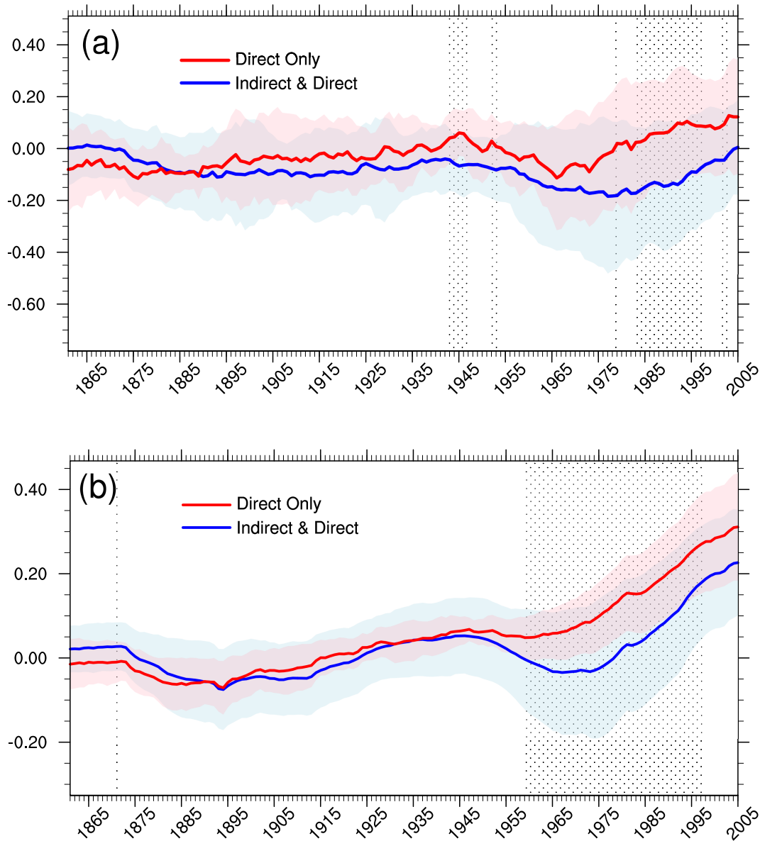
Figure 2. (a) JJAS rainfall from 1861–2005 averaged over South Asia ( 10\text{--}35^\circ\text{N} , 70\text{--}90^\circ\text{E} ) in twenty-four CMIP5 models which have all-forcing historical experiments. The models are divided into two groups, the direct effect only models (red) and the indirect effect included models (blue), as shown in Table 1. The thick lines show MME-means with a 21-year running mean applied, while the pale envelope indicates the \pm 1\sigma range from the mean. Differences exceeding the 90% significant level using a permutation test are stippled. The curves are centred around zero by removing the mean rainfall from pre-industrial control runs ( piControl ) of the same models. Units are \text{mm day}^{-1} . (b) Same as (a) but for the global mean and annual mean land-sea surface temperature contrast from 1861–2005. Units are K.
