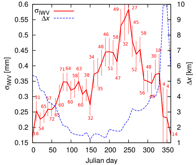
Figure 4. \sigma_{\text{IWV}} as a function of Julian day. The coincidence interval is 20 minutes in this case, pairs within 30 days were taken into account. The quantity of measurement pairs from which \sigma_{\text{IWV}} was calculated is indicated by the numbers near the curve. The dashed line shows the mean horizontal distance between the pairwise soundings of IWV as a function of the season. The uncertainties ( \pm\sigma ) are indicated by the error bars (for calculation see text).
