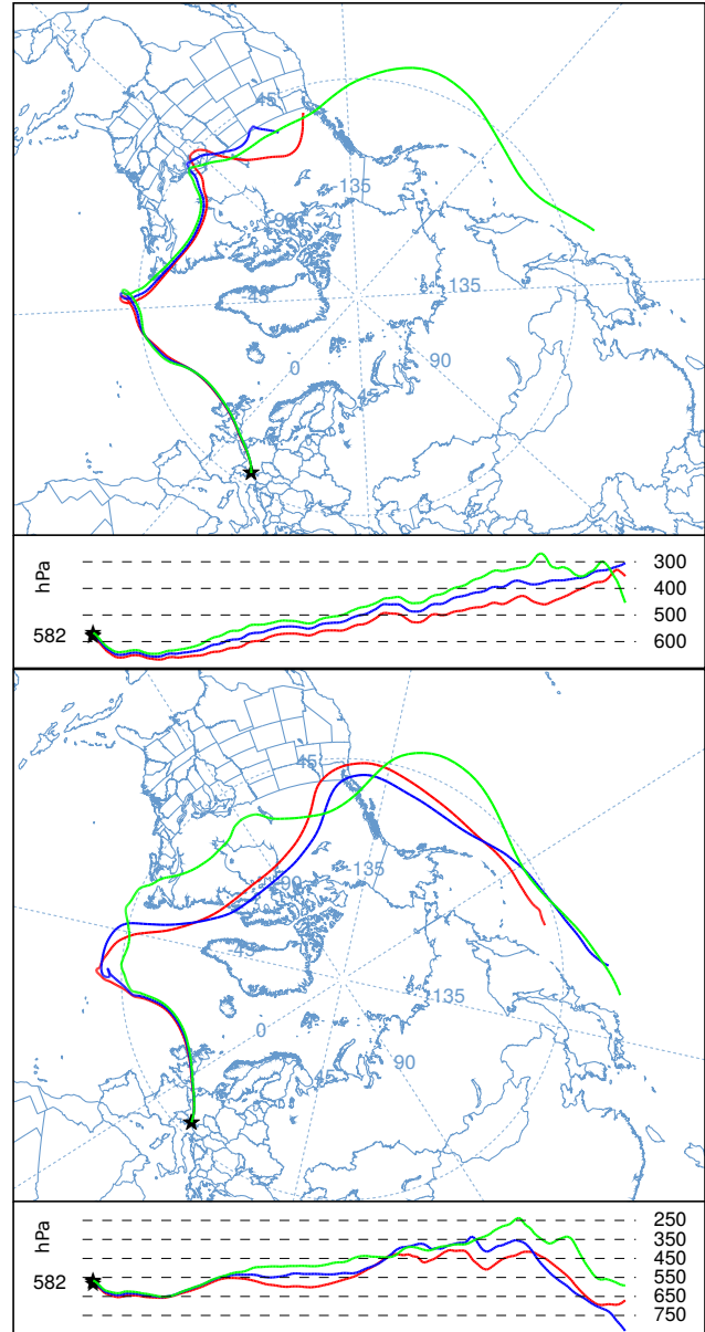
Figure 12. Backward trajectories from the NOAA HYSPLIT model (see text) ending above Mt. Zugspitze at 4600 m, 4700 m and 4800 m a.s.l. at 6:00 UTC (upper plot) and 8:00 UTC (lower plot), July 29, 2009 were calculated from reanalysis data with a vertical velocity model and a duration of 315 hours. The vertical sections are referred to the air pressure along the pathways. The remarkable coherence of the three pathways during a longer time indicates a rather good reliability.
