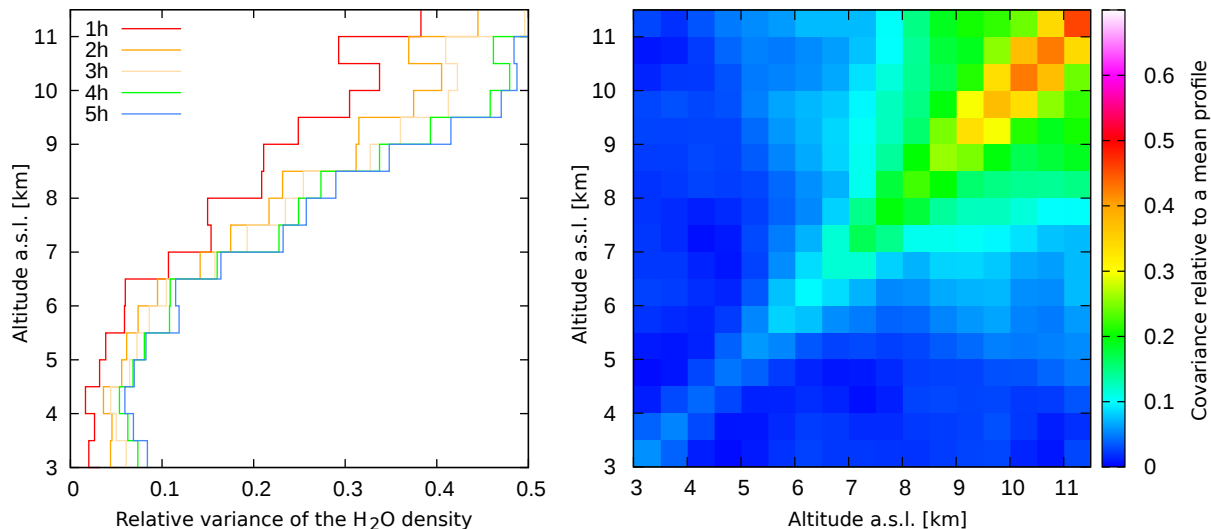
Figure 6. The short-term variability of the vertical water vapor profile is illustrated by the plot of the relative variance as a function of altitude within different time intervals (left plot). The covariance matrix (right plot) gives an idea of the interconnectivity of the variation between different altitudes.
