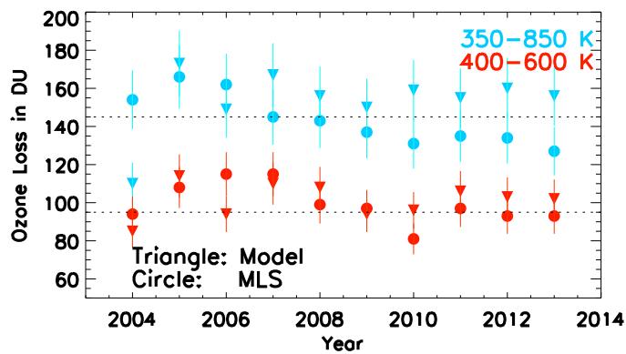
Fig. 6. Vortex averaged (defined by \geq 65^\circ EqL) column ozone loss computed from model simulations and measurements, during the maximum ozone loss period in the Antarctic, at 350–850 K and 400–600 K for the 2004–2013 period. The estimated uncertainty of the column loss computed from both simulations and measurements is about 10 % (e.g. Kuttippurath et al., 2011).
