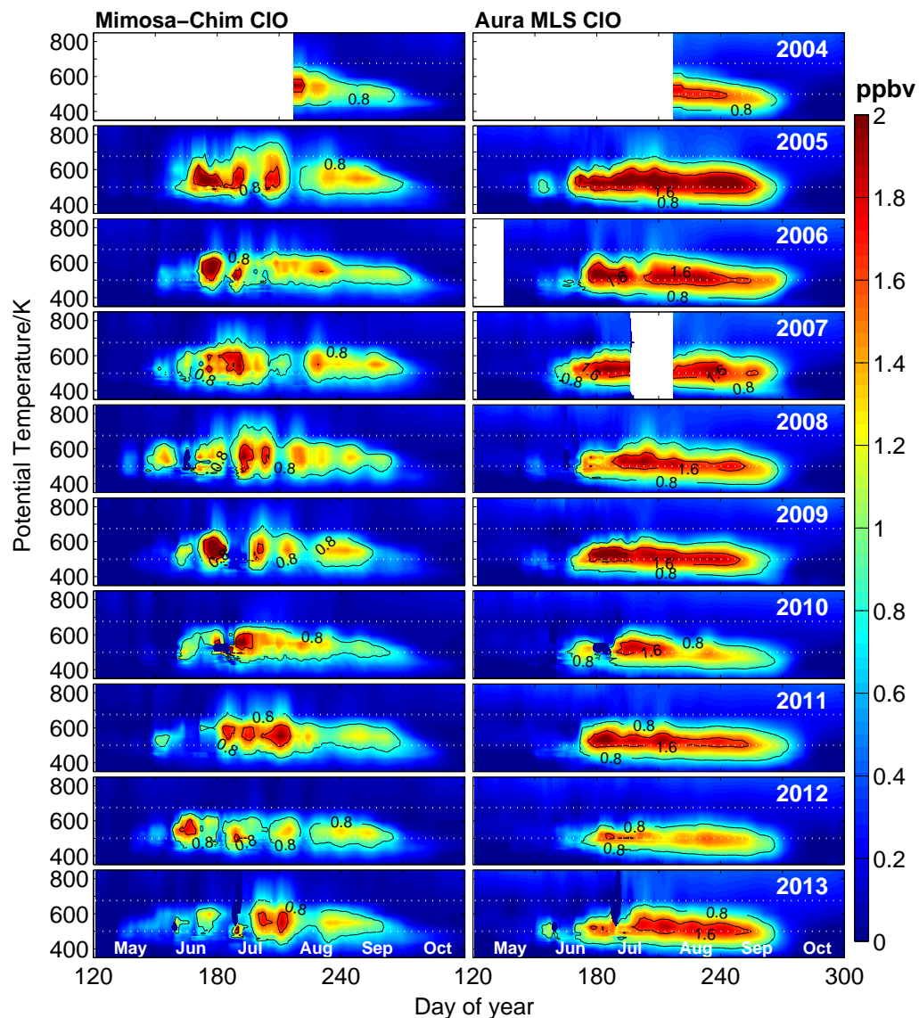
Fig. 3. Vertical distribution of the vortex averaged (defined by \geq 65^\circ EqL) CIO estimated from the Mimosa-Chim model and MLS measurements for the Antarctic winters 2004–2013. The model results are interpolated with respect to the time and location of the MLS measurements inside the vortex and then averaged for the corresponding day. CIO data are not available during early May 2006, and late July and early August 2007. The measurements are selected with respect to local solar time 10–16 h and solar zenith angles below 89^\circ as available. Both model results and MLS data are smoothed for seven days. The Y-axis represents potential temperature in Kelvin (K). The white dotted lines represent 500 K ( \sim 19 km) and 675 K ( \sim 26 km).
