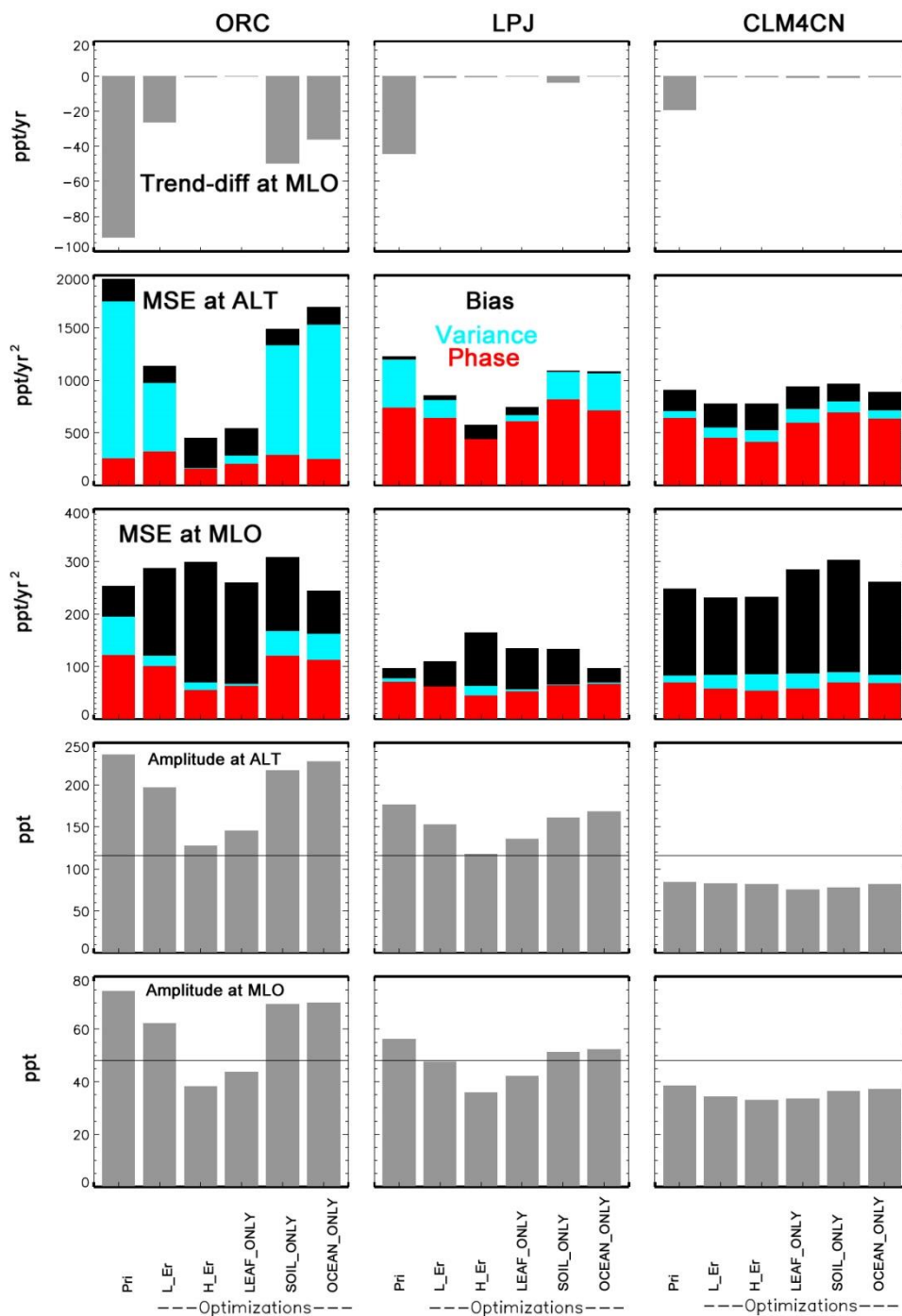
6 Figure 11: Upper row: differences in annual trends (in ppt yr -1 ) between simulated monthly mean OCS mixing ratios 7 and measurements, at Mauna Loa. Second and third rows: analysis of smoothed seasonal cycles in simulations and 8 observations (at Alert and Mauna Loa, respectively), and calculation of the mean square error (MSE, in ppt 2 ) 9 decomposed into three components (bias, phase and variance, as described by Kobayashi and Salam (2000)). Fourth
