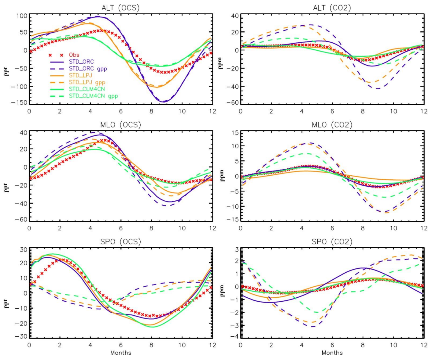
3 Figure 6: Average smoothed seasonal cycles of OCS (left column) and CO 2 (right column) monthly mean 4 mixing ratios, simulated at ALT, MLO and SPO, and obtained after removing the annual trends. OCS cycles 5 simulated with the LMDz model using the “STD_ORC”, “STD_LPJ” and “STD_CLM4CN” setups (Table 6 1). The dashed lines represent the smoothed seasonal cycles of the OCS (left column) and CO 2 (right 7 column) monthly mean mixing ratios when only the contribution of the leaf OCS uptake (resp. the GPPs) of 8 the three vegetation models are used in the LMDz transport model (“ORC gpp”, “CLM4CN gpp” and “LPJ 9 gpp”). Observations (red crosses) are from NOAA-ESRL global monitoring network (Montzka et al., 2007).
