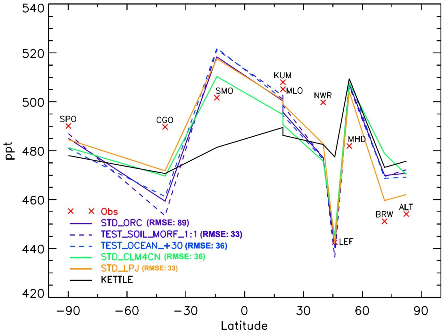
3 Figure 7: Differences in OCS annual mean mixing ratios between 10 stations of the NOAA monitoring 4 network, plotted as a function of latitude, for observations (red crosses surmounted by station acronyms) and 5 simulations (no symbol). Note that the global mean for each mixing ratio series has been set to the global 6 mean of the observations. Simulations obtained with the LMDz model using the “STD_ORC”, 7 “STD_CLM4CN” and “STD_LPJ” setups (Table 1). Data derived solely from the Kettle et al. (2002) 8 surface fluxes are shown in black solid line. The sensitivity of latitudinal gradients to changes in soil uptake 9 and ocean emissions (dashed colored lines) was investigated using the “TEST_Soil_MORF_1:1 +30%” and 10 “TEST_Ocean_+30%” setups.
