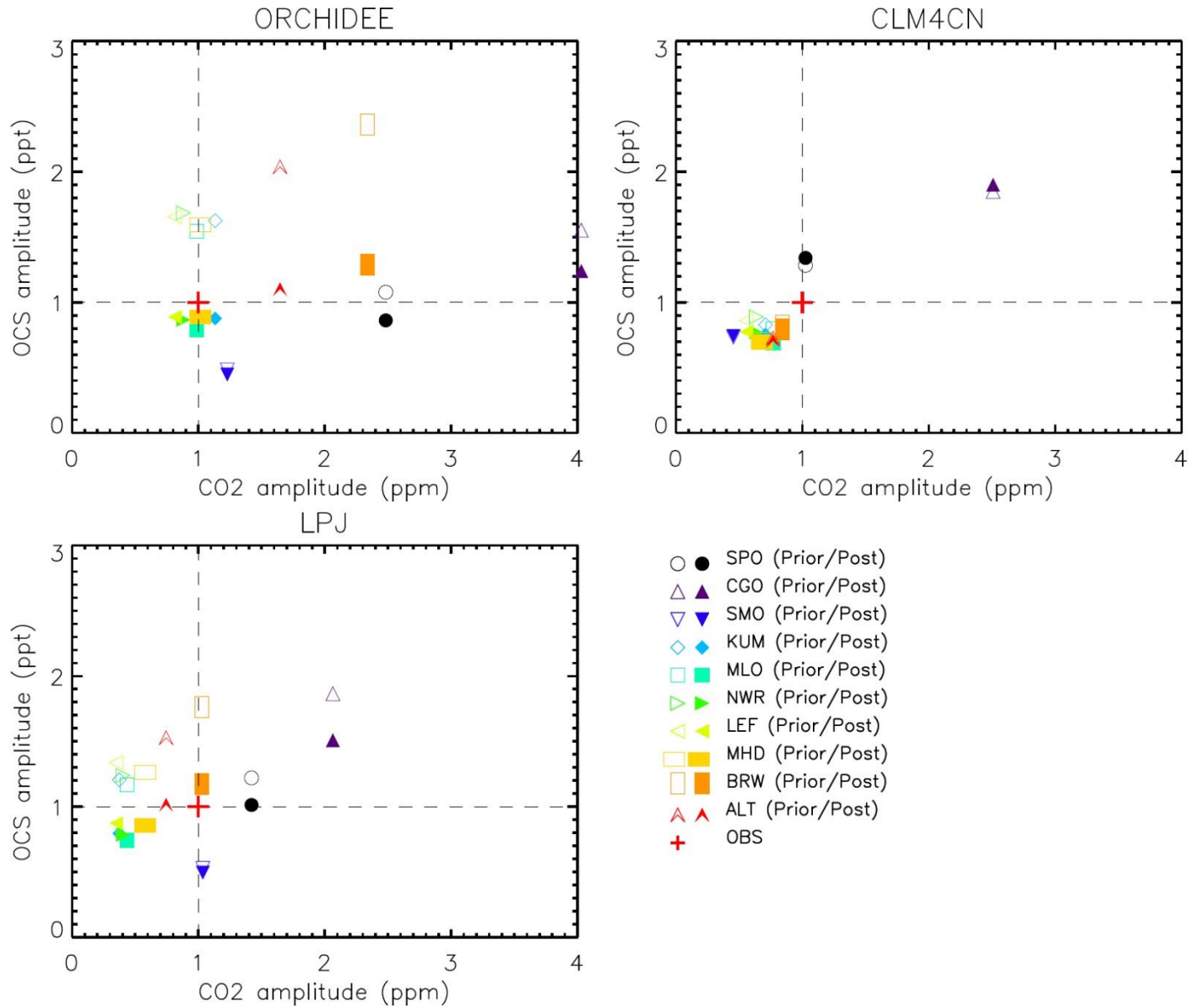
6 7 Figure 12: Scatter plots of normalized amplitudes of smoothed seasonal cycles of OCS versus those of CO 2 , 8 before (open symbols) and after optimization (filled symbols) of OCS fluxes at 10 stations of the NOAA 9 monitoring network, obtained from the “STD_ORC”, “STD_CLM4CN” and “STD_LPJ” setups for the 10 forward simulations and the “OPTIM_H-Er” setup for the optimizations, over the period 2006-2010. Since 11 the amplitude of the seasonal cycle in the observations at each site is used to normalize that of the 12 simulations, the normalized amplitude of observations is 1 (red cross). Hence, a linear translation along the 13 Y-axis towards Y = 1 characterizes the optimization process.
