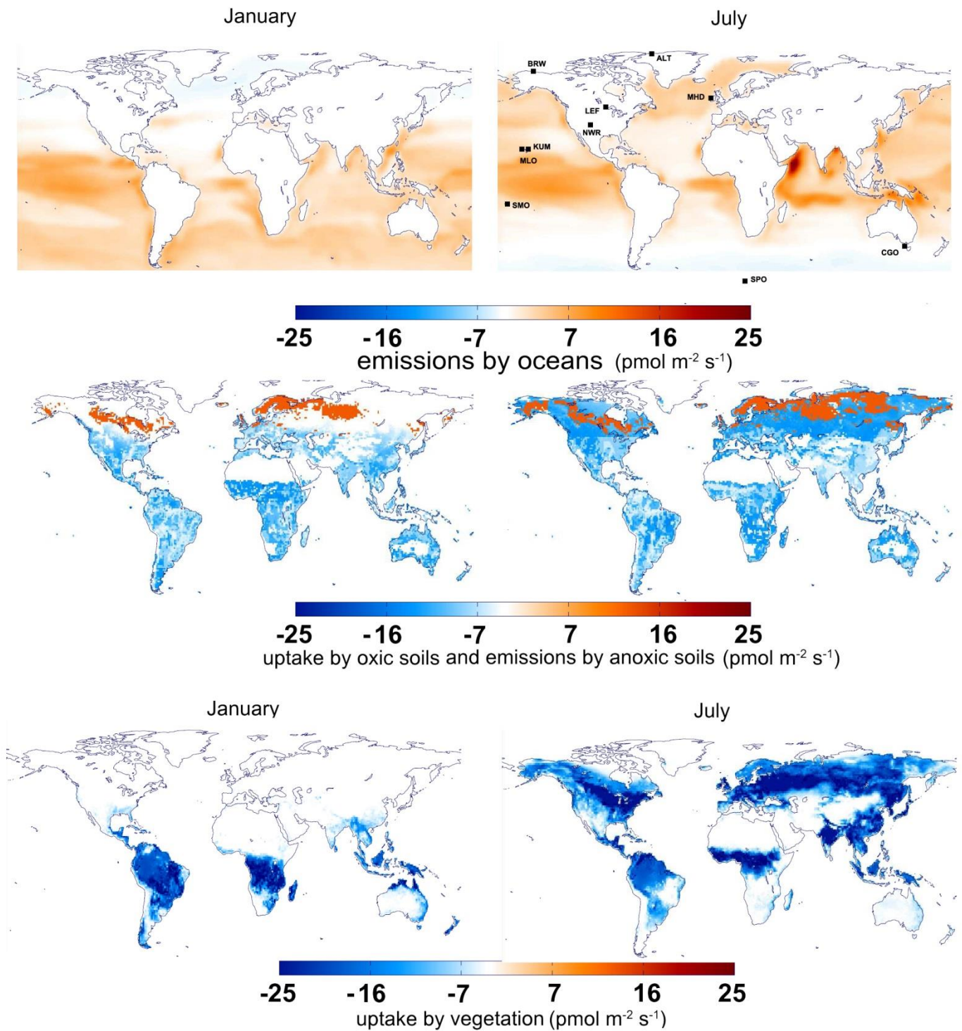
2 Figure 1: Monthly mean direct oceanic emissions (first row, from the standard run of Launois et al. (2014)) 3 for January (left column) and July (right column), monthly mean uptake of OCS by soils (second row, using 4 \text{H}_2 deposition velocities (Morfopoulos et al., 2012) and OCS vs. \text{H}_2 deposition velocities in a 0.75:1 ratio) 5 and vegetation (third row, deduced from the GPP of ORC). The 10 NOAA stations are: SPO, South Pole, 6 89.9°S, 59°E; CGO, Cape Grim, Australia, 40.7°S, 144.8°E; SMO, American Samoa, 14.3°S, 170.6°W; 7 MLO, Mauna Loa, United States, 19.5°N, 155.6°W; NWR, Niwot Ridge, United States, 40.1°N, 105.6°W; 8 BRW, Barrow, United States, 71.3°N, 156.6°W; ALT, Alert, Canada, 82.5°N, 62.3°W; MHD, Mace Head,
