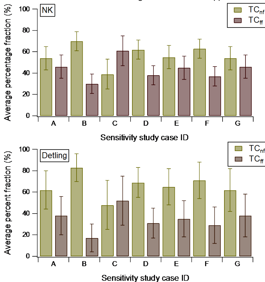
Figure S6: Daily average percentage of non-fossil total carbon fraction ( TC_{nf} ) and the total carbon fossil fraction ( TC_{ff} ) as calculated using different source ratios. For details on the source ratios used, refer to the case ID given in Table 4.
