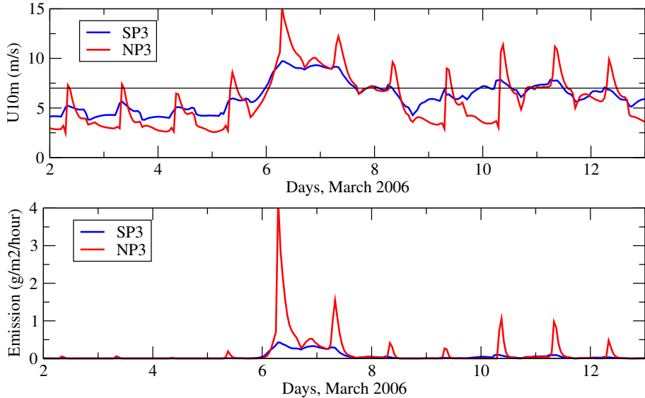
Figure 3. Comparison from 2 to 13 March 2006 of the 10 m wind (upper panel, \text{m s}^{-1} ) and emission (lower panel, \text{g m}^{-2} \text{h}^{-1} ) for simulations SP3 (blue) and NP3 (red) in the grid cell selected for emission analysis at ( 7.5^\circ \text{ W} , 18.5^\circ \text{ N} ) (shown in red in Fig. 1). The horizontal line in the upper panel corresponds to a wind of 7 \text{ m s}^{-1} above which emissions start to be significant.
