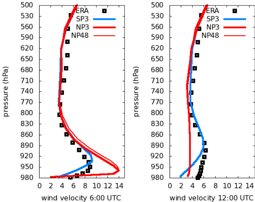
Figure 8. Wind mean vertical profiles (m s -1 ) for JFM 2006 at 06:00 and 12:00 UTC at Banizoumbou. Model results (colored curves) are compared to ERAI (black squares) for the same time period.
