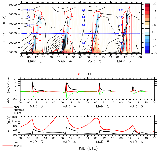
Figure 9. Four consecutive days showing the diurnal cycle of the boundary layer at Banizoumbou, in early March 2006. Are shown in the upper panel: the vertical distribution of the module of the horizontal wind (black contours, \text{m s}^{-1} ), the wind module tendency due to vertical transport by the thermal plume model, according to Eq. (7) (colored shades with absolute iso-values 0.5, 1, 2, 3, 5, 10 and 20 \text{ m s}^{-1} \text{ h}^{-1} ). The red contour delimits the depth of the boundary layer and corresponds to the 0.25 value of the bulk Richardson number (Eq. 8). The red arrows correspond to the thermal plume velocity in \text{m s}^{-1} (under-sampled with respect to the space–time discretization of the simulation). The vertical axis, in pressure (Pa), and the altitude (in km, blue contours) are also shown. In the middle panel, we show for the first model layer (located at about 30 m above surface) the decomposition of the total wind module tendency (TOTAL, red, \text{m s}^{-1} \text{ h}^{-1} ) as the sum of the thermal plume contribution (THERMAS, black) and turbulent diffusion (TKE, green). The lower panel shows the wind speed at 10 m (black) and 950 hPa (red), close to the altitude where the nocturnal jet reaches its maximum.
