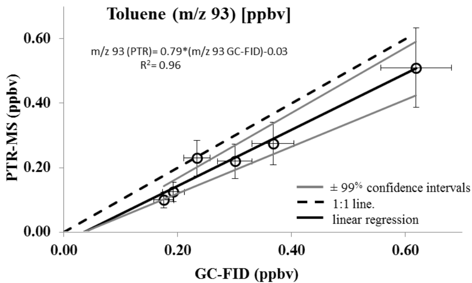
Figure S-2. Scatter plots of VOC concentrations (ppbv) (benzene and toluene) of PTR-MS against WAS TD-GC-FID measurements at 360 \pm 10 m a.g.l.
