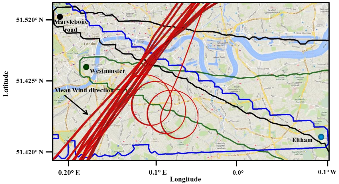
Figure S-1. Flight track and NOAA HYSPLIT particle dispersion plots for three LAQN ground monitoring sites located in Greater London during RF 5 (10:30 – 13:00 local time, 3/7/13).
