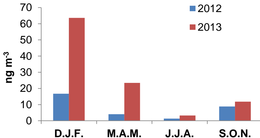
Figure 1. \Sigma PAH median air concentrations in winter (D.J.F.), spring (M.A.M.), summer (J.J.A.), and autumn (S.O.N.) at Košetice.
