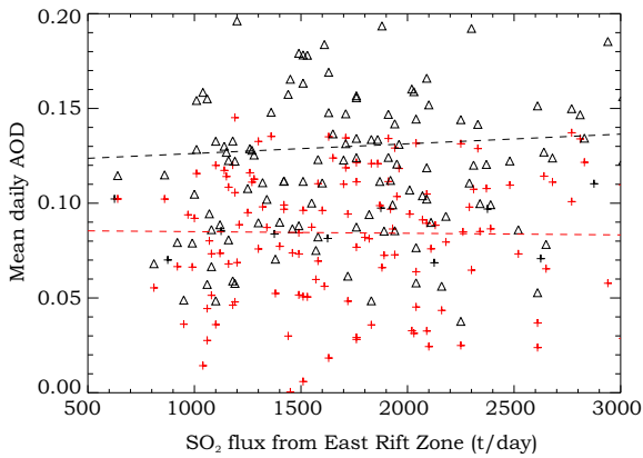
Fig. 6. Comparison of SO 2 flux from East Rift as reported by (Elias and Sutton, 2012), with AOD (550 nm) measurements from MODIS Aqua on the same day. The lack of relationship between ground and satellite-based measurements may be due to several factors including dilution effects and differences in measurement times. Black triangles show MODIS AOD retrievals and the black dashed line indicates linear regression line. The red crosses show AOD values after de-trending for a linear relationship with windspeed, as demonstrated in Figure 11. The red dashed line shows corrected linear regression.
