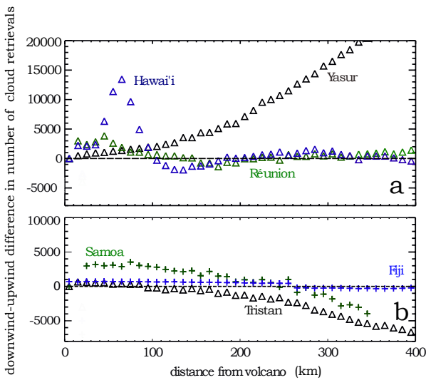
Fig. 7. Plots of the difference between numbers of cloud retrievals (cloud fraction > 0.2) downwind and upwind of volcanic vents (a) and island summits (b) from MODIS (Aqua), 2002–2008. At Hawai'i, and to some extent Réunion, there is a notable increase in the number of cloud retrievals made downwind relative to upwind within 100 km of the island.
