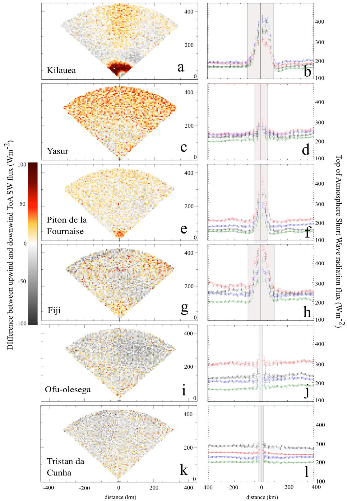
Fig. 5. Scatterplots showing the difference between upwind and downwind Top of Atmosphere Short-Wave flux (a, c, e, g, i, k) for volcanoes and ‘controls’. Positive values indicate higher SW flux downwind of the volcano. Profiles (b, d, f, h, j, l) indicate seasonal average SW fluxes for arcs of \frac{\pi}{2} at equal distance upwind and downwind from the volcano or island. December–February is red, March–May is blue, June–August is green and September–November is black.
