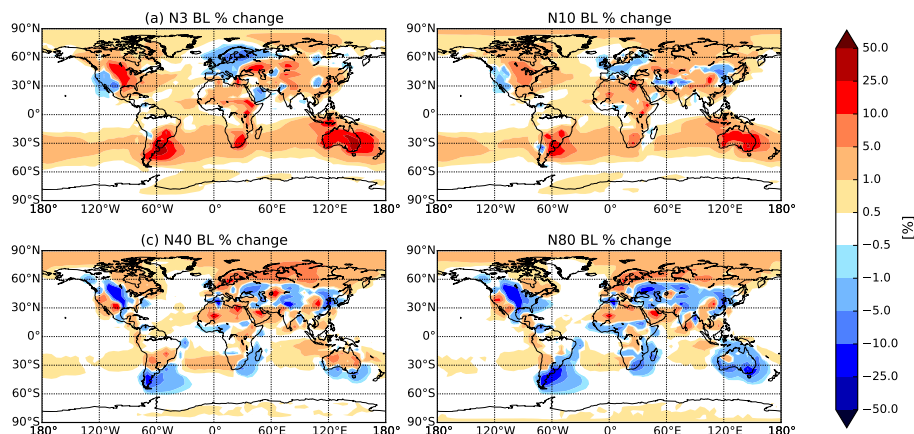
Figure 6. Percentage change in annually averaged boundary layer (a) N3, (b) N10, (c) N40 and (d) N80 when changing MEGAN BVOC emissions from year 1000 to year 2000 with anthropogenic emissions off (BE2.AEO.meg–BE1.AEO.meg). Globally averaged, N3, N10 and N40 increased by 3.2, 1.9 and 0.4 % respectively, whereas N80 decreased by 0.6 % (see Table 2). An increase in particle number concentration is represented by red colors, and a decrease in blue.
