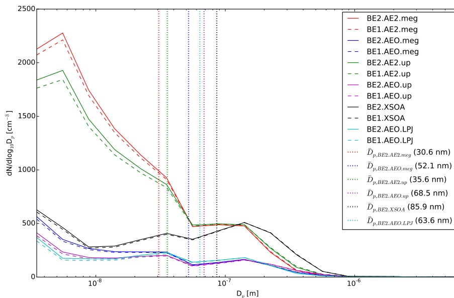
Figure 7. Simulated global boundary layer annual-mean particle number size distributions for the simulations outlined in Table 1. The vertical dotted lines represent the mean diameter for the simulations using year 2000 biogenic emissions (BE2.AE2.meg, BE2.AEO.meg, BE2.AE2.up, BE2.AEO.up, BE2.XSOA and BE2.AEO.LPJ).
