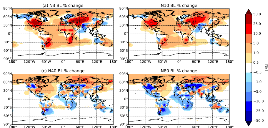
Figure 9. Percentage change in annually averaged boundary layer (a) N3, (b) N10, (c) N40 and (d) N80 when changing LPJ-GUESS BVOC emissions from year 1000 to year 2000 with anthropogenic emissions off (BE2.AEO.LPJ–BE1.AEO.LPJ). Globally averaged, N3 and N10 increased by 5.9 and 3.5% respectively, whereas N40 and N80 decreased by 0.1 and 1.8% respectively (see Table 2). An increase in particle number concentration is represented by red colors, and a decrease in blue.
