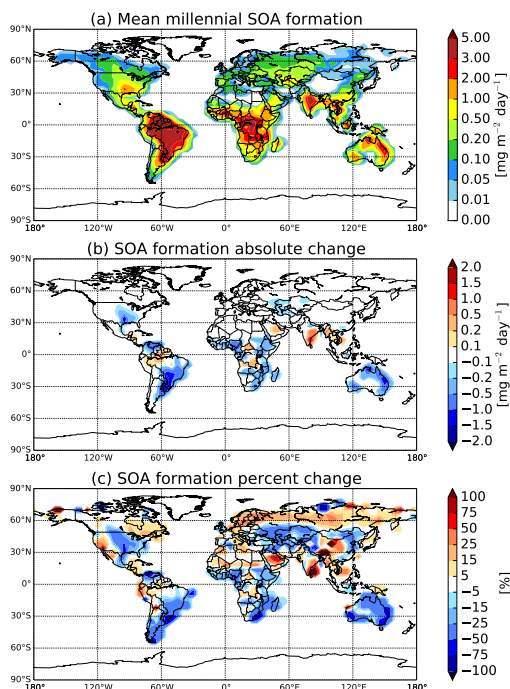
Figure 2. (a) Mean millennial fixed yield biogenic SOA formation from MEGAN emissions between the periods 1000–2000 in \text{mg m}^{-2} \text{ day}^{-1} , (b) absolute change in fixed yield biogenic SOA formation from averaged MEGAN BVOC emissions (monoterpenes, isoprene and sesquiterpenes) between 1000 and 2000 in \text{mg m}^{-2} \text{ day}^{-1} , and (c) relative change in fixed yield biogenic SOA formation from averaged MEGAN BVOC emissions (monoterpenes, isoprene and sesquiterpenes) between 1000 and 2000. An increase in SOA formation in (b) and (c) is represented by red colors, and a decrease in SOA formation by blue.
