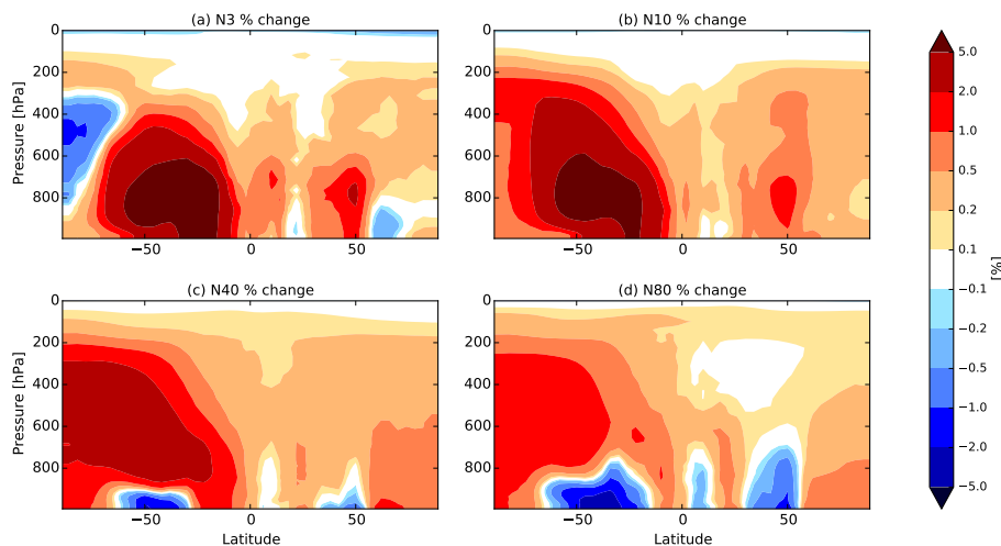
Figure 5. Zonal-mean annual-average percentage change in (a) N3, (b) N10, (c) N40 and (d) N80 when changing MEGAN BVOC emissions from year 1000 to year 2000 with constant present day anthropogenic emissions (2005) (BE2.AE2.meg–BE1.AE2.meg). An increase in particle number concentration is represented by red colors, and a decrease in blue.
