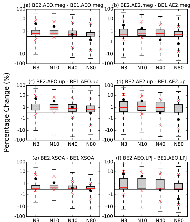
Figure 10. Global percent changes in N3, N10, N40 and N80 for biogenic emissions from 1000 to 2000 on a logarithmic scale for the simulations (a) BE2.AEO.meg–BE1.AEO.meg, (b) BE2.AE2.meg–BE1.AE2.meg, (c) BE2.AEO.up–BE1.AEO.up, (d) BE2.AE2.up–BE1.AE2.up, (e) BE2.XSOA–BE1.XSOA, and (f) BE2.AEO.LPJ–BE1.AEO.LPJ. The black dots indicate the global mean, the red line is the global median, the grey boxes are the interquartile range, the whiskers are the global maximum and minimum changes and the red X's indicate the 5th and 95th percentiles (see Table 2).
