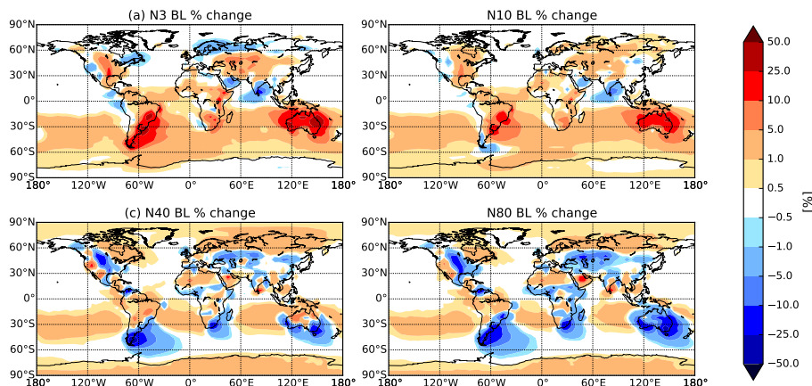
Figure 4. Percentage change in annually averaged boundary layer (a) N3, (b) N10, (c) N40 and (d) N80 (number of particles with diameter greater than 3, 10, 40 and 80 nm respectively) when changing MEGAN BVOC emissions from year 1000 to year 2000 with constant present day anthropogenic emissions (2005) (BE2.AE2.meg–BE1.AE2.meg). Globally averaged, N3 and N10 increased by 2.3 and 1.5 % respectively, whereas N40 and N80 decreased by 0.6 and 1.3 % respectively (see Table 2). An increase in particle number concentration is represented by red colors, and a decrease in blue.
