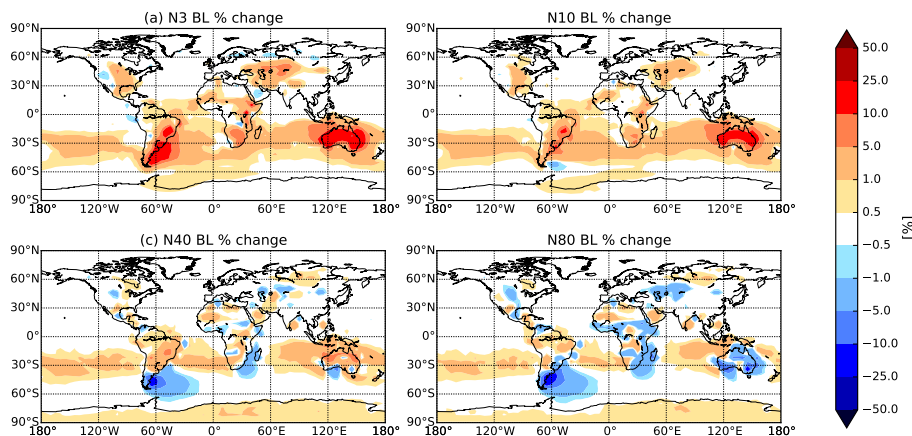
Figure 8. Percentage change in annually averaged boundary layer (a) N3, (b) N10, (c) N40 and (d) N80 when changing MEGAN BVOC emissions from year 1000 to year 2000 with constant present day anthropogenic emissions (2005) including an additional 100 \text{ Tg (SOA) yr}^{-1} as per D'Andrea et al. (2013) (BE2.XSOA–BE1.XSOA). Globally averaged, N3, N10 and N40 increased by 1.9, 1.2 and 0.3 % respectively, whereas N80 decreased by 0.3 % (see Table 2). An increase in particle number concentration is represented by red colors, and a decrease in blue.
