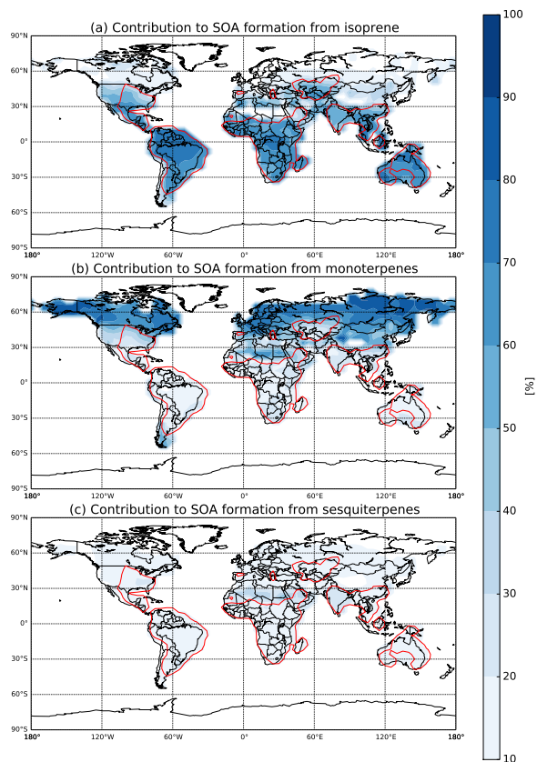
Figure 3. Percent contribution to SOA formation by (a) isoprene, (b) monoterpene and (c) sesquiterpene emissions from the MEGAN reconstruction, averaged over the years 1000–2000. The area enclosed by the red contour represents greater than 5% of the maximum mean millennial SOA formation from emissions of BVOCs (isoprene + monoterpenes + sesquiterpenes).
