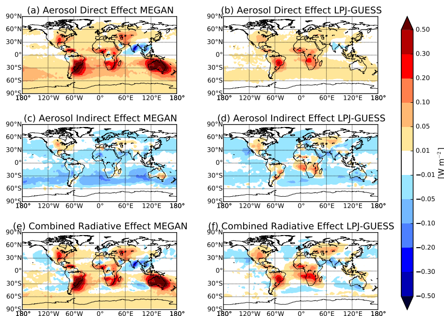
Figure 11. Annual mean change between year 1000 and year 2000 in (a) DRE with MEGAN BVOC emissions and anthropogenic emissions off ( \text{BE2.AEO.meg}-\text{BE1.AEO.meg} ), (b) DRE with LPJ-GUESS BVOC emissions and anthropogenic emissions off ( \text{BE2.AEO.LPJ}-\text{BE1.AEO.LPJ} ), (c) AIE with MEGAN BVOC emissions and anthropogenic emissions off, (d) AIE with LPJ-GUESS BVOC emissions and anthropogenic emissions off, (e) combined radiative effect with MEGAN BVOC emissions and anthropogenic emissions off, and (f) combined radiative effect with LPJ-GUESS BVOC emissions and anthropogenic emissions off. Global mean changes are +0.065 , +0.022 , -0.020 , -0.008 , +0.049 , and +0.015 \text{ W m}^{-2} respectively (see Table 3).
