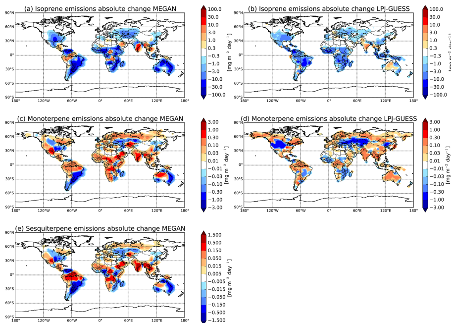
Figure 1. Absolute change in (a) isoprene, (c) monoterpene, and (e) sesquiterpene emissions between the years 1000–1010 and 1980–1990 in \text{mg m}^{-2} \text{day}^{-1} from the MEGAN terpenoid reconstruction and absolute change in (b) isoprene, and (d) monoterpene emissions between the years 1000 and 2000 in \text{mg m}^{-2} \text{day}^{-1} from the LPJ-GUESS terpenoid reconstruction (Acosta Navarro et al., 2014). Note the change of scale between panels. An increase in emissions is represented by red colors, and a decrease in isoprene emissions by blue.
