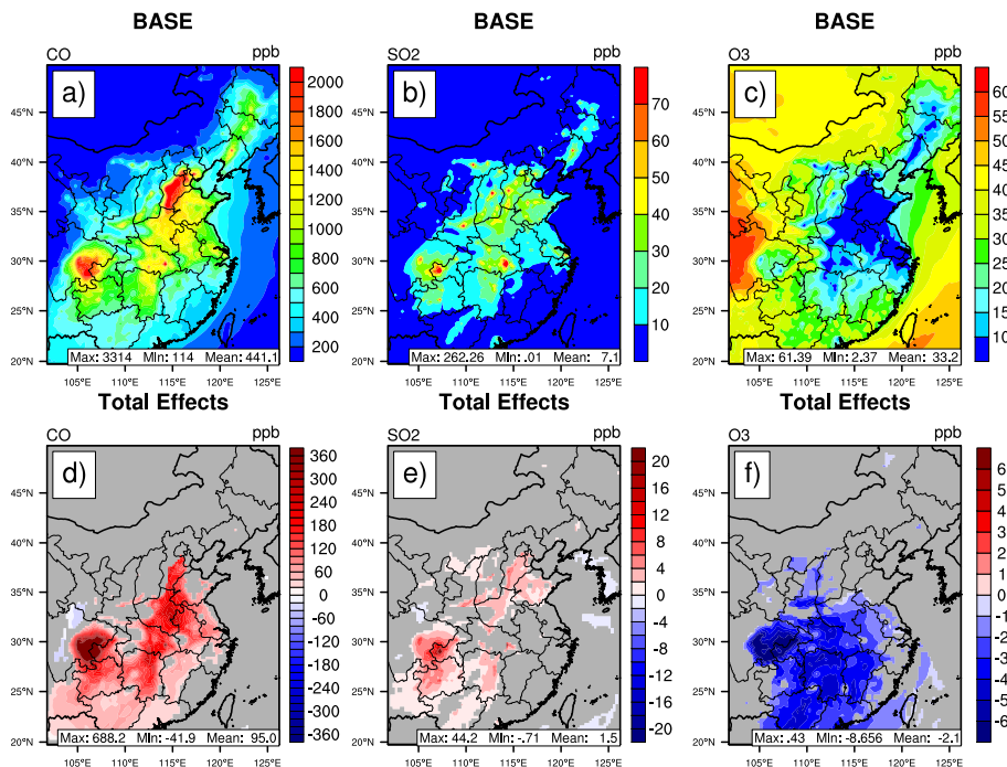
Figure 9. Simulated monthly mean CO, SO 2 , and O 3 mixing ratios and aerosol feedbacks (scenario BASE – EMP) on the three gas pollutants over eastern China in January 2013. Grey shaded areas indicate regions with less than 95 % significance.
