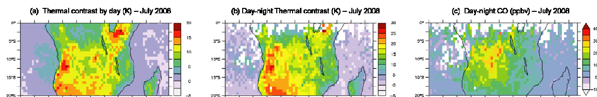
Figure S1. (top) Thermal contrast by day (in K), in July 2008 in southern Africa. (b) Day-night difference of the thermal contrast (in K), in July 2008 in southern Africa. (bottom). (c) Day-night difference of IASI CO (in ppbv).
