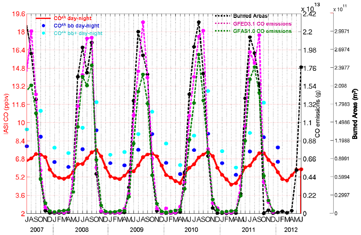
Figure B2. Evolution of the day-night difference of the integrated content qCO^{4A} (see text Sect. 4.1) on land, and of fires, between July 2007 and June 2012 in southern Africa. Red: day-night difference of qCO^{4A} . Blue dots: day-night difference of qCO^{4A} computed with a polluted CO profile as input in 4A. Black dashed: MODIS Burned Areas. Purple dashed: CO emissions from GFED3.1. Green dashed: CO emissions from GFAS1.0.
