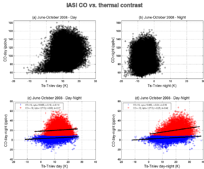
Figure B1. (a) IASI CO (in ppbv) by day as a function of the thermal contrast (in K), between June and October 2008, in southern Africa, on land. (b) Same as (a), by night. (c) Day-night difference of IASI CO (in ppbv) as a function of the thermal contrast by day (in K). (d) Same as (c) for the day-night difference of the thermal contrast.
