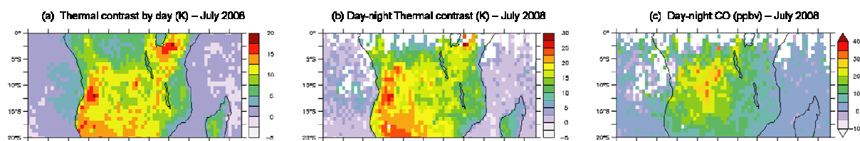
Figure S1. (a) Thermal contrast by day (in K), in July 2008 in southern Africa. (b) Day-night difference of the thermal contrast (in K). (c) Day-night difference of IASI CO (in ppbv).
