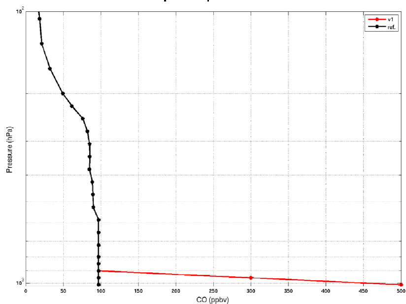
Figure S2. Black: reference profile of CO used as input in 4A for the retrieval of IASI CO (in ppbv). Red: a polluted profile in the boundary layer.
