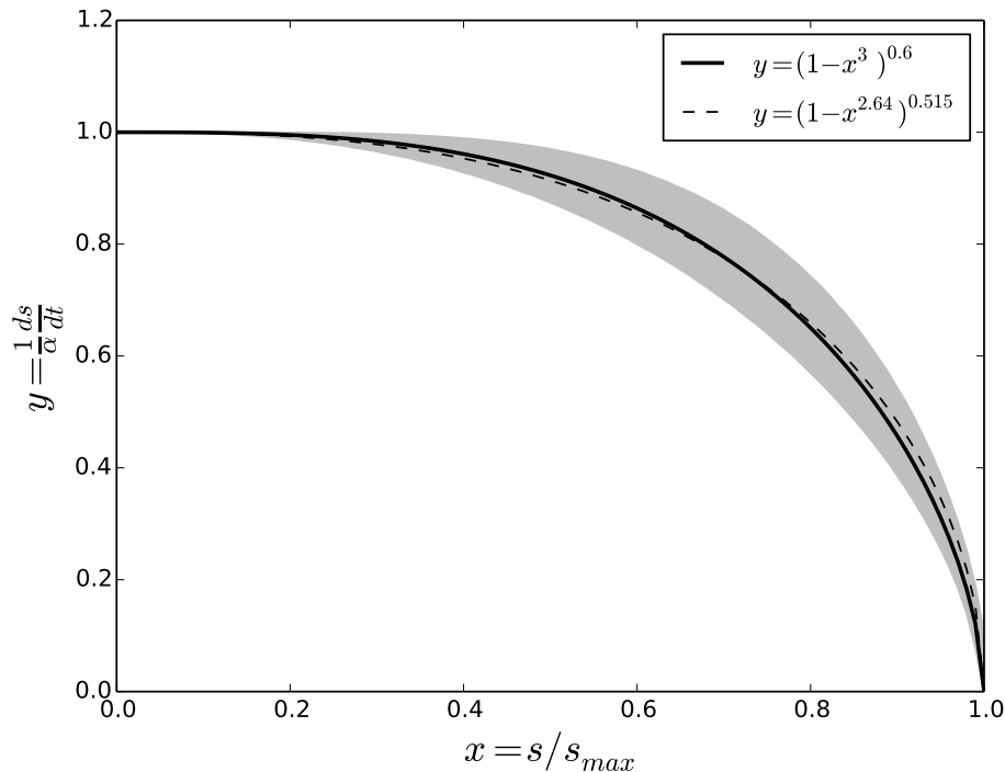
Figure 2. Scaled ds/dt as a function of s/s_{\max} evaluated from numerical solution of Eq. (1) using a range of updraft velocities and the various Whitby aerosol loadings. The solid line represents the parametrization (Eq. 16) with \mu = 3 and \lambda = 0.6 . The dashed line uses the coefficients determined in Appendix B.
