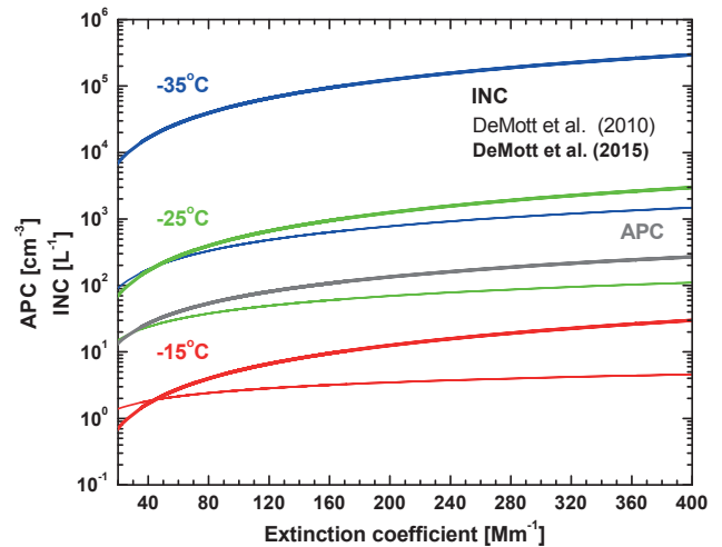
Fig. 5. Relationship between dust extinction coefficient and \text{APC}_{280} (grey line) after Eq. (1) and INC after Eq. (2) (thin lines) (DeMott et al., 2010) and Eq. (3) (thick lines) (DeMott et al., 2015) for temperatures of -15 , -25 , and -35^\circ\text{C} . The full range of dust extinction coefficients from 30 – 400 \text{ Mm}^{-1} measured on 29 September 2011 (Fig. 1) is shown.
