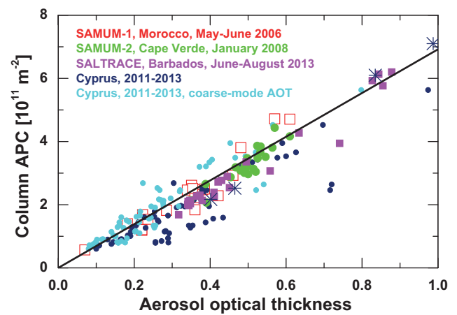
Fig. 2. Correlation between aerosol optical thickness (500 nm AOT) and column-integrated aerosol particle number concentration (column APC_{280} ) considering particles with r > 280 nm. Desert-dust-dominated observations from several field campaigns (SAMUM-1, large red open squares, SAMUM-2, green circles, SALTRACE, small pink squares) and from long-term observations at Limassol from 2011–2013 are considered. For Cyprus, coarse-mode (light blue circles) and total (fine + coarse-mode, deep blue circles) AOTs are correlated with column APC_{280} . In the case of the stars (4 Cyprus observations with total AOT from 1.6–4), AOT and column APC values are divided by 4. Least squares fitting to all shown data (except the dark blue Cyprus values) yield the black solid line with the slope of 6.85 \times 10^{11} \text{ m}^{-2} .
