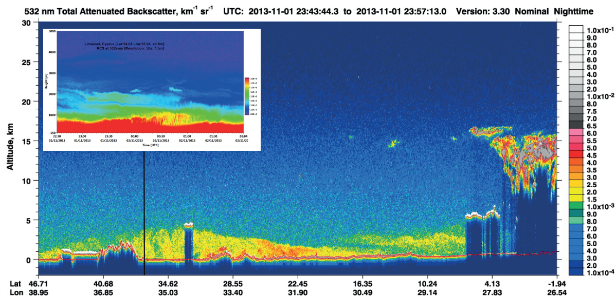
Fig. 11. CALIOP measurement (height versus latitude/longitude display) of the attenuated 532 nm particle backscatter coefficient during an overpass 180 km to the east of Limassol on 1 November 2013, 23:43–23:57 UTC. Desert dust layers are given in green to yellow colors and reach up to about 4 km height. The inserted height-time display shows the CUT lidar observation of the cross-polarized range-corrected 532 nm backscatter signal up to 5 km height on 1 November 2013, 22:30 to 2 November 2013, 02:04 UTC. The vertical black line indicates the closest position of CALIOP (laser foot print) to the ground-based CUT lidar at Limassol, Cyprus.
