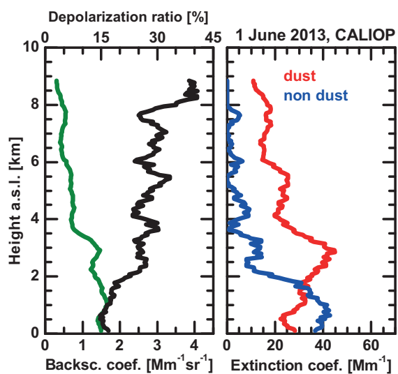
Fig. 9. CALIOP data analysis products based on the 135 signal profile averages shown in Fig. 8: (Left) Vertical profiles of 532 nm particle backscatter coefficient (green) and particle linear depolarization ratio (black), and (right) derived particle extinction coefficients for non-dust (blue) and desert dust particles (red). The particle backscatter coefficients (left, green) are taken from the CALIOP data base and smoothed with 600 m gliding window length. The particle linear depolarization ratio is computed from the cross-polarized and total backscatter coefficient profiles after smoothing the profiles with 600 m vertical window length. Lidar ratios used in the backscatter-to-extinction conversion are 50 sr for the non-dust particles and 55 sr for Saharan dust.
