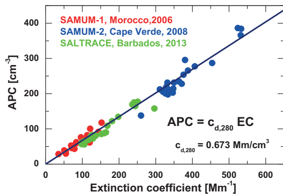
Fig. 4. Relationship between dust layer mean 500 \text{ nm} extinction coefficient (EC) and dust layer mean \text{APC}_{280} for observations taken during three desert dust field campaigns at Morocco, Cape Verde, and Barbados. The linear regression yields c_{d,280} = 0.673 \pm 0.07 \text{ Mm cm}^{-3} . The correlation coefficient is 0.915 . c_{d,280} is used in Eq. (1).
