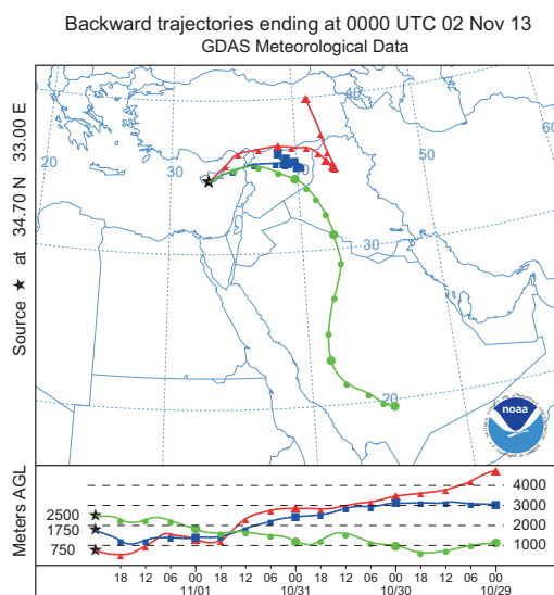
Fig. 12. HYSPLIT 4 day backward trajectories arriving within the dust layer over Limassol, Cyprus, at 750 (red), 1750 (blue), and 2500 m height (green) on 2 November 2013, 00:00 UTC.
