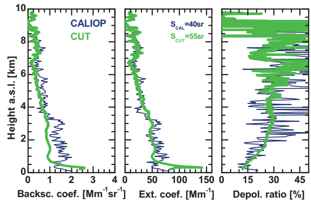
Fig. 8. Comparison of profiles of particle backscatter coefficient, extinction coefficient, and particle linear depolarization ratio measured with ground-based CUT lidar at Limassol (thick green curves, 60 min means) on 1 June 22:28–23:28 UTC, and with spaceborne CALIOP (black noisy curves, 45 km east of Limassol, during seconds 38–43 of 23:53 UTC). In the case of CALIOP, 135 signal profiles are averaged (nine level-2 aerosol profiles, 45 km horizontal resolution). No vertical smoothing is applied to the CALIOP data. CUT lidar signal profiles were vertically smoothed by 180 m. A lidar ratio of S_{CAL} = 40 sr was selected in the retrieval of CALIOP data and of S_{CUT} = 55 sr (optimum lidar ratio for this Saharan dust case after Mamouri et al. (2013)) was applied in the CUT computation of backscatter and extinction profiles.
