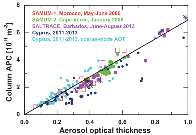
Fig. 2. Correlation between aerosol optical thickness (500 nm AOT) and column-integrated aerosol particle number concentration (column \text{APC}_{280} ) considering particles with r > 280 nm. Desert-dust-dominated observations from several field campaigns (SAMUM-1, large red open squares, SAMUM-2, green circles, SALTRACE, small pink squares) and from long-term observations at Limassol from 2011-2013 are considered. For Cyprus, coarse-mode (light blue circles) and total (fine + coarse-mode, deep blue circles) AOTs are correlated with column \text{APC}_{280} . In the case of the stars (4 Cyprus observations with total AOT from 1.6–4), AOT and column APC values are divided by 4. Least squares fitting to all shown data (except the dark blue Cyprus values) yield the black solid line with the slope of 6.85 \times 10^{11} \text{ m}^{-2} .
