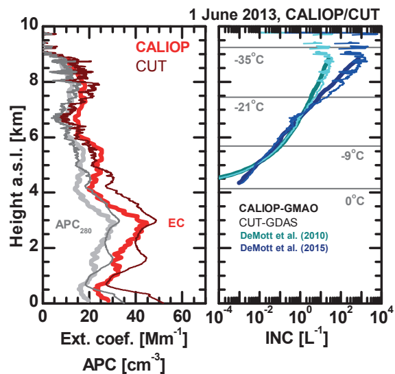
Fig. 10. Profiles of 532 nm desert dust extinction coefficient \sigma_d , APC_{280} , and INC. GDAS (Global Data Assimilation System) profiles of temperature and pressure for the Limassol region were used in the CUT lidar data analysis (thin lines) and GMAO (Global Modeling and Assimilation Office) Data Assimilation System profiles of the meteorological parameters along the CALIOP flight track were used in the analysis of the space lidar observations (thick lines). INC profiles computed with Eq. (2) (DeMott et al., 2010) are shown as green lines (CALIOP, thick, CUT lidar, thin). INC profiles computed with Eq. (3) (DeMott et al., 2015) are shown as blue lines (CALIOP, thick, CUT lidar, thin). Grey horizontal lines indicate the temperature ranges for which the parameterizations are explicitly valid ( -9 to -35 °C, Eq. (2), -21 to -35 °C, Eq. (3)). Uncertainties are of the order of 20% (for \sigma_d ), 30% (for APC_{280} ), and within a factor of 3 (in the case of INC) when using the dust INC parameterization after DeMott et al. (2015).
