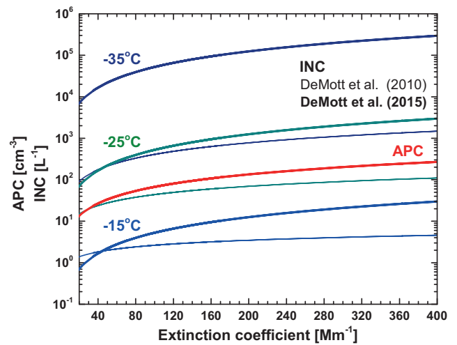
Fig. 5. Relationship between dust extinction coefficient and \text{APC}_{280} (red line) after Eq. (1) and INC after Eq. (2) (thin lines) (DeMott et al., 2010) and Eq. (3) (thick lines) (DeMott et al., 2015) for temperatures of -15 , -25 , and -35^\circ\text{C} . The full range of dust extinction coefficients from 30 – 400 \text{ Mm}^{-1} measured on 29 September 2011 (Fig. 1) is shown.
