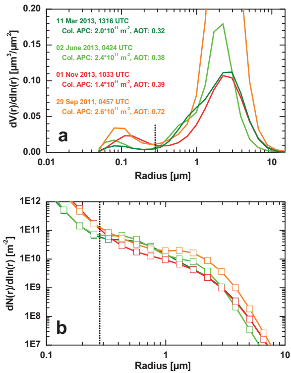
Fig. 3. Column-integrated particle volume size distribution (a) and respective particle number size distribution (b) derived from AERONET sun/sky photometer observations at Limassol, Cyprus. Two Saharan dust cases (11 March 2013, olive, 2 June 2013, green) and two Middle East desert dust cases (29 September 2011, orange, 1 November 2013, red) are shown. The dotted vertical lines at 0.28 \mu\text{m} indicate the lower limit of the particle radius range considered in the calculation of column \text{APC}_{280} , which is defined as the sum of all particles larger than 280 \text{ nm} in radius. The column \text{APC}_{280} values for the four measurement cases are given as numbers together with 500 \text{ nm} total AOT in the upper panel a.
