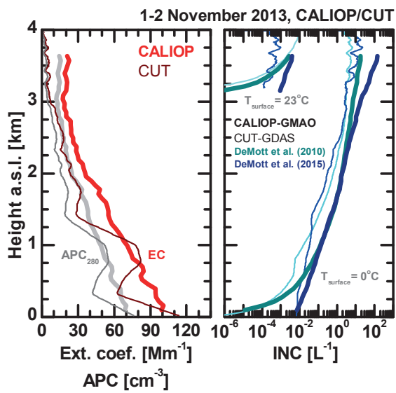
Fig. 13. Same as Fig. 10, except for a Middle East desert dust outbreak on 1–2 November 2013. In the case of CALIOP profiles (180 km east of Limassol), again 135 signal profiles (45 km horizontal resolution) are averaged, collected during seconds 8–14 of 23:47 UTC on 1 November 2013. The CUT lidar profiles show average values for the time period from 00:00–00:59 UTC on 2 November 2013. The original GDAS and GMAO temperature and pressure profiles were used in the computation of the INC profiles indicated by T_{\text{surface}} = 23^{\circ}\text{C} . The GDAS and GMAO temperature profiles were shifted by 22 K (Limassol) and 23 K (CALIOP) in the case of the INC curves indicated by T_{\text{surface}} = 0^{\circ}\text{C} . Uncertainties are of the order of 20% (for \sigma_d ), 30% (for \text{APC}_{280} ), and within a factor of 3 (for INC) when using the dust INC parameterization after DeMott et al. (2015).
