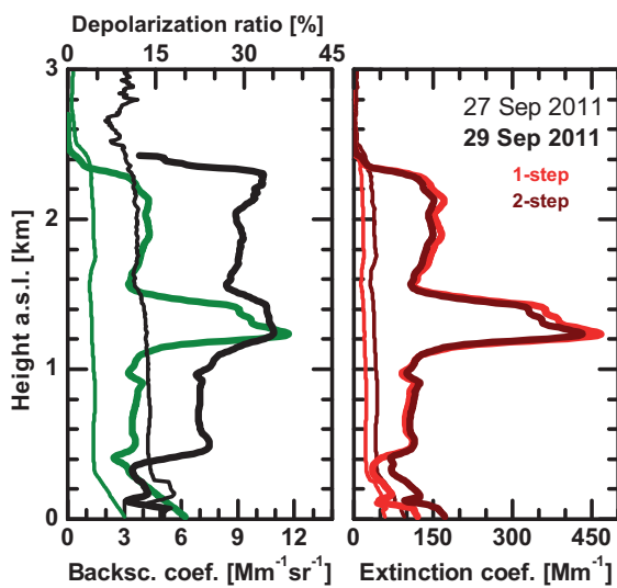
Fig. 1. (Left) 532 nm particle backscatter coefficient (green) and particle linear depolarization ratio (black) as a function of height above sea level (a.s.l.) and (right) dust extinction coefficients computed by means of the 1-step and 2-step methods (Mamouri and Ansmann, 2014). A major dust outbreak from the Middle East deserts was observed with the CUT lidar at Limassol, Cyprus, on 29 September 2011, whereas fine-mode soil dust, probably injected during biomass burning events in Turkey, was observed on 27 September 2011. The data analysis is explained in detail by Mamouri and Ansmann (2014). figure
