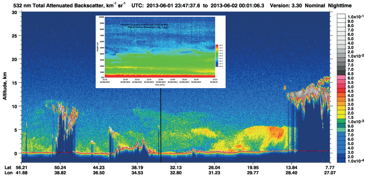
Fig. 6. CALIOP measurement (height versus latitude/longitude display) of the attenuated 532 nm particle backscatter coefficient during an overpass 45 km to the east of Limassol on 1 June 2013, 23:47 UTC, to 2 June 2013, 00:01 UTC. Desert dust layers are given in green to yellow colors and reach up to 4–10 km height. The inserted height-time display shows the CUT lidar observation of the range-corrected cross-polarized 532 nm backscatter lidar signal on 1 June 2013, 21:33–23:53 UTC (height range from 250–10000 m a.s.l.). Dust (green, yellow, and light blue layers) is observed up to 9–10 km height. The vertical black line indicates the closest position of CALIOP (laser footprint) to the ground-based CUT lidar at Limassol, Cyprus.
