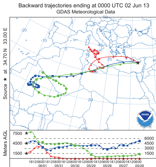
Fig. 7. HYSPLIT 7-day backward trajectories arriving within the dust layer over Limassol, Cyprus, at 1500 (red), 4500 (blue), and 7500 m height (green) on 2 June 2013, 00:00 UTC.
