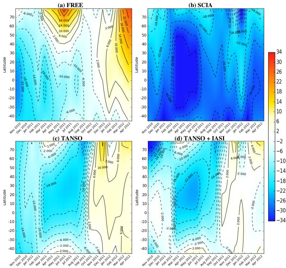
Fig. 11. Time series of the monthly average smooth x\text{CH}_4 difference (in ppb) between the experiments and the measurements from the TCCON network: (a) FREE, (b) SCIA, (c) TANSO and (d) TANSO + IASI experiments.
