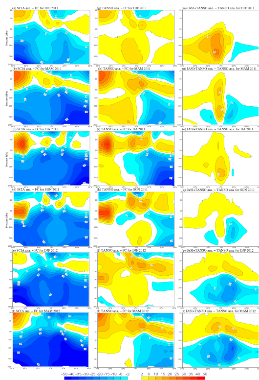
Fig. 8. Seasonal and zonal mean difference between the CH 4 mole fraction (in ppb): from the SCIA experiment and the FREE free run (left); from the TANSO experiment and the FREE free run (middle); from the IASI+TANSO experiment and the TANSO experiment (right). The seasonal means are from top to bottom row: DJF 2010/2011, MAM 2011, JJA 2011 and SON 2011, DJF 2011/2012 and MAM 2012.
