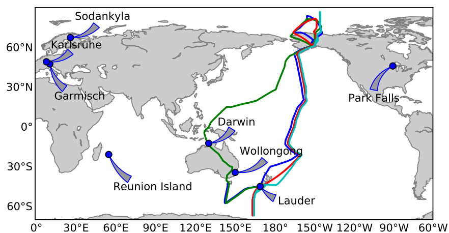
Fig. 4. Location of few TCCON stations used in this paper (blue points) and trajectories of the 2011 HIPPO campaigns. The campaign periods are respectively: 16 June–29 June (blue), 28 June–11 July (green), 19 August–30 August (red), 29 August–09 September (cyan). Note that for the plot, some trajectories are shifted one or two degrees east or west in order to avoid superposition between them.
