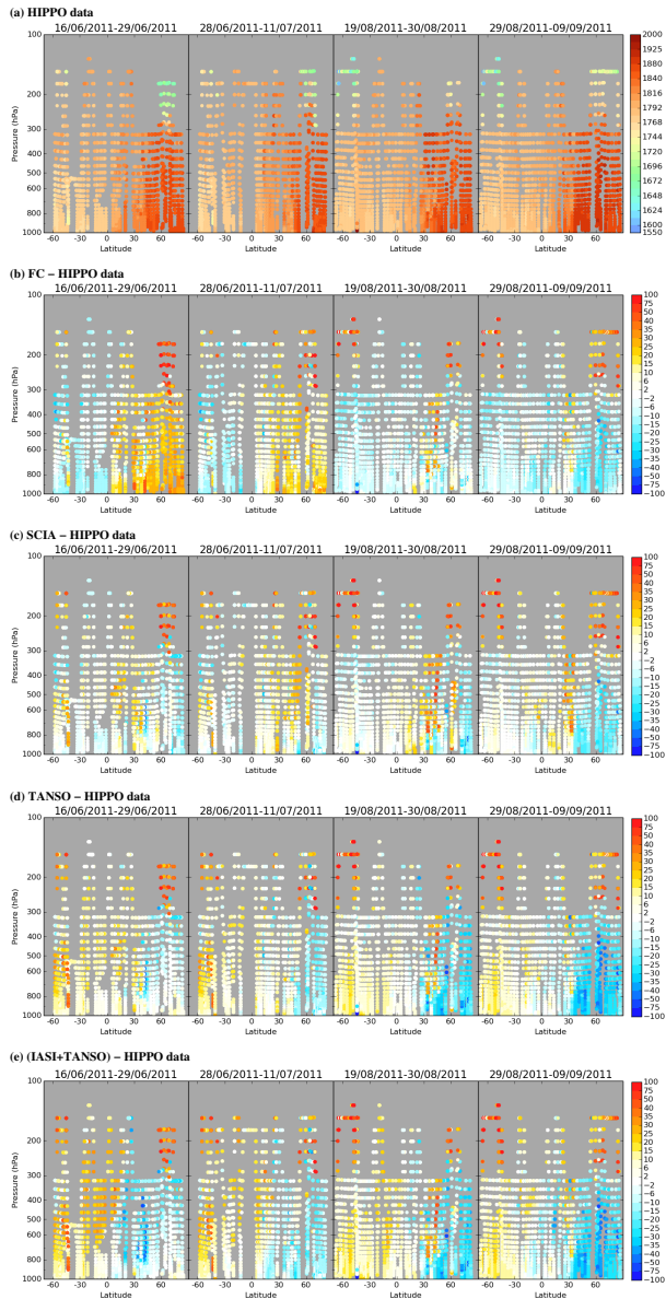
Fig. 9. Top row (a): HIPPO CH 4 data (latitude vs. pressure, in ppb) for the four campaigns (from the leftmost panel for the first campaign to rightmost panel for the last campaign). The beginning and end dates of each campaign is detailed on top of each panel. From row 2 to 5: difference between the experiments and the HIPPO data (in ppb): (b) FREE minus HIPPO, (c) SCIA analysis minus HIPPO, (d) TANSO (v.1) analysis minus HIPPO and (e) TANSO+IASI analysis minus HIPPO. A global bias has been removed from the FRRE run and from each analysis (see Table 1). The grey shade means there is no observation.
