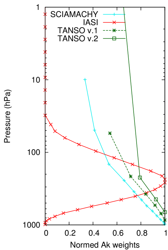
Fig. 3. Example of averaging kernels (cyan: SCIAMACHY, dotted green: TANSO v.1 and full green: TANSO v.2.0) and weighting function normalised by its maximum value (red: IASI) of the CH 4 products from the different instruments.
