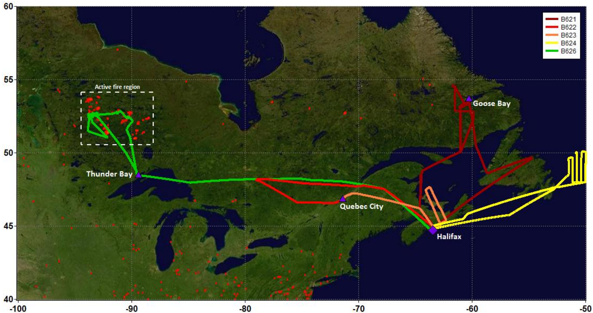
Figure S1: Flight tracks for flights B621-624 and B626 during BORTAS, overlain on a MODIS accumulated 10 day fire map for eastern Canada during the period 20/07/2011 – 29/07/2011. Images courtesy of MODIS Rapid Response Project at NASA/GSFC.
