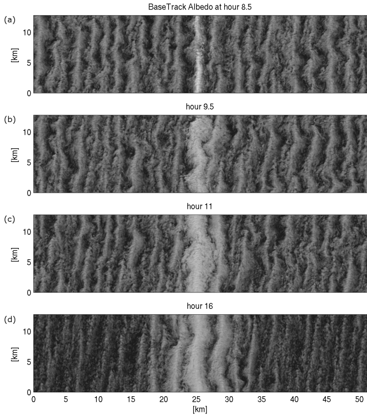
Fig. 6. x - y snapshots of albedo for run BaseTrack at hours (a) 8.5 (half an hour after track injection), (b) 9.5, (c) 11, and (d) 16.
