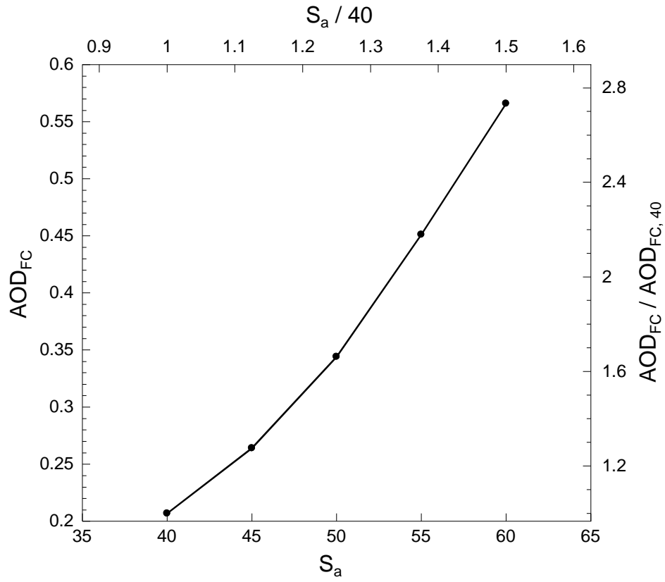
Figure 14. Mean AOD_{FC} as a function of S_a derived from the full column retrievals shown in Fig. 12.
