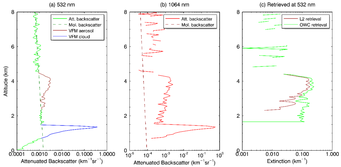
Figure 5. Solid curves in panel (a) and (b) show CALIOP attenuated backscatter profiles corrected for attenuation of molecular scattering and ozone absorption 532 nm (a) and 1064 nm (b). The dashed lines in these panels show the corresponding molecular backscatter profiles. Panel (c) shows the aerosol extinction profiles at 532 nm obtained from the standard L2 profile products (brown line) and retrieved in this paper using the OWC constrained technique (light green line). In both cases the retrievals were applied to a sequence of 5-km averaged L1 profiles, which in turn were averaged further for 4 consecutive 5-km profiles around 10°S, as shown in Figure 4. Brown and blue coloring in panel (a) indicate the data segments detected as aerosol and cloud in the standard L2 data processing.
