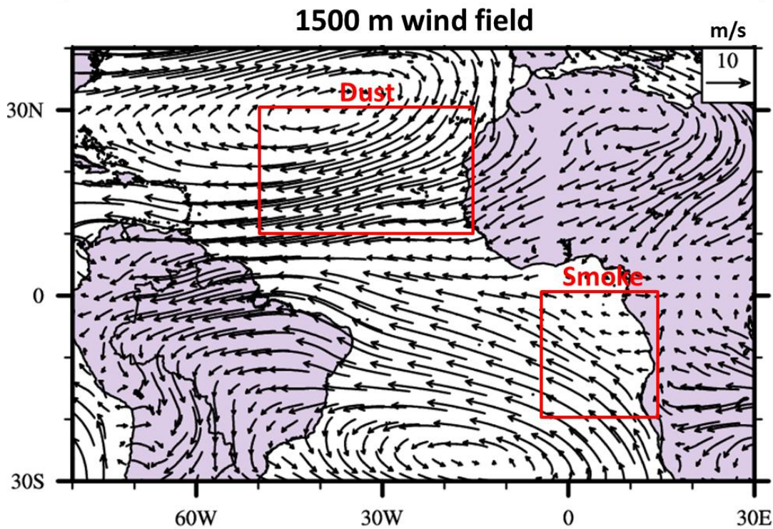
1 2 Figure 1. Spatial domains analyzed (red boxes) and wind fields (arrows) from ECMWF data for 3 July and August from 2007 to 2012. The northern region (10°N-30°N, 50°W-15°W) is along the 4 Saharan dust transport pathway over the tropical North Atlantic, while the southern region (20°S- 5 0°, 5°W-15°E) is along the smoke transport pathway over the tropical South Atlantic.
