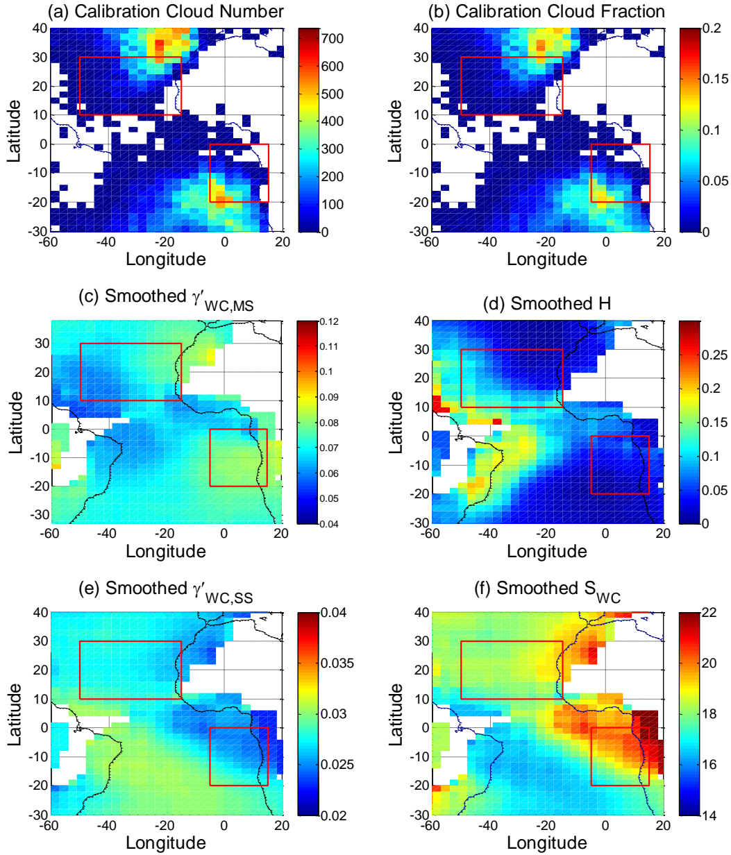
Figure 3. Spatial distributions of (a) number of calibration opaque water clouds above which no other cloud or aerosol layer was detected, (b) the fraction of calibration clouds relative to the total samples in each grid, (c) smoothed mean integrated attenuated backscatter, \gamma'_{WC,MS,NA} = \int_{C_{base}}^{C_{top}} B'(r) dr , from opaque water clouds in (a), (d) H calculated using Eq. (4), (e) mean integrated attenuated single-scattering backscatter, \gamma'_{WC,SS,NA} = \gamma'_{WC,MS,NA} H , calculated from (c) and (d) and used as a reference in each grid box, and (f) water cloud lidar ratio S_{WC} = 1/2\gamma'_{WC,SS,NA} (i.e., Eq.(5)) calculated from (e). The grid box size is 2^\circ \times 3^\circ (lat \times lon). The smoothing window is a 5^\circ \times 5^\circ grid. The white color represents the grids having no data samples. Data is from all nighttime CALIOP measurements during June – August in the years 2007 – 2012.
