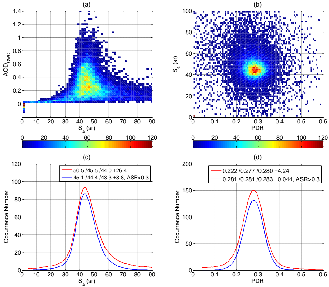
Figure 8. Analysis results for the dust transport region as indicated by the red box in Figure 6. The upper row shows 2-D distributions of (a) OWC AOD vs. S_a retrieved using OWC AOD as a constraint, (b) S_a vs. PDR, while the lower row shows histograms of (c) S_a and (d) PDR occurrence frequencies. The S_a distribution in (c) has a bin size of 0.1 sr and is smoothed, while the bin size for S_a in (a) and (b) is 1.5 sr. The PDR distribution in (c) has a bin size of 0.001 and is smoothed, while the bin size in (b) is 0.006. The red curves in (c) and (d) include all data and the blue curves are screened data using ASR > 0.3. The numbers in the legends of are mean/median/mode \pm standard deviation of S_a (c) and PDR (d).
