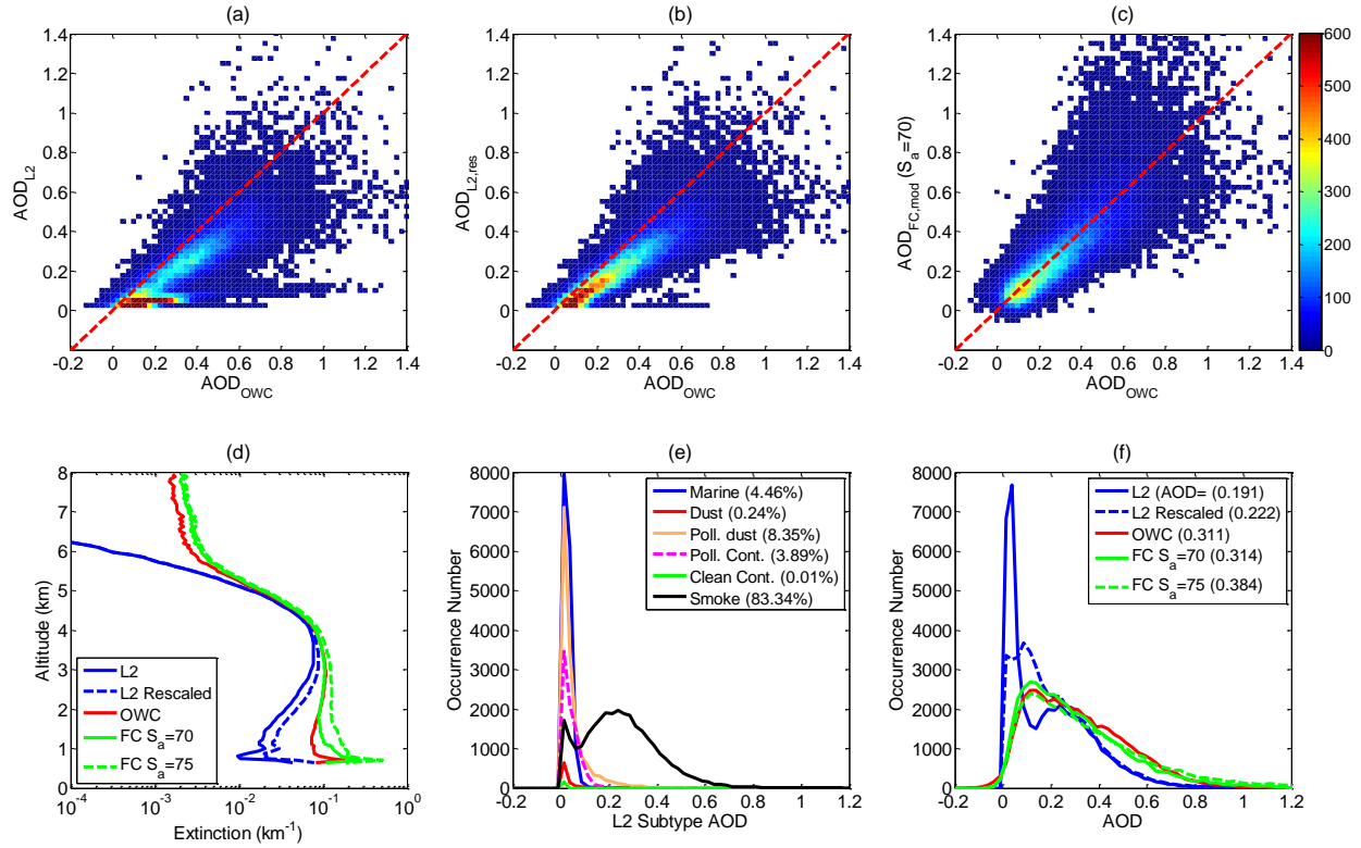
3 Figure 12. Analysis results for the smoke transport region as indicated by the red box in Figure 7. 4 The top row shows two dimensional distributions of (a) AOD_{L2} vs. AOD_{OWC} , (b) AOD_{L2, res} vs. 5 AOD_{OWC} , and (c) AOD_{FC, mod} vs. AOD_{OWC} for S_a = 70 sr. full column AOD using modeled dust 6 S_a = 40 sr vs. AOD_{OWC} . The bottom row shows (d) extinction profiles and histograms of occurrence 7 number, (e) L2 AOD of different aerosol types, and (f) AOD retrieved using different retrieval 8 methods. The bin size for AOD is 0.025.
