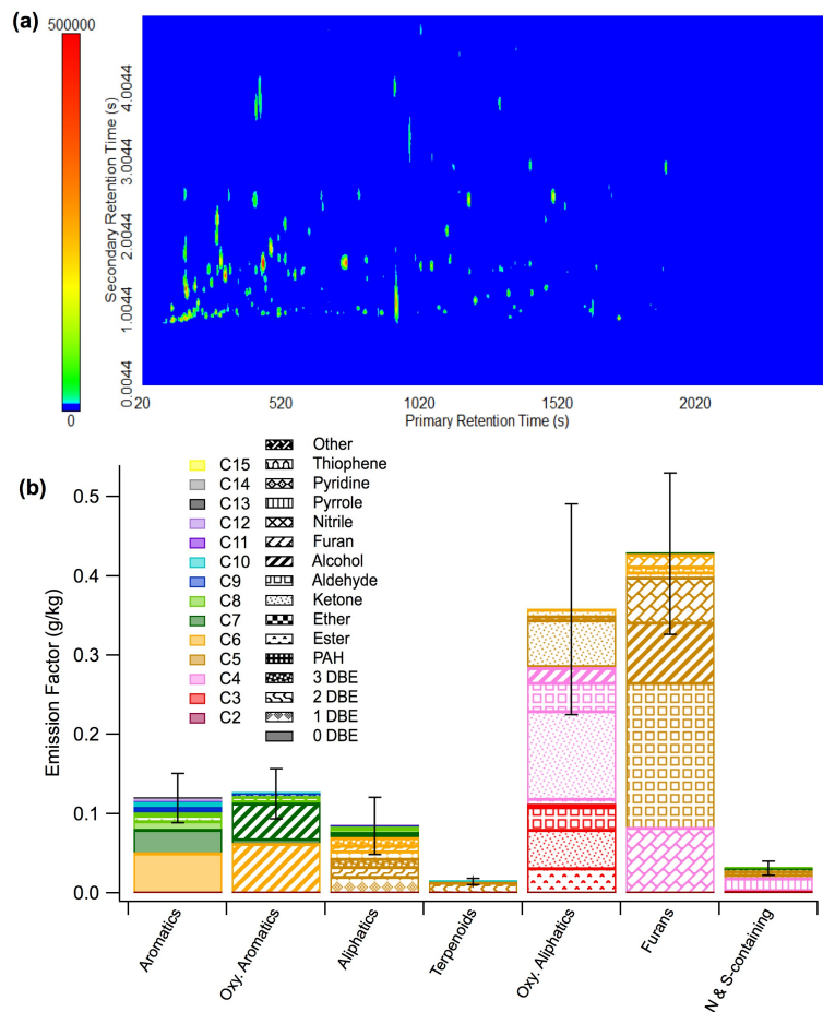
Figure 4. As in Fig. 1, for a wiregrass fire.
