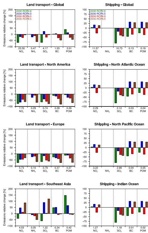
Figure 2. Relative changes in the emissions from land transport (left) and shipping (right) in the year 2030 with respect to 2000, for the four RCP scenarios. The changes are calculated globally (upper row) and for the regions defined in Fig. 1 (lower three rows). Total emissions for the year 2000 are shown at the bottom of each panel, in units of Tg(species) a -1 and Tg(NO x ) a -1 for NO x . Note the different vertical scales for the two sectors.
