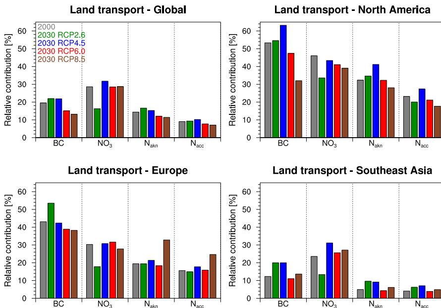
Figure 6. Relative contributions of land transport to the average mass and number burdens of selected aerosol species and different particles size modes (Aitken and accumulation mode), respectively. Results are shown for the year 2000 and for the four RCP scenarios in 2030. The values are integrated over the continents and in the two lowermost model layers ( \sim 0\text{--}230 m). For the definition of the different regions see Fig. 1.
