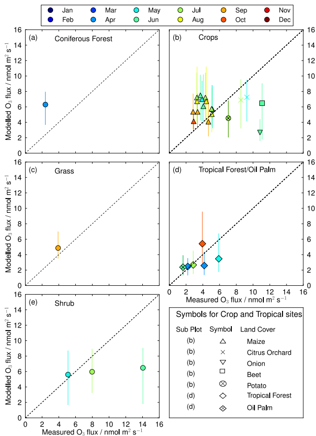
Figure 11. Measured and modelled monthly average O_3 dry deposition fluxes at short-term measurement sites. Colours indicated the average flux for relevant month and shapes indicate the measurement sites.
