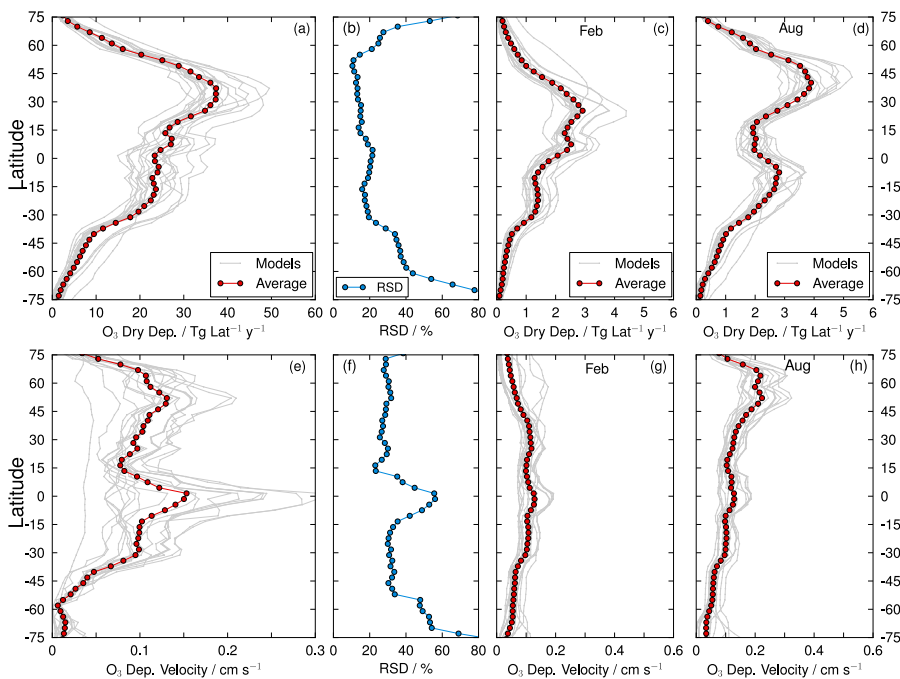
Figure 2. Latitudinal distribution of total O_3 dry deposition (top row) and average O_3 deposition velocities (bottom row) per 3^\circ latitude band for the model ensemble. Panels show the total annual O_3 dry deposition and average annual O_3 dry deposition velocity ( a , e ), the relative standard deviation (RSD) in annual deposition and average annual deposition velocity across the models ( b , f ), and the total monthly O_3 dry deposition fluxes and average annual dry deposition velocities in February ( c , g ) and August ( d , h ).
