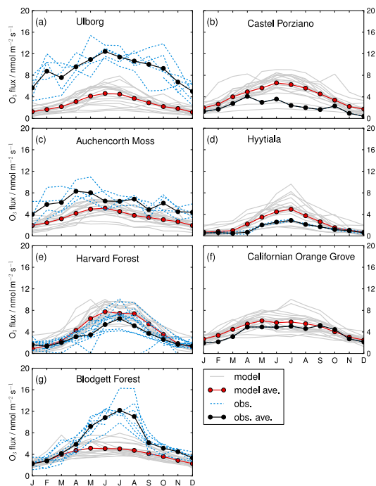
Figure 8. Measured and modelled monthly average O_3 dry deposition fluxes at Ulborg (a) , Castel Porziano (b) , Auchencorth Moss (c) , Hyytiala (d) , Harvard Forest (e) , Californian orange grove (f) , and Blodgett Forest (g) . Grey lines show results from individual models and blue lines show observations different years.
