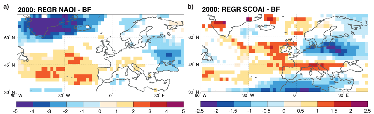
Fig. 4: Blocking frequency anomalies (in % of days in which a blocking event occur at a given grid box) per unit of NAOI (NAOI, a) and SCOAI (SCOAI, b) standard deviation. The anomalies are calculated using a one-point regression analysis (see Appendix B). Only differences significant at the 95% confidence level are shown (based on the correlation significance between NAOI/SCOAI and blocking frequency). Note that the two panels use different colour-scales.
