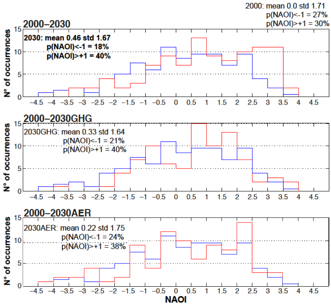
Fig. 2: Frequency distributions of the winter (DJF) NAOI for the 2000 control simulation (blue, all panels), 2030 (red, upper panel), 2030GHG (red, central panel) and 2030AER (red, lower panel). Numbers show the NAOI mean value, the standard deviation (std) and the probability of having a NAOI greater than +1 ( p(\text{NAOI}) > +1 ) or smaller than -1 ( p(\text{NAOI}) < -1 ). Values of the simulations having a NAOI mean significantly different from 2000 control mean at 95% confidence level are shown in bold. The 2000s mean NAO is by definition equal to 0 and the number of occurrences has been normalized to 30 years for a direct comparison with the other simulations.
