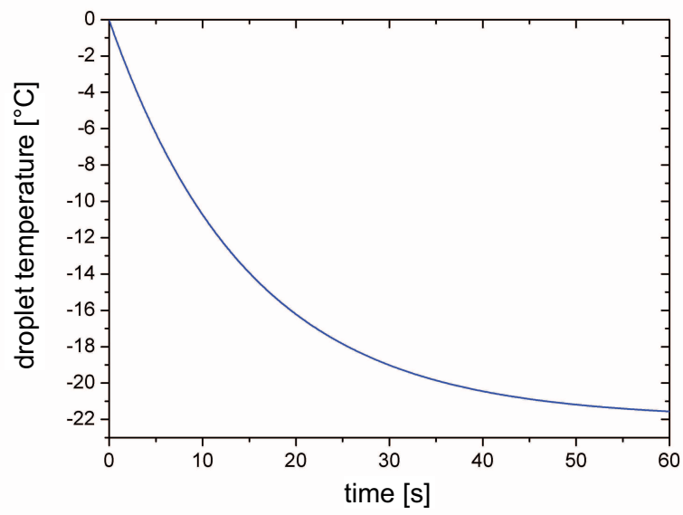
Fig. 13. Development of droplet temperature during cooling in the AL.
