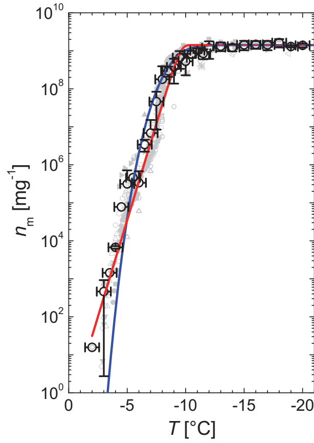
Fig. 12. Average n_m values (black circles) overlying all separate data points which were included in the average (shown as background in light grey), together with fits obtained from a time-independent variant of the parameterization given in Hartmann et al. (2013) (red curve, see Eq. 6 ) and in Niedermeier et al. (2014) (blue curve).
