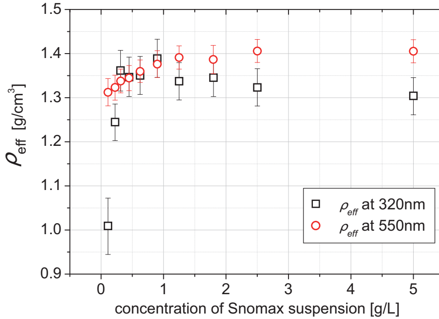
Fig. 3. The effective density of Snomax measured for particles generated from differently concentrated suspensions for two different dry particle sizes.
