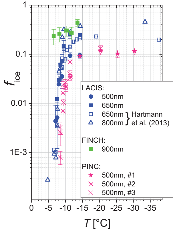
Fig. 7. Frozen fractions as a function of temperature measured with FINCH, LACIS and PINC for different dry particle sizes. Open symbols given for LACIS represent the data published in Hartmann et al. (2013). PINC data labeled with #1 were taken during a campaign at LACIS, #2 and #3 denote data taken at ETH using the INUIT snomax sample and a different Snomax sample, respectively. For more details on the different data sets see Sect. A7.
