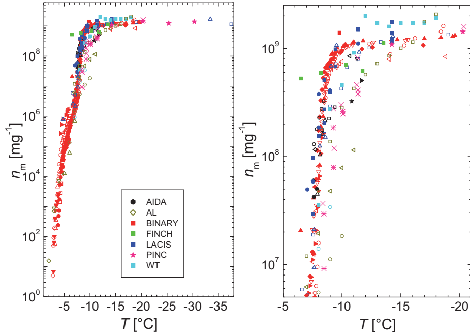
Fig. 11. Number of INM per dry Snomax mass as a function of temperature, derived from measured f_{\text{ice}} of all instruments, i.e. for all data shown in Figs. 5 to 8. BINARY data are solely displayed in red, but otherwise the same symbols and color codes are used as in Figs. 5 to 8, i.e. in all cases data from one instrument are always displayed in a single color. The right panel is similar to the left, zooming in on values for 5 \times 10^6 \text{ mg}^{-1} < n_m < 2.5 \times 10^9 \text{ mg}^{-1} and on temperatures < -21 \text{ }^\circ\text{C} .
