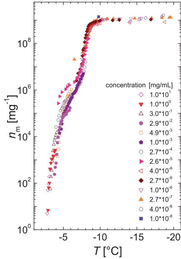
Fig. 10. BINARY data represented as number of INM per dry Snomax mass, n_m , as a function of temperature, for all data shown in Fig. 5 and using identical symbols.
