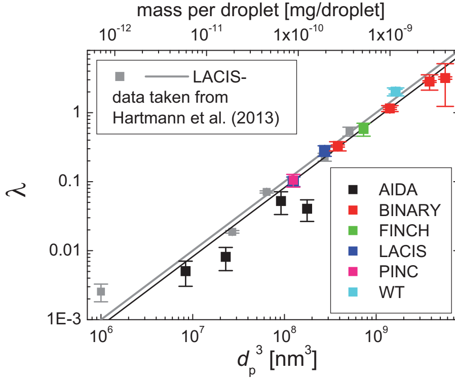
Fig. 9. Average number of INM per particle or droplet as a function of the third power of particle diameter or mass per droplet, respectively, for data sets that showed a clear plateau with f_{ice}^* < 1 . Grey symbols represent data published in Hartmann et al. (2013). The grey line is the corresponding fit function derived in Hartmann et al. (2013), which also describes the data collected in the present study well. The black line represents a fit obtained for this study (for details see text).
