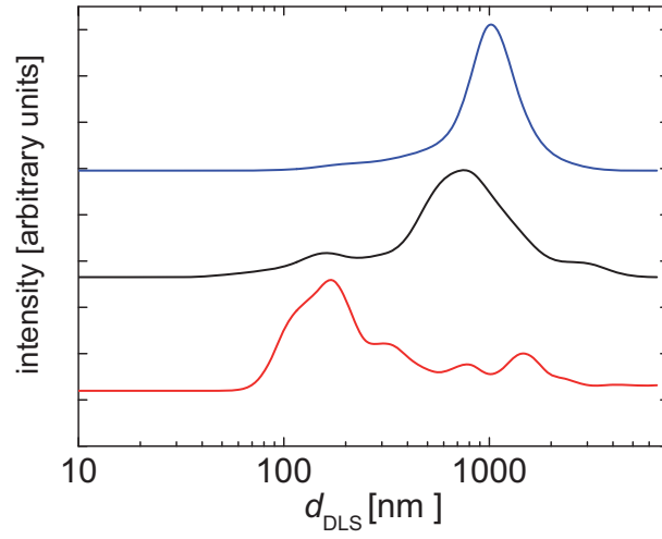
Fig. 4. Size distributions of the particulate matter present in Snomax suspensions as measured with DLS. The blue curve represents the size distribution seen in a freshly produced Snomax suspension, the black and red curve show size distributions as present in particles after dispersion with a nozzle spray disperser or an atomizer, respectively.
