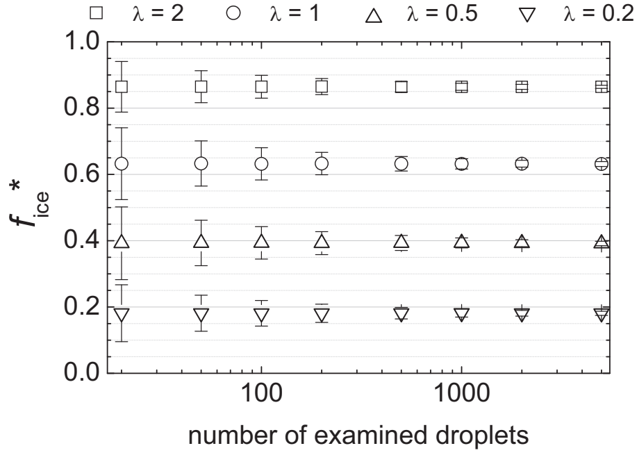
Fig. 2. Average f_{ice}^* and the respective standard deviation for different numbers of examined droplets and for different values of \lambda , obtained by theoretical considerations.
