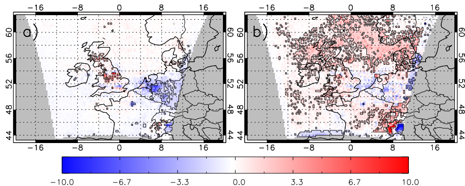
Figure 5. Mean bias in tropospheric NO 2 column ( \times 10^{15} molecules cm -2 ), 2006, between AQUAM Run C (AKs applied) and OMI for (a) summer (RMSE = 3.68 \times 10^{15} molecules cm -2 and FGE = 0.65) and (b) winter (RMSE = 5.12 \times 10^{15} molecules cm -2 and FGE = 0.63). The RMSE and FGE are over the UK between 8° W–2° E and 50–60° N and black polygoned regions show significant differences. Also the same for mean bias plots in Figs. 6–9.
