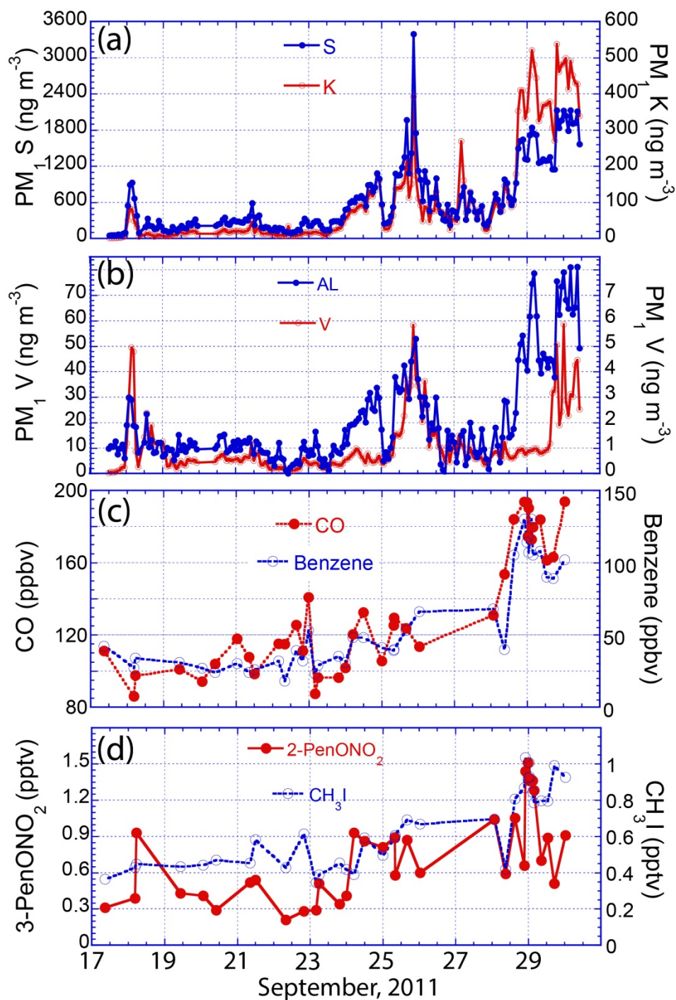
Figure 12. Time series of (key elements and gases. (a) & (b) DRUM time series of Sulfur + Potassium & Aluminum + Vanadium, respectively. (c) Carbon Monoxide and Benzene, both common biomass burning emissions. (d) 2-Pentane Oxyl Nitrate, a photochemical pentane daughter product and Methyl-Iodide, a halogenated organic specie also emitted by burning, the oceans, and used in agriculture.
