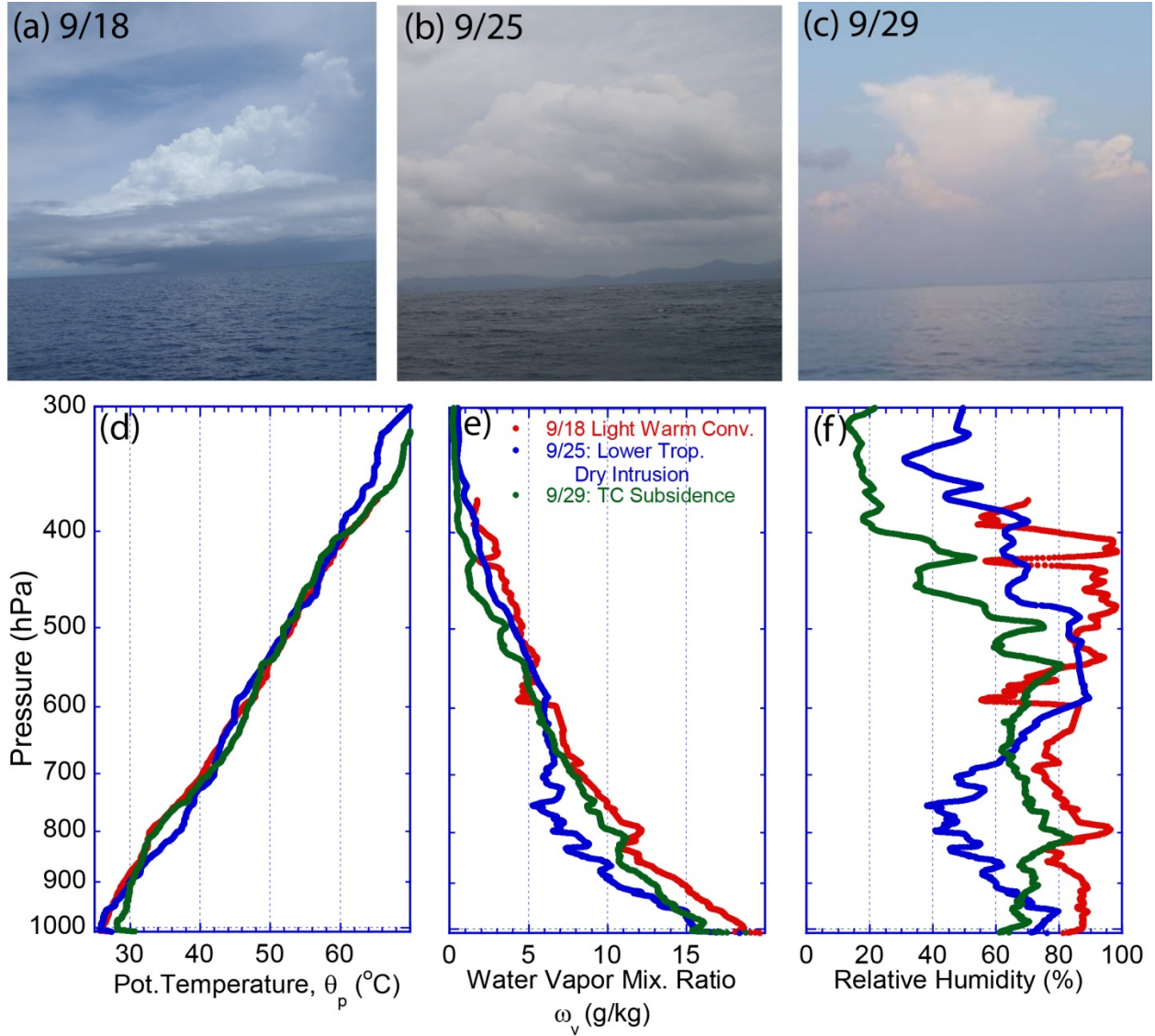
Figure 8. Photographs and corresponding sounding elements for three aerosol regimes during periods of marginal convection. a) Sept. 18 th at Apo reef with isolated warm convection in moderately moist conditions; (b) Sept 25 th at El Nido with warm non precipitating convection with a lower troposphere dry intrusion during the height of the pollution event; (c) Sept. 29 th at the Northern Sulu Sea with isolated deep convection in overall TC induced subsidence during height of biomass burning event. (d), (e) and (f) Corresponding Vasco released radiosonde profiles of potential temperature, water vapor mixing ratio, and relative humidity, respectively.
