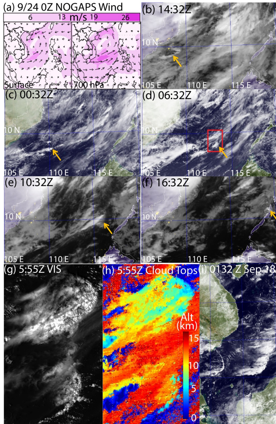
Figure 11. Day visible and night infrared time series of September 24 th squall line/cold pool event. (a) Sept 24 th 0Z NOGAPS surface and 700 hPa winds at event initiation. (b) Sept. 23 rd 14:32Z cold pool arc cloud propagating south from Ho Chi Min City initiated thunderstorm. (c) Sept 24 th 00:32Z, convective cell spawned by cold pool, propagating to the NNE; (d) Sept 24 th 06:32 Z cold pool from cell in (c); (e) Convective cell spawned by cell in (e); (f) final cell spawned by cold pool from (e) sampled by Vasco .; (g) & (h) 250 m MODIS Aqua Ch 1 visible and derived cloud height product respectively. Inset in (d) is the domain. (i) Sep 18 0132 Z MTSAT image of extensive latitudinal dimension of two squall line events.
