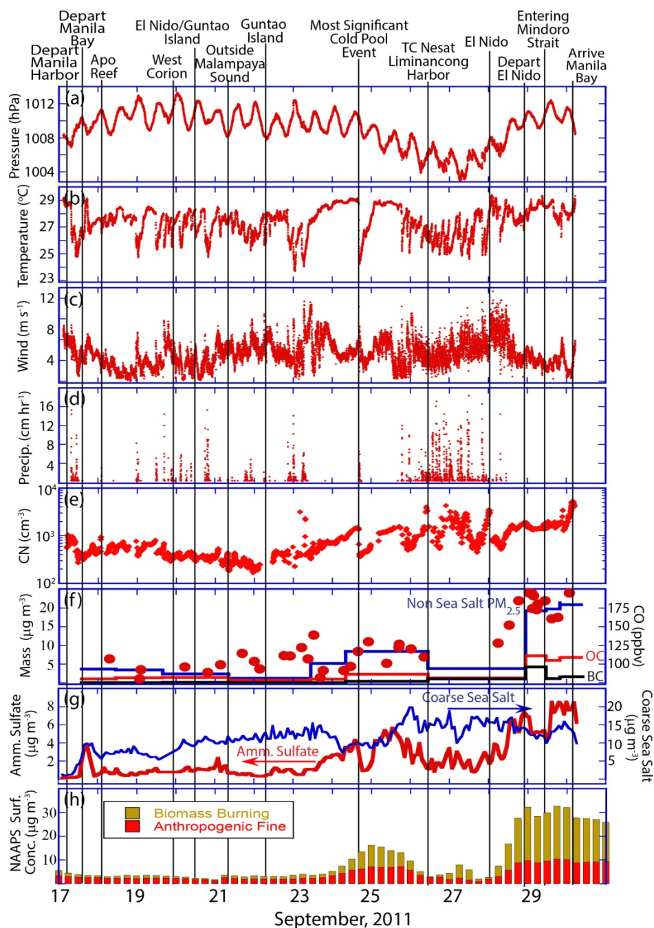
Figure 7. Cruise time series of key meteorological, aerosol and chemistry indicators in 1 minute intervals. Key sampling points and events are marked by vertical lines. (a) Surface pressure (hPa); (b) Ambient air temperature ( ^{\circ}\text{C} ); (c) Wind speed ( \text{m s}^{-1} ); (d) Precipitation rate ( \text{cm hr}^{-1} ); (e) CPC total particle count; (f) Left Axis: \text{PM}_{2.5} gravimetric mass with sea salt subtracted, and associated organic and black carbon; Right Axis-dots: Can Carbon Monoxide (ppbv); (g) Left Axis-red: DRUM impactor time series of inferred \text{PM}_{10} inferred ammonium sulfate ( \mu\text{g m}^{-3} ); Right Axis-blue: Inferred coarse mode sea salt ( d_p > 0.8 \mu\text{m} ). (h) NAAPS total fine mode particle mass segregated into Anthropogenic (+Biogenic) fine mode and biomass burning.
