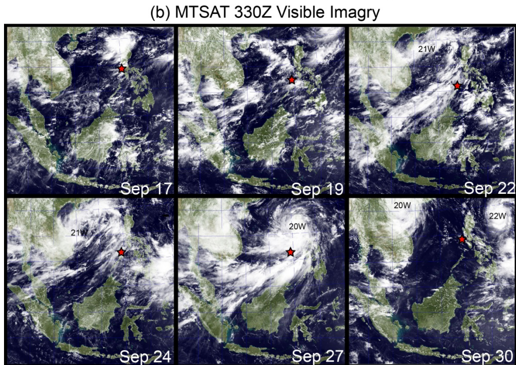
Figure 3. (a) Daily NOGAPS surface winds with CMORPH precipitation for 6 days throughout the cruise demonstrating key meteorological and aerosol modes. (b) Corresponding NexSat 330UTC/1130 LST MTSAT visible imagery with synthetic color background. Ship location at satellite imagery time is located by a red star.
