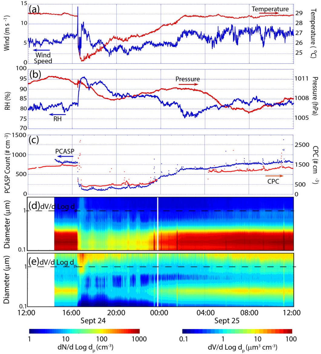
Figure 10. Twenty four hour times series of meteorology and aerosol parameters centered on the September 24 th cold pool event. Times are in UTC. (a) 1 minute temperature and wind speed; (b) 1 minute relative humidity and pressure; (c) PCASP and CPC total aerosol particle count; (d) and (e) PCASP number and volume distributions, respectively.
