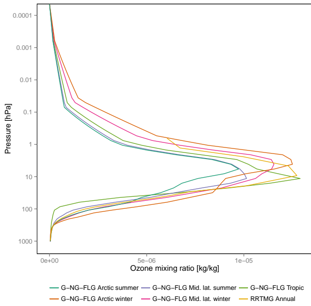
Fig. 1. Ozone profile datasets available in the G-NG-FLG and RRTMG parameterizations.
