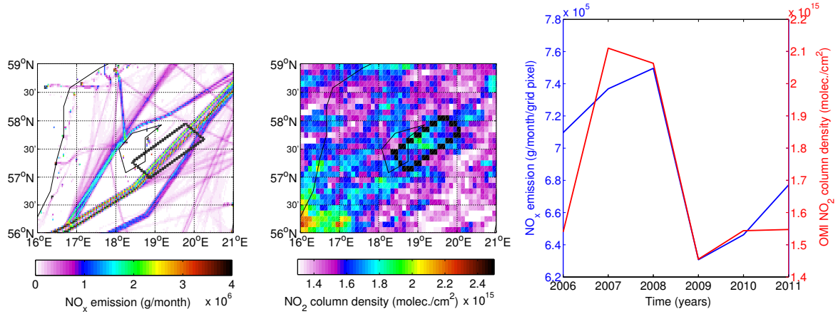
Fig. 6. Comparison between STEAM NO x emissions and OMI NO 2 tropospheric columns during the period 2006–2011. Left panel: July–August cumulative NO x emissions from STEAM; central panel: July–August mean NO 2 tropospheric columns from OMI; right panel: time series of both NO x emissions (blue line) and NO 2 columns (red line) as derived from the mean value within the black boxes in the left and central panel, respectively. Note that the axes have been selected so that the observed decreases have the same size in the plot.
