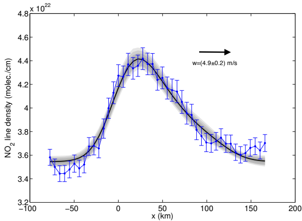
Fig. 4. OMI NO 2 line density (blue colour) for westerly wind conditions as a function of the distance ( x ) to/from Helsinki. Positive numbers in the x-axis are eastward from the city center. The error bars were derived using the error propagation for the discrete integral. The black line shows the MCMC fitted model and the grey areas correspond to the 50–99 % probability uncertainty regions.
