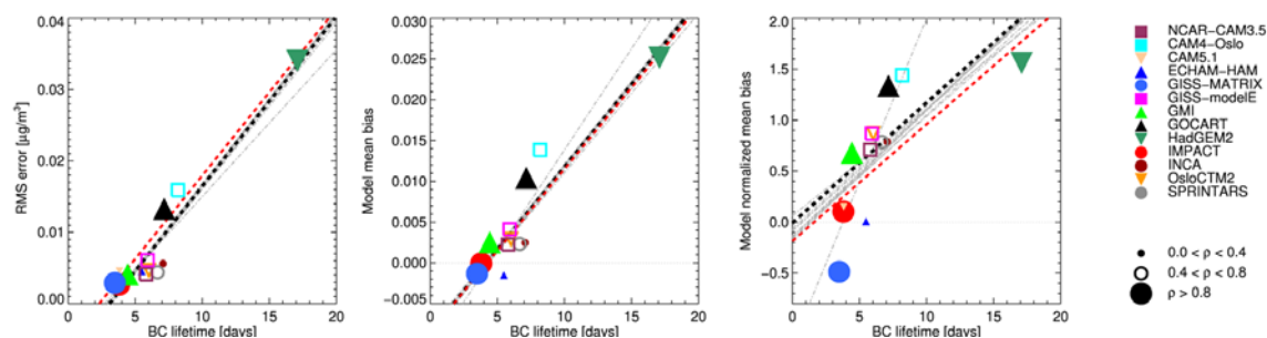
Figure 3: Modeled global black carbon lifetime plotted versus root-mean-square error, mean bias and normalized mean bias, between model prediction and observations for the five HIPPO regions (P1-P5). Each RMS or bias calculation is based on 72 data points. The symbol size indicates the corresponding Pearson correlation coefficient. The black dashed line shows a least-squares regression line with all models included. The grey lines show regressions with one model removed. The red dashed line shows a regression using only models with p > 0.8 .
