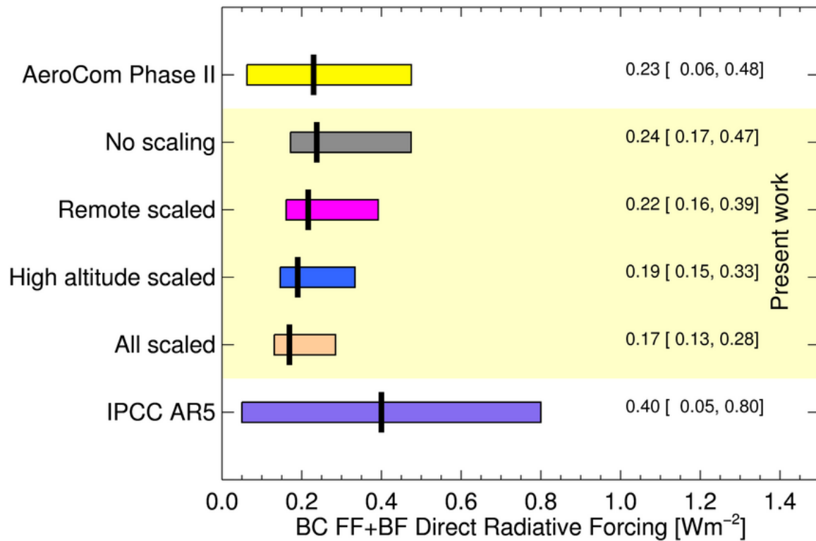
Figure 4: Model median and 5%-95% range for BC FF+BF forcing, for 1750-2010, with various scalings applied. The yellow bar shows the AeroCom Phase II result (Myhre et al., 2013b). The grey bar shows unscaled values from the present work, then with remote scaling (pink) and high altitude scaling (blue) applied. The khaki bar shows the lower limit on BC FF+BF forcing from the present work, with both scalings applied. Below we compare with the recent estimate in IPCC WG1's AR5.
