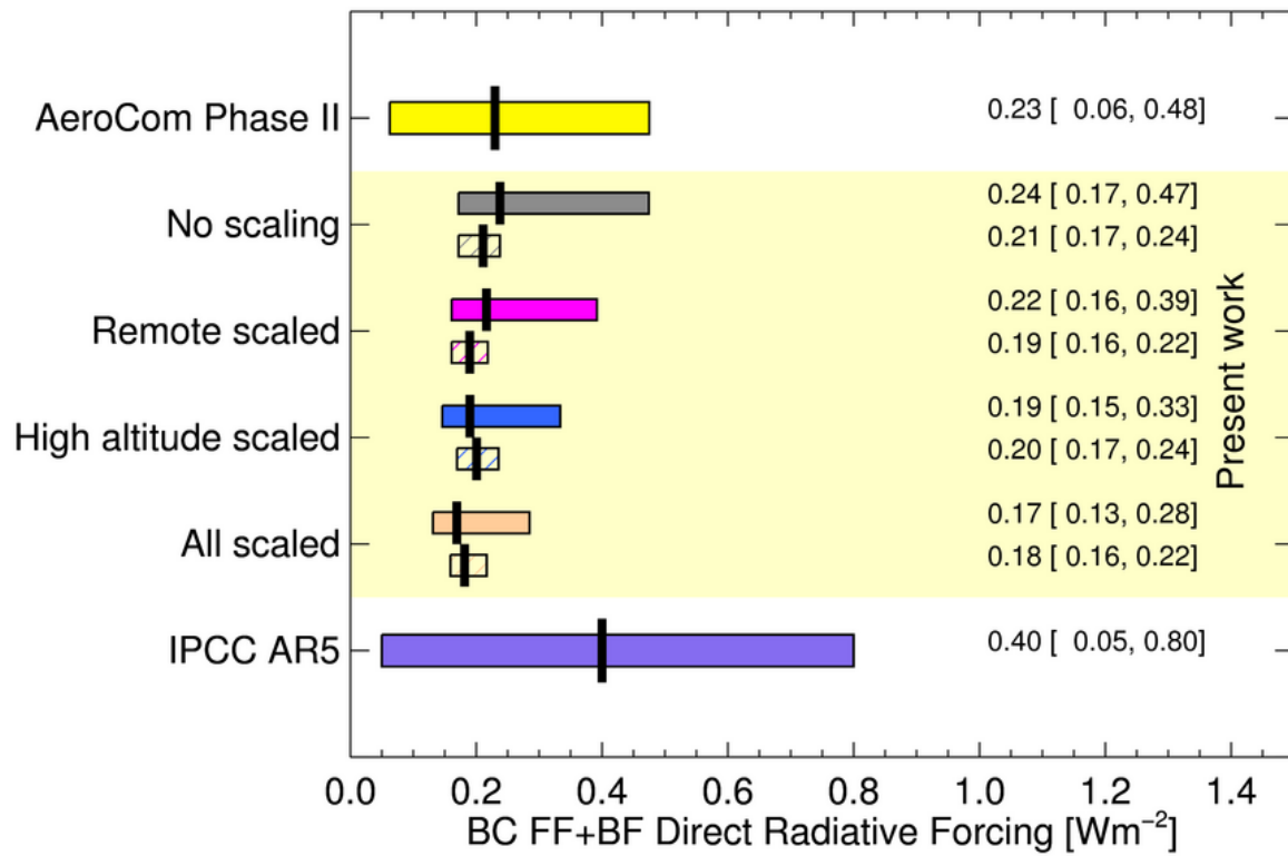
Figure 6: As Figure 4, except also showing the BC FF+BF forcing from the three models selected based on RMS and correlation vs HIPPO (hatched boxes).
