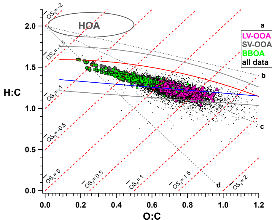
Figure 6. Van Krevelen-triangle diagram for time periods dominated by the given factor (as defined in Sect. 3.3) and for all data points. Estimated oxidation state, OS_c \approx 2 \times O:C - H:C (Kroll et al., 2011). Red and blue lines indicate the region usually inhabited by ambient data in the f_{43} vs. f_{44} plot; grey lines represent 10% error. Grey ellipse shows typical HOA values. (a) + alcohol/peroxide, m = 0 ; (b) carboxylic acid + fragmentation, m = -0.5 ; (c) + carboxylic acid (no fragmentation), m = -1 ; (d) + ketone/aldehyde, m = -2 (Ng et al., 2011).
