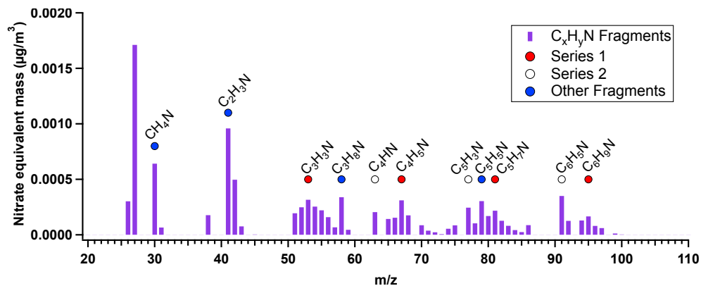
Figure 8. Rocky Mountain study-average mass spectrum of CHN fragments.
