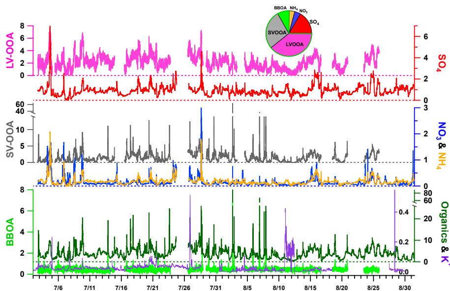
Figure 3. Time series of inorganic components, total organics, and organic factors (LV-OOA, SV-OOA, and BBOA) in \mu\text{g m}^{-3} . Potassium ( \text{K}^+ ) is from 17 min-average PILS-IC samples. Pie chart shows study-average contributions for each component; the dark green outline contains total organics.
