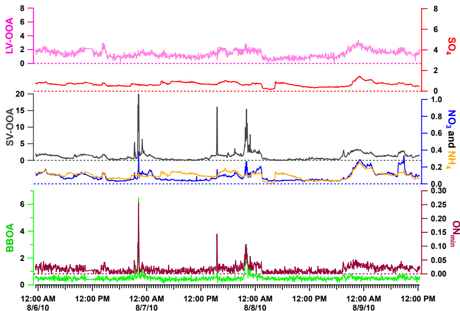
Figure 7. Time series showing select elevated- ON_{min} periods with inorganics and other organic factors from the Rocky Mountain National Park site.
