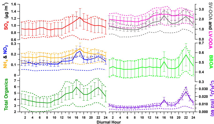
Figure 4. Study-average diurnal concentrations of particulate sulfate, nitrate, ammonium, total organics, BBOA, LV-OOA, SV-OOA, C_3H_3O^+ ( m/z 55), and C_2H_4O_2^+ ( m/z 60, levoglucosan). Solid lines are means, with \pm 20\% error bars reflecting AMS quantitation error. Dashed lines are 25th and 75th percentiles.
