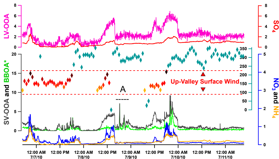
Figure 11. Timeline of species and relevant organic factor concentrations for 7–11 July 2010, plotted with 1 h surface wind direction at the site (diamonds). Wind directions 90 through 180° denote up-valley winds and are demarcated by dashed red lines and warm-colored diamonds. BBOA* is calculated using the six-factor PMF reconstructions outlined in the Supplement.
