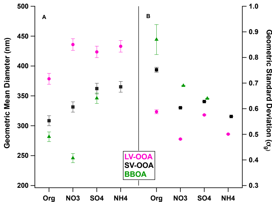
Figure 9. (A) Geometric mean diameter of the log normal mass size distribution fit for the indicated species or total organics for the average of time periods dominated by the color-designated organic factor; error bars are estimations of size-dependent PToF error, compounding chopper broadening and calibration-particle size standard deviation (Supplement). (B) Geometric standard deviation of the lognormal fit, with error bars equaling the reduced chi-squared value. Ammonium concentrations were too low during BBOA events for size determination.
