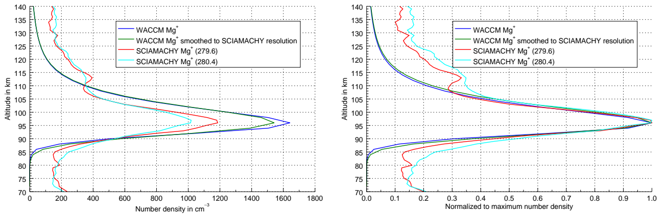
Fig. 20. Vertical profiles of \text{Mg}^+ for SCIAMACHY and WACCM at the equator. The right plot shows the profiles normalized to the maximum of each profile, to better compare the shape of the profiles. The VCD between 70 and 140 km at the equator is 2.7 \times 10^9 \text{ cm}^{-2} for SCIAMACHY (both 279.6 nm and 280.4 nm) and 2.4 \times 10^9 \text{ cm}^{-2} for WACCM. Note that the statistical error for SCIAMACHY estimated by Langowski et al. (2013) (Figs. 22 and 23) is \approx \pm 150 \text{ cm}^{-3} for the 279.6 nm line and \approx \pm 250 \text{ cm}^{-3} for the 280.4 nm line.
