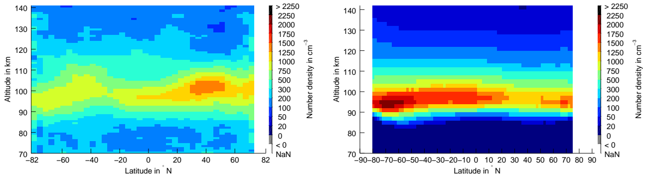
Fig. 18. Annual means of Mg^+ for SCIAMACHY (left, 280.4 nm) and WACCM (right). SCIAMACHY shows a wider vertical profile, and a stronger latitudinal dependence of the peak altitude. The peak densities are in very good agreement. The averaging for WACCM simulations is restricted to match the time periods, where SCIAMACHY measurements are available.
