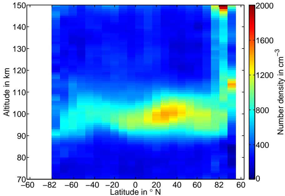
Fig. 21. \text{Mg}^+ profiles averaged over all available data for 2008–2012 for the \text{Mg}^+ line at 280.4 nm. The stray-light contaminated measurements at the start of the sunlit part of each orbit are also used here extending the coverage to higher northern latitudes and even the ascending node side. High \text{Mg}^+ densities are observed at the north pole. See Fig. 1 and Sect. 4 2nd paragraph for an explanation of the x-axis labels. Note that this is an older plot, which shows data with a wrong polarization correction, which is, however, unimportant for the effect shown here.
