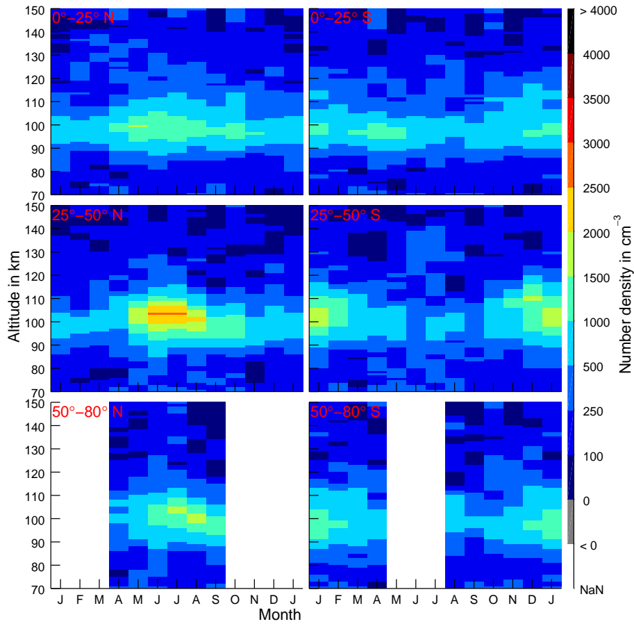
Fig. 8. Seasonal variation of the vertical profile of \text{Mg}^+ (280.4 nm line) for different latitudinal zones (left: NH, right: SH, top: low latitudes, mid: mid latitudes, bottom: high latitudes), averaged over all available observations in 2008–2012. For all these latitudinal zones a seasonal cycle in the peak altitude with a summer maximum and a winter minimum can be observed. The seasonal variations are similar or larger than the month-to-month variations. The maximum peak altitude is 5–10 km higher than the minimum peak altitude. For mid latitudes, the peak altitude in the winter hemisphere is still higher than the peak altitude at the equator (see also Fig. 6).
