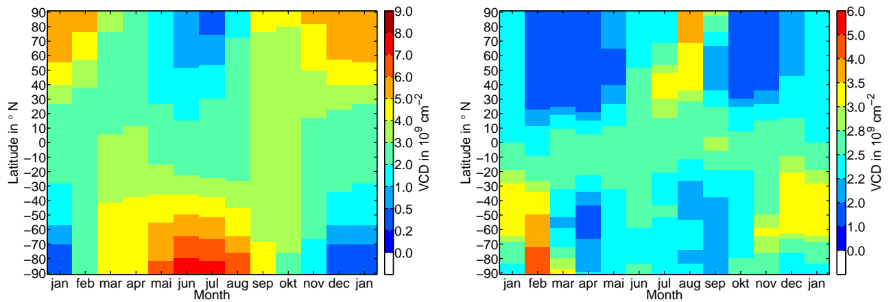
Fig. 16. WACCM VCD timelines for different latitudes for Mg (left) and Mg^+ (right). Mg VCD vary between 0.5 \times 10^9 \text{ cm}^{-2} and 8 \times 10^9 \text{ cm}^{-2} and show a clear seasonal cycle with a winter maximum, which is most pronounced at the poles. Mg^+ VCD vary from 1 \times 10^9 \text{ cm}^{-2} to 5 \times 10^9 \text{ cm}^{-2} , with most VCD between 2 \times 10^9 \text{ cm}^{-2} and 3 \times 10^9 \text{ cm}^{-2} . A clear seasonal cycle with a summer maximum for Mg^+ is observed. SCIAMACHY results of VCD are shown in Figs. 5 and 9.
