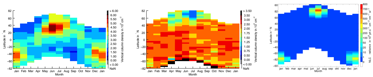
Fig. 24. Vertical column densities of Mg^+ (left), Mg (mid) and NLC radiance (right) retrieved from SCIA-MACHY. A clear reduction of Mg^+ and Mg VCD is observed in the vicinity of NLC. However, this is also observed in neighbouring regions without NLC and can also be explained by other processes. (Note that the NLC retrieval includes more latitudes from the ascending node side).
