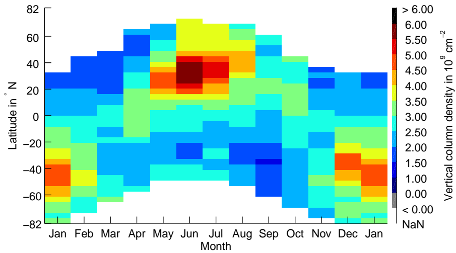
Fig. 9. Seasonal variation of the \text{Mg}^+ vertical column density (VCD) between 70 km and 150 km and for different latitudinal regions, retrieved from the 280.4 nm line. A clear seasonal cycle with a summer maximum can be observed. The summer maximum in the NH has higher values compared to the one in the SH. The highest variability can be found between 25^\circ and 50^\circ in both hemispheres.
