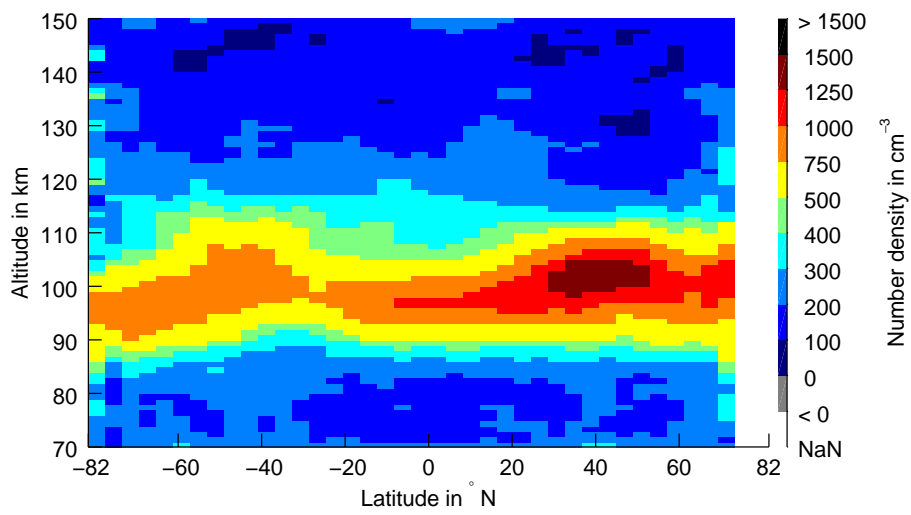
Fig. 7. Latitudinal variation of \text{Mg}^+ profiles averaged over all available data for 2008–2012 for the \text{Mg}^+ line at 280.4 nm.
