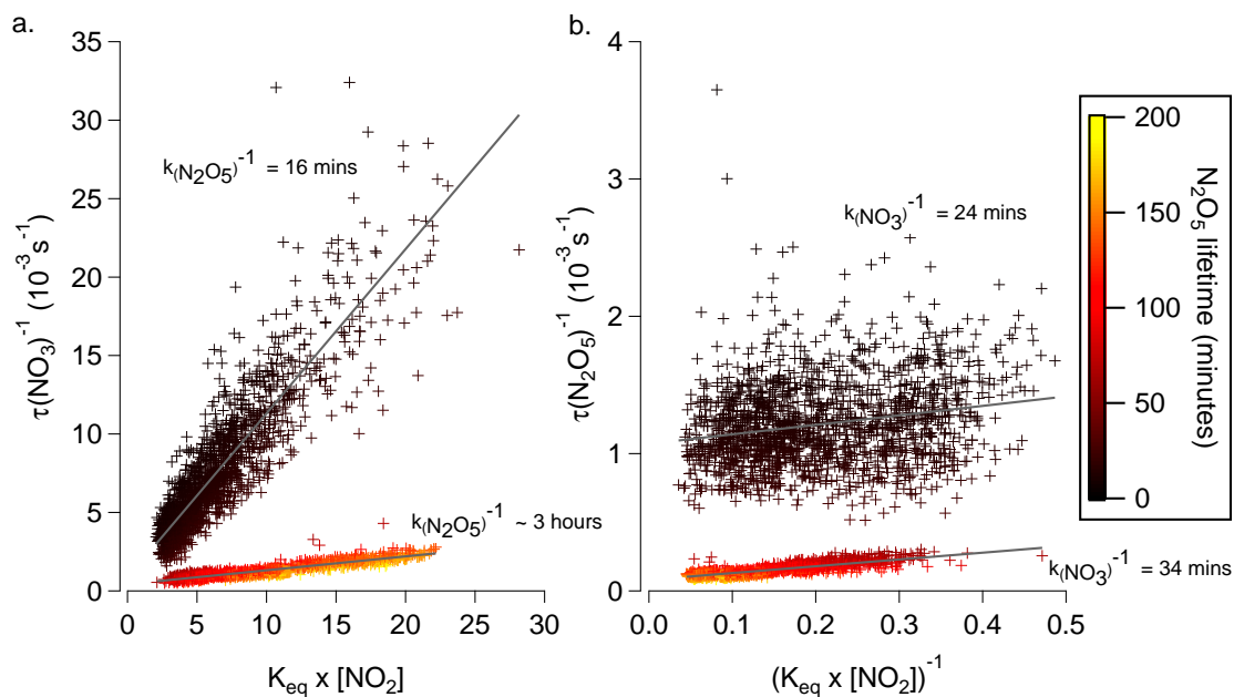
Fig. 4. Plots of \tau_{ss}(\text{NO}_3)^{-1} against K_{eq}[\text{NO}_2] (a) and \tau_{ss}(\text{N}_2\text{O}_5)^{-1} against (K_{eq}[\text{NO}_2])^{-1} (b), which allows calculation of the first-order rate coefficients k_{\text{NO}_3} and k_{\text{N}_2\text{O}_5} . The two plumes show the extremes in \text{N}_2\text{O}_5 lifetimes observed for the steady-state analysis. Points are coloured according to the \text{N}_2\text{O}_5 lifetime. The slopes with a short lifetime (darker colours) are from B537, while the slopes with a longer lifetime (lighter colours) are from B542. The solid grey lines are the linear fits to the data, with the inverse values for each slope given on the plots in units of time i.e. minutes or hours.
