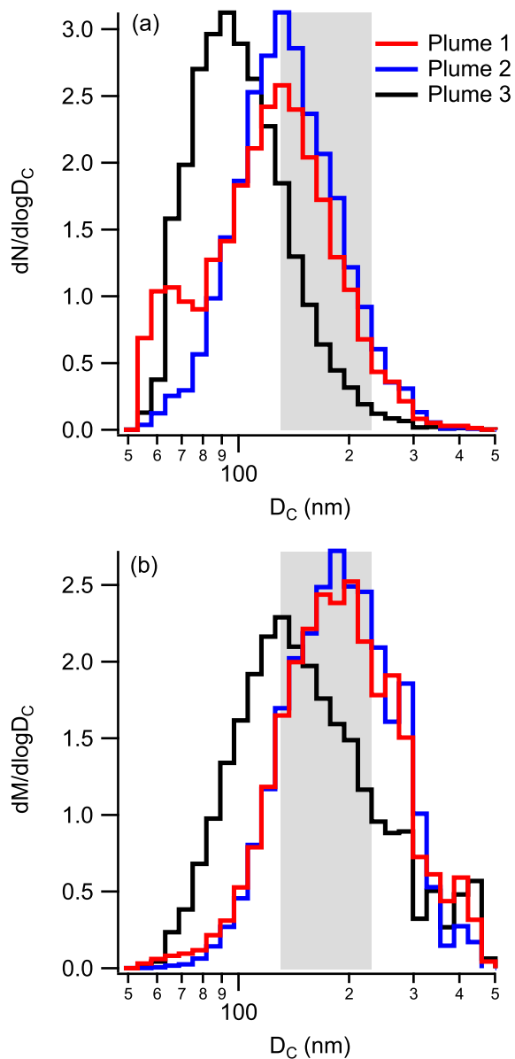
Figure 5. Normalised average BC core size distributions measured by the SP2 during for the three plumes. Part (a) presents the number distribution, and part (b) the mass distribution. The discontinuity at \sim 300 nm is due to saturation of the broadband detector and switching to the narrowband. The grey shaded regions show the range of core diameter used for calculating coating properties.
