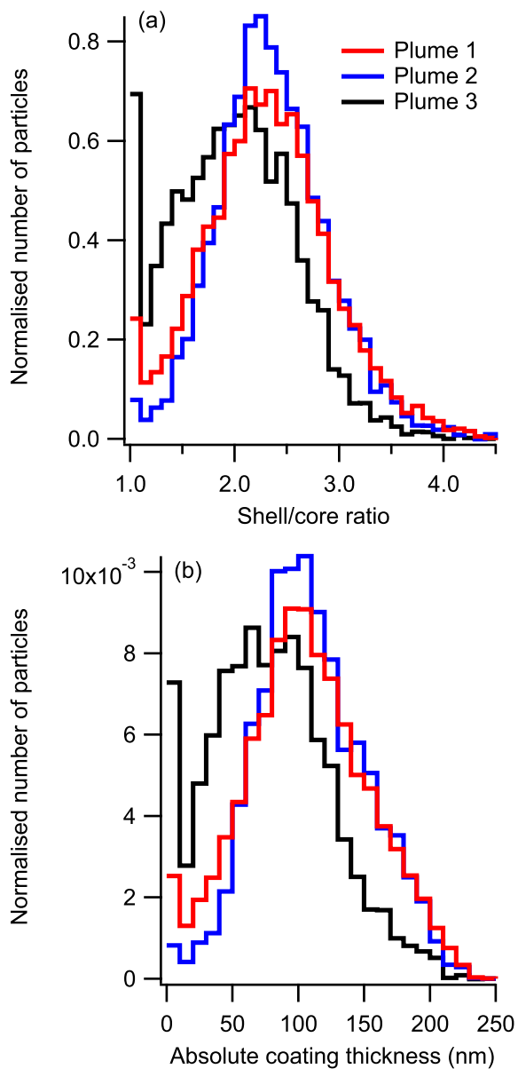
Figure 6. Distributions of measured coating thicknesses, measured by the SP2, expressed in terms of (a) shell/core ratio and (b) absolute coating thickness. The first bin ( D_P = D_C = 1 , uncoated particle) also contains all particles with measured scattering less than that predicted for an uncoated core (equivalent to D_P < D_C ). Such particles are a result of random variations in the detected scattering, however as the result D_P < D_C is nonphysical they are assigned the nearest realistic value.
