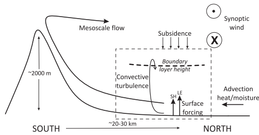
Fig. 1. Sketch of the main process driving the development of the atmospheric boundary layer observed on June 25, 2011 (IOP5). The majority of the surface stations were located near the main site (see Fig. 4) whereas the aircraft measurements were gathered in an East West direction during the case under study. Note that the shear produced by the opposite wind direction is occurring above the boundary layer ( \sim 600 m) as shown at Fig. 3.
