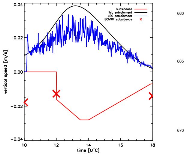
Fig. 7. Temporal evolution of the entrainment velocity and prescribed subsidence velocities at the top of the boundary layer for the run with prescribed subsidence (case 2). The subsidence values calculated by ECMWF model are also shown.
