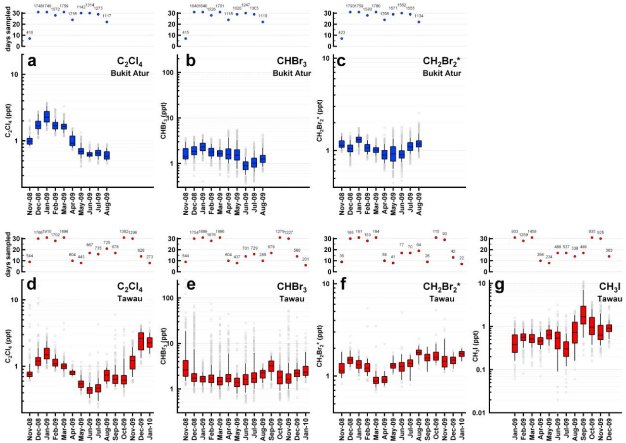
2 Figure 4(a-g): Box and whisker plots for the halocarbon observations at Bukit Atur for (a) C_2Cl_4 , 3 (b) CHBr_3 , (c) CH_2Br_2^* and at Tawau for (d) C_2Cl_4 , (e) CHBr_3 , (f) CH_2Br_2^* and (g) CH_3I . In each 4 panel, the coloured boxes show the data falling between the 25 th and 75 th percentiles, with the 5 median value shown as a black horizontal line inside each box. The vertical black lines above and 6 below each box indicate the 95 th and 5 th percentiles respectively. Outliers (values beyond the 95 th 7 and 5 th percentiles are shown as grey open circles. The mixing ratio (y-axis) scale is logarithmic in 8 order to show the extreme high values, such as for CHBr_3 at Tawau (e). The filled circles in the 9 smaller panel above each box and whisker plot show the number of days sampled each month and 10 labels indicate the number of samples used to generate each box and whisker. The total sample 11 count is different at each site due mainly to different periods of instrument down time and 12 differences in the sampling frequency at each site.
