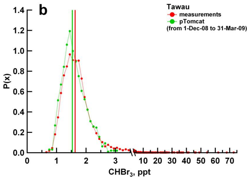
1 2 Figure 7(a & b): Time series (a) of observed (red dots) and p-TOMCAT modelled (green line) 3 CHBr 3 at Tawau and probability distributions (b) for observed (red circles with red dotted line) and 4 modelled CHBr 3 (green circles with green dotted line) for December 2008 to March 2009. The 5 black vertical error bar in (panel a during May 2009) shows the typical CHBr 3 measurement 6 precision ( \pm 1 s.d.) for the whole observational period. Median CHBr 3 mixing ratios are indicated 7 (b) by the red solid line for the observations and by the green solid line for the model. The model 8 compares well overall with the observations though there are periods when the model 9 underestimates the observations (e.g. October 2009). The model does not capture the full variability 10 of the observations which is expected given the model resolution and the uniform distribution of 11 coastal emissions in the model, this is illustrated by absence of the high tail in the modelled CHBr 3 12 (b).
