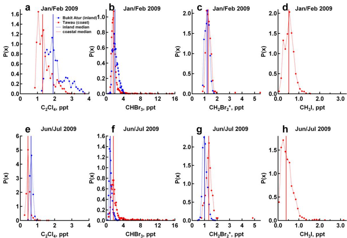
2 Figure 5(a-h): Probability distributions and median values at each site for January/February 2009 3 (merged) for (a) C_2Cl_4 , (b) CHBr_3 , (c) CH_2Br_2^* , (d) CH_3I (Tawau only) and June/July 2009 4 (merged) for (e) C_2Cl_4 , (f) CHBr_3 , (g) CH_2Br_2^* and (h) CH_3I (Tawau only). Bukit Atur distributions 5 are shown as blue circles with dotted blue lines and Tawau as red circles with dotted red lines. 6 Median values for inland Bukit Atur are shown by solid vertical blue bars and for coastal Tawau by 7 solid vertical red bars. The bin width for each probability distribution is 0.1 ppt and the area under 8 each curve is equal to 1 (probability of 1). High values beyond the scale of x-axis are not shown, for 9 instance the high tail is not wholly visible for CHBr_3 at Tawau (b & f), though all data are included 10 in the box and whisker plots (Figure 4).
