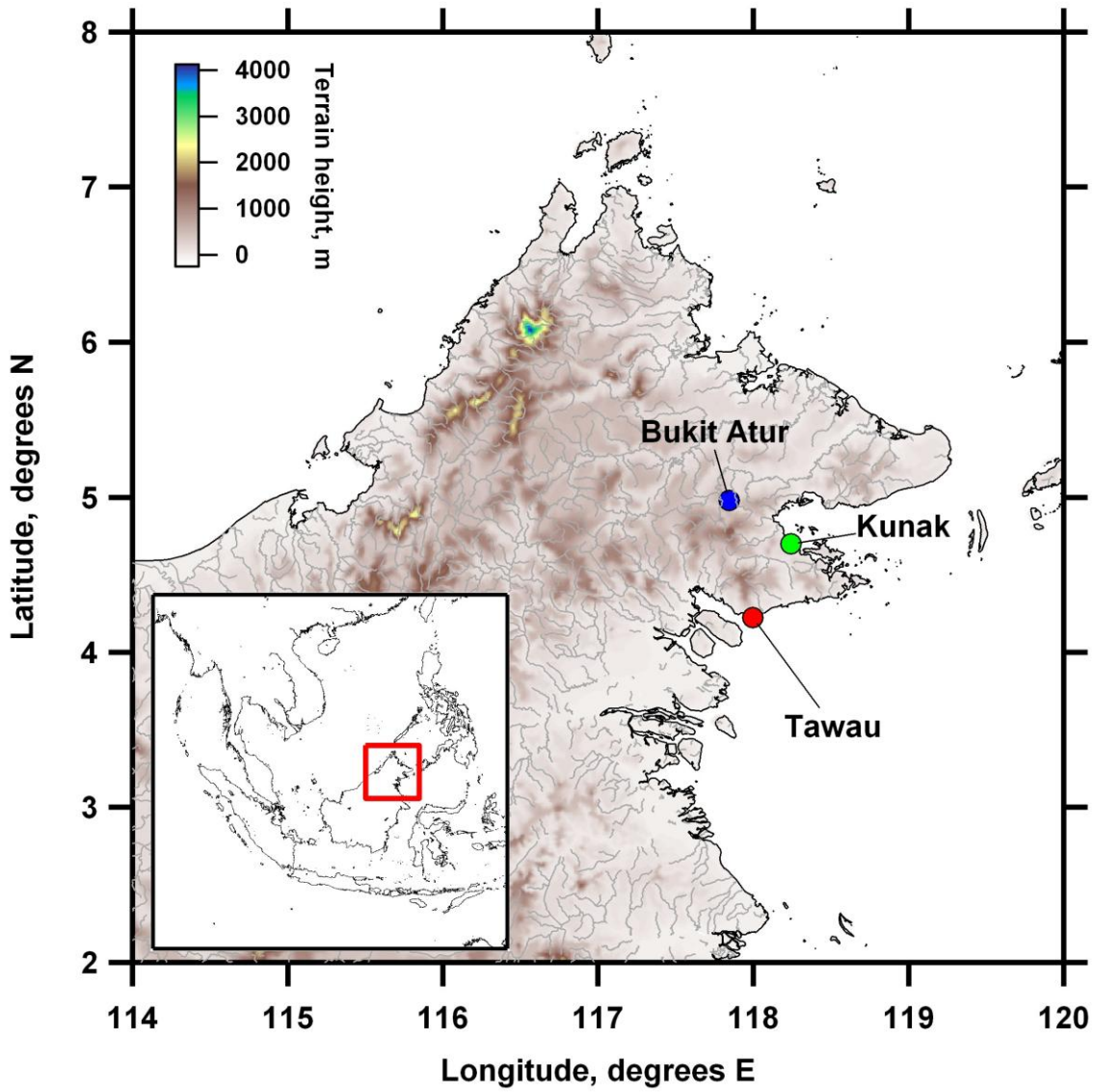
2 Figure 1: Site location map for Sabah. The inland rainforest site on Bukit Atur is shown by the blue 3 circle, the coastal site near Tawau is a red circle and the coastal site at Kunak (green circle) is also 4 shown as featured in Pyle et al. (2011). The Tawau site is ~85 km to the south of Bukit Atur. The 5 inset (lower left corner of main panel) shows the southeast Asia region with a red square to show 6 coverage of the main map.
