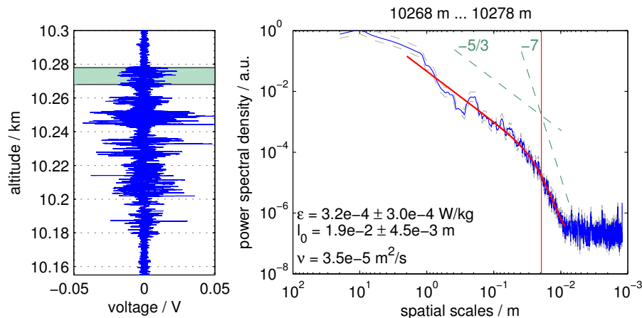
Figure 1. Example of raw data (left) and associated power spectrum (right) computed for the shaded area in the raw data plot. In the raw data, an amplitude of \lesssim 1 mV corresponds to instrumental noise. In the spectrum, the blue curve shows the measurement, the grey dashed lines the 95% confidence interval and the red curve the fit of the Heisenberg model to the measured spectrum, the red vertical line indicates the inner scale l_0 . The green dashed lines visualise slopes of -5/3 and -7 . The errors given are fit errors.
