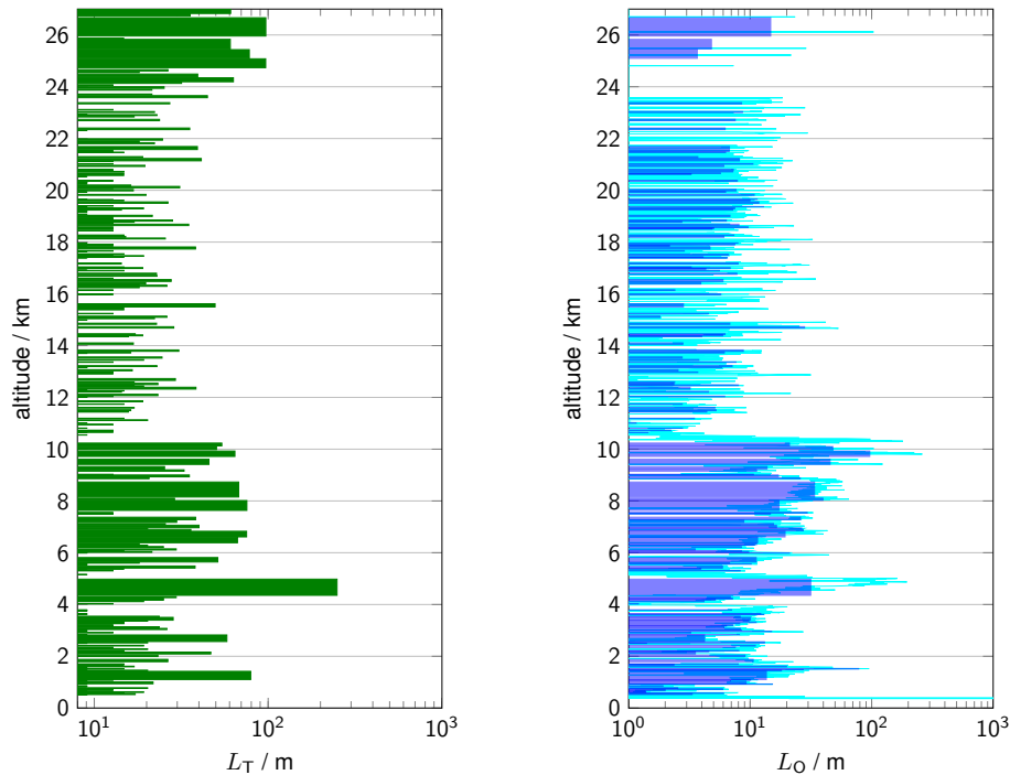
Figure 3. Thorpe length (left) and Ozmidov scale (right) vs. altitude for the detected inversions of the BEXUS 12 flight. The cyan curve shows the Ozmidov scale in the full resolution of the LITOS profile, the blue one averages over the inversions detected by the radiosonde.
