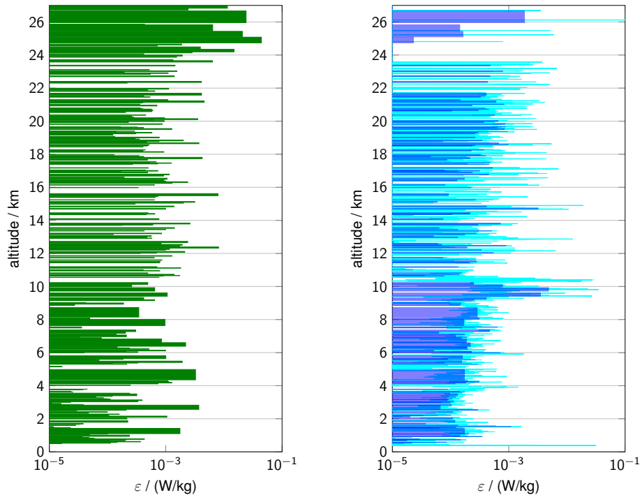
Figure 7. Energy dissipation rates from Thorpe analysis of the radiosonde (left) and spectral analysis of the high-resolved wind measurement (right) for the BEXUS 12 flight. The cyan curve shows the full resolution, the blue one averages over the unstable layers detected by the Thorpe analysis.
