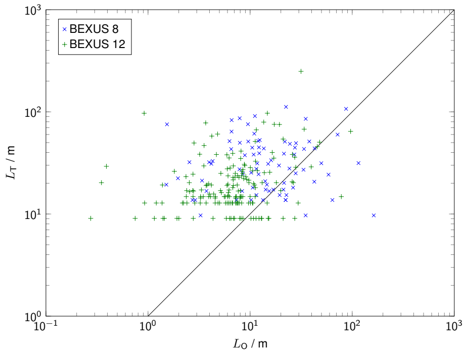
Figure 5. Thorpe scale L_T vs. Ozmidov scale L_O for the BEXUS 8 (blue) and 12 (green) flights. The black diagonal line represents L_O = L_T . Note that L_T is limited by the resolution of the radiosonde ( \sim 10 m).
