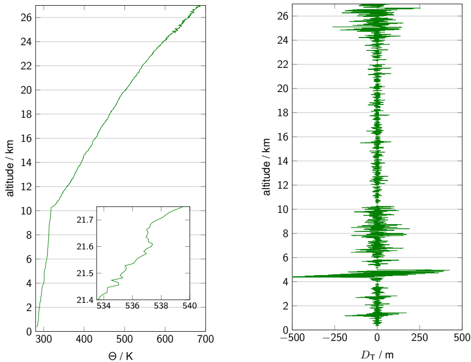
Figure 2. Potential temperature profile (left) and Thorpe displacement (right) for the BEXUS 12 flight. The inset in the left panel shows a magnification from 21.4 to 21.75 km for better visibility of instabilities (manifested as negative gradients of potential temperature).
