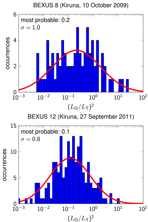
Figure 6. Statistics for the ratio (L_O/L_T)^2 for the BEXUS 8 (top) and BEXUS 12 (bottom) flights. The red curves show the most likely normal distributions for the logarithmic data.
