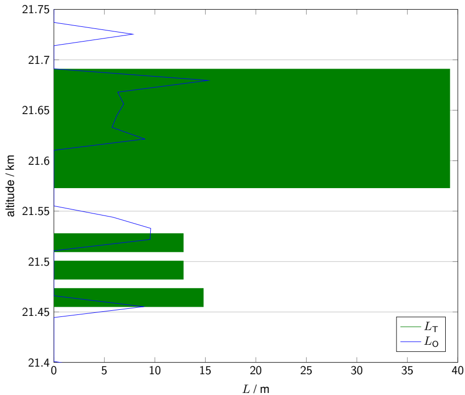
Figure 4. Detail plot of Thorpe (green) and Ozmidov (blue) scales for the BEXUS 12 flight.
