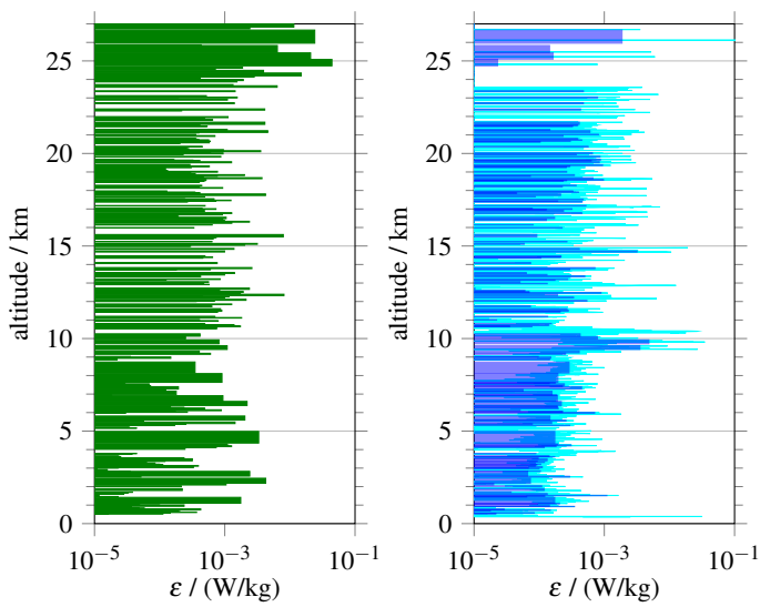
Figure 7. Energy dissipation rates from Thorpe analysis of the radiosonde (left) and spectral analysis of the high-resolved wind measurement (right) for the BEXUS 12 flight. The cyan curve shows \varepsilon in the full resolution, the blue one averages over the unstable layers detected by the Thorpe analysis ( \langle \varepsilon \rangle ).
