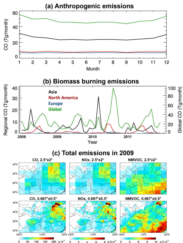
Figure 3. (a) Monthly anthropogenic (fossil + biofuel) emissions of CO within the nested and global model domains; emissions are unchanged from one year to another. (b) Monthly biomass burning emissions of CO over 2008–2011 within the nested or global model domains. (c) Spatial distributions of CO, NO x and NMVOC emissions from all sources in 2009 over eastern China on the global vs. nested grids.
