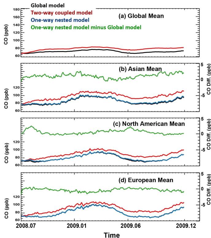
Figure 5. Daily mean tropospheric mean CO mixing ratio from July 2008 through December 2009 averaged over the global or nested model domains simulated by the global model alone (black), by the two-way coupled model (red), and by the one-way nested model (blue; with no feedbacks to the global model; only for nested domains). Also shown in (b–d) is the difference between the one-way nested and the global model (green; right axis).
