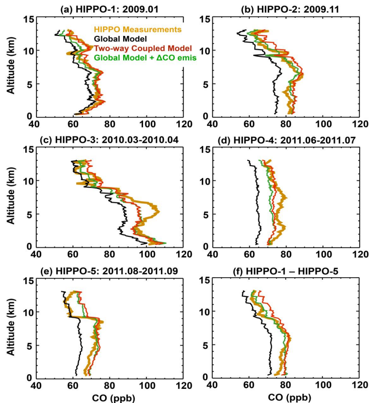
Figure 8. Measured and simulated vertical profiles of CO at 0.1 km intervals averaged over (a–e) individual and (f) all HIPPO campaigns. Model results are sampled at times and locations coincident to HIPPO measurements. Green lines represent global model simulations with increased global CO emissions that roughly resemble the two-way coupled simulation (especially below 4 km); increases in CO emissions are 15% for HIPPO-1, 25% for HIPPO-2, 15% for HIPPO-3, 25% for HIPPO-4, and 35% for HIPPO-5.
