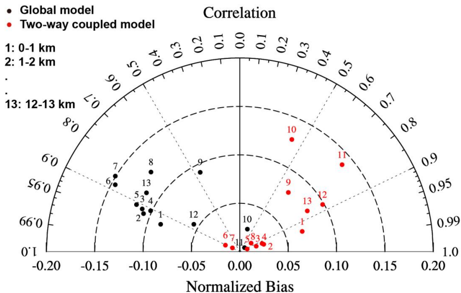
Figure 7. Correlation and mean normalized bias of modeled CO with respect to HIPPO measurements throughout the HIPPO campaigns, for individual vertical layers (0–1 km, 1–2 km, etc.).
