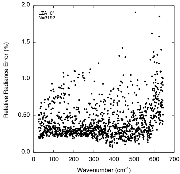
Figure 6. Relative radiance estimation error for the FIR region. Calculated from the root mean square values of the radiance errors divided by the mean radiance spectrum (the right and left plots of Figure 5 respectively).
