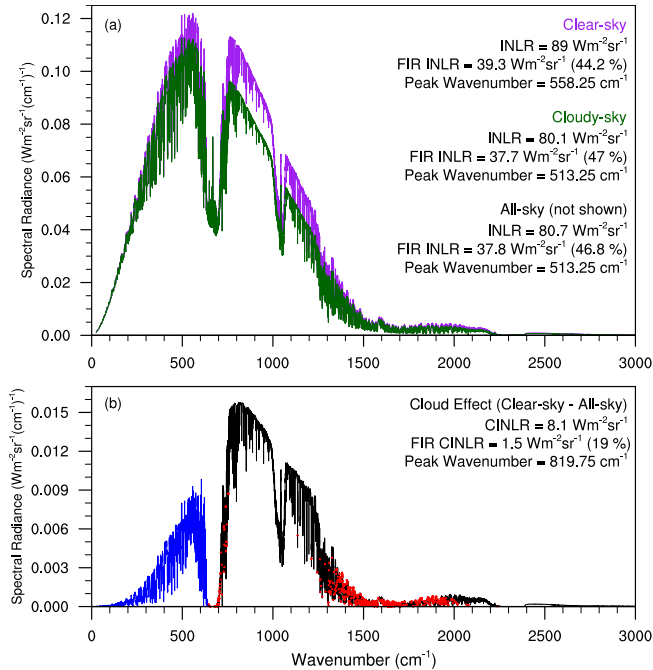
Figure 11. The outgoing longwave spectral radiance constructed from IASI data globally averaged for: a) clear (purple) and cloudy (green) pixels. Numbers in parentheses are the fractional FIR contributions to the total LW broadband INLR. The all-sky curve is between the clear and cloudy curves but is not plotted for clarity. b) The difference between the clear-sky and all-sky spectrum's constructed from IASI measurements (black) and estimated far infrared radiances (blue) from predictor wavelengths in the mid infrared with the highest correlations (red dots). The number in parentheses is the fractional contribution of the FIR INLR (FIR CINLR) to the total INLR (CINLR). Data is the area weighted mean of April 2012.
