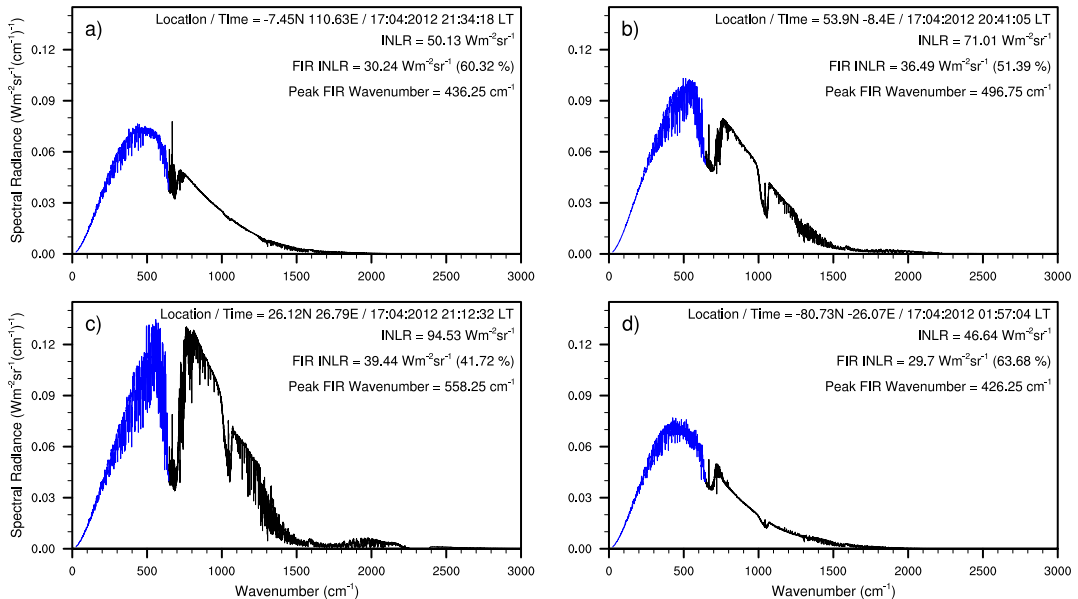
Figure 10. The total outgoing longwave spectral radiance ( 25.25 - 2999.75 \text{ cm}^{-1} ) constructed from IASI measurements (black) and estimated far infrared radiances (blue) for 4 instantaneous scenes over: a) tropical equatorial land, b) midlatitude land, c) the Sahara desert, and d) Antarctica. All are night-time scenes from the 17th April 2012.
