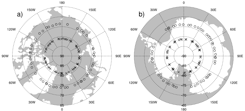
Figure 7. Locations of nearest nadir viewing SNOs, chosen as described in section 2.4 between Metop-A and Terra (inner crosses) and Aqua (outer circles) for a) the Arctic, and b) Antarctic, for 2012.
