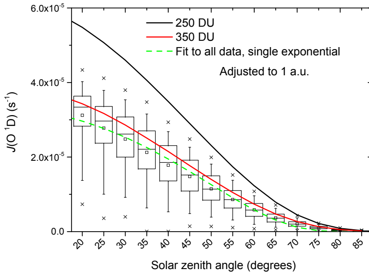
Figure 4. Solar zenith angle dependence of J(\text{O}^1\text{D}) . Crosses mark the 1 and 99 percentile. The boxes span 25/75 %, the whiskers mark 10 and 90 %, the central line indicates the median and the square the average value. The x axis value is the central value of the 5^\circ bin used. The two solid lines were calculated using TUV (V 5.0) for ozone column amounts of 250 DU (February) (black solid line) and 350 DU (September) (red dashed line). The short-dashed green line is the fit to a single exponential term to all data.
