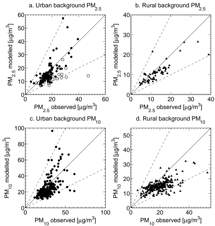
Fig. 5. Bottom-up calculated vs observed PM 2.5 and PM 10 concentrations at urban and rural background monitoring stations in 2009. Panel (a) distinguishes into stations located in cities > 100000 inhabitants (dots) and those not (circles). For better viewing, only urban stations in cities > 100000 inhabitants are shown for PM 10 (c).
