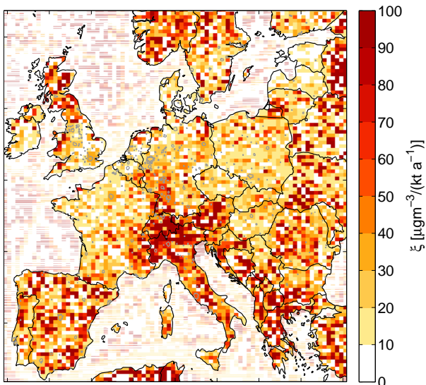
Fig. 3. The regression coefficient \xi relating additional primary PM emissions within each EMEP grid cell to PM concentration increments.
