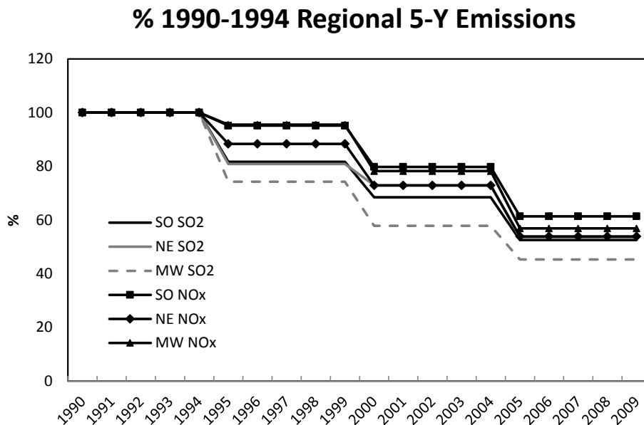
Figure 3. Estimates of regional mean annual SO 2 and NO x emissions for four 5 year periods (P1, P2, P3, and P4) between 1990 and 2009, expressed as percentages of the 1990–1994 (P1) regional means. In the SO, NE, and MW mean P1 SO 2 emissions are 3.48, 1.68, and 3.27 Tg S yr -1 , and mean P1 NO x emissions are 1.89, 1.06, and 1.35 Tg N yr -1 (Xing et al., 2013).
