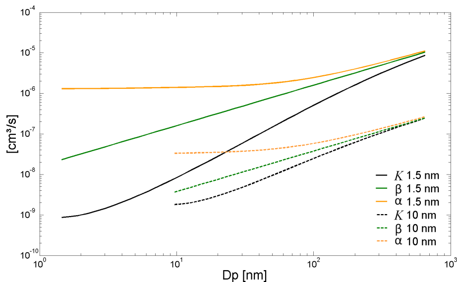
Fig. 1. Coagulation coefficient K , attachment coefficient \beta and recombination coefficient \alpha [ \text{cm}^3 \text{s}^{-1} ] for small cluster ions and particles (1.5 nm, solid lines) and large ions and particles (10 nm, dashed lines) as function of ions and particles of diameter D_p .
