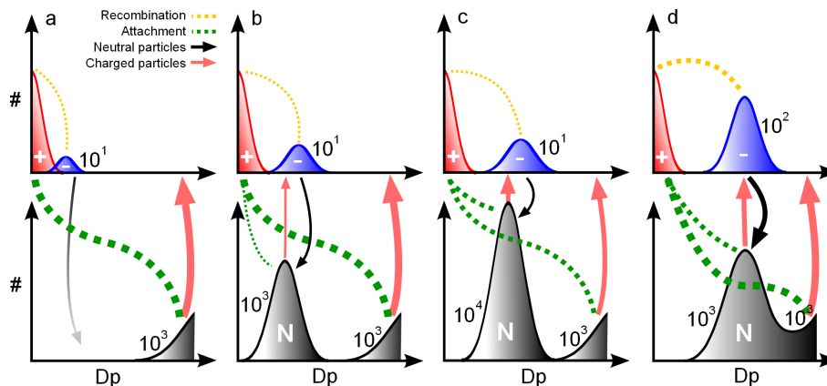
Fig. 9. Conceptual model of the influence of cluster ion recombination and attachment at different stages of particle nucleation and growth (a–d). Permanently available positive cluster ions are denoted in red, the negative growing mode in blue and neutral particle modes in black. The black and red arrows denote the generation of neutral and charged particles, respectively. The size of the arrows and dashed lines denotes the prevailing mechanism. Numerals indicate the orders of magnitude of the number concentrations of the respective modes.
