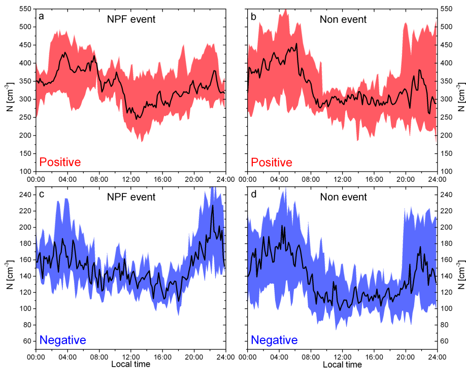
Fig. 3. Median diurnal variation of cluster ion concentrations (diameter < 1.6 nm) during 8 selected NPF event days ( a , c ) and 13 non-event days ( b , d ), as measured with the NAIS during summer 2012 at the “Waldstein” site. The shaded areas denote the 25th and 75th percentile.
