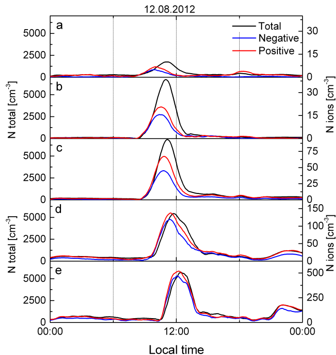
Fig. 4. Temporal evolution of total particle concentrations as well as positive and negative ion concentrations in diameter ranges of (a) 1.8–2.1 nm, (b) 3.7–4.3 nm, (c) 7.6–8.8 nm, (d) 13.6–15.7 nm and (e) 21.1–24.5 nm. The data originates from single NAIS size channels, measured during the NPF event on 12 August 2012 at “Waldstein”. Ion concentrations increase during the growth process, while total particle concentrations increase rapidly at the beginning of NPF but begin to decrease at diameters above 8 nm. Note that the ion concentrations (right axes) are always smaller than the particle concentrations (left axes). Data was smoothed for illustrational purpose.
