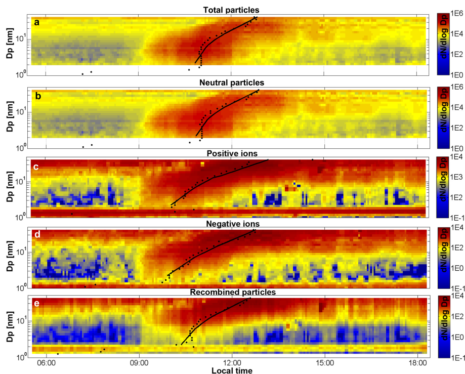
Fig. 2. NPF event of 12 August 2012 as measured with the NAIS. Shown are (a) total particles, (b) neutral particles, (c) positive ions, (d) negative ions and (e) calculated neutral particles from ion–ion recombination. Black filled circles denote the concentration maxima for each size class, while black lines are smoothed fits in order to obtain continuous growth rates.
