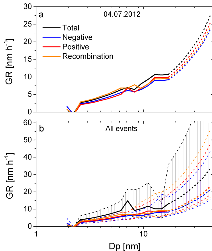
Fig. 6. Growth rates of negative ions, positive ions and total particles determined from NAIS measurements, (a) for a single event on 4 July 2012 and (b) median values for all 8 selected NPF events used for this study. Hatched areas denote the 25th and 75th percentile. Additionally, \text{GR}_{\text{rec}} deduced from ion–ion recombination is shown in orange. Dashed segments of the curves denote inaccurate growth rates.
