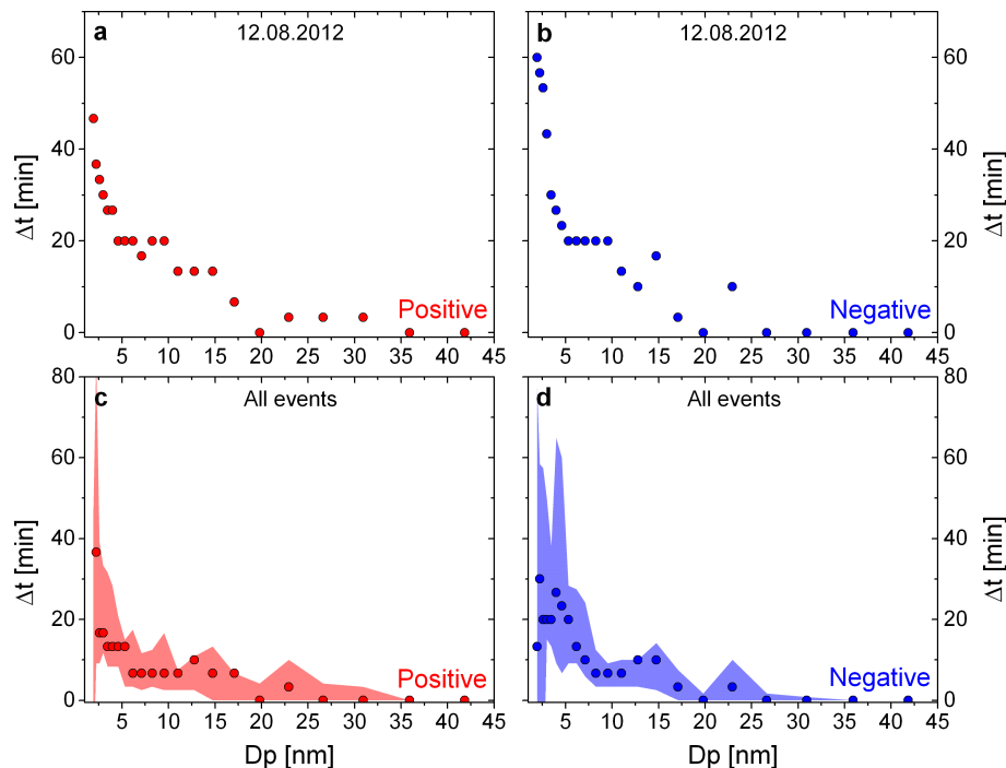
Fig. 5. Results from the cross-correlation study showing the size-dependence of the time difference ( \Delta t ). Appearance of (a) positive and (b) negative ions compared to total particles measured with NAIS on 12 August 2012, and median values of \Delta t for all 8 selected NPF event days for (c) positive and (d) negative ions. Shaded area denote the 25th and 75th percentile
