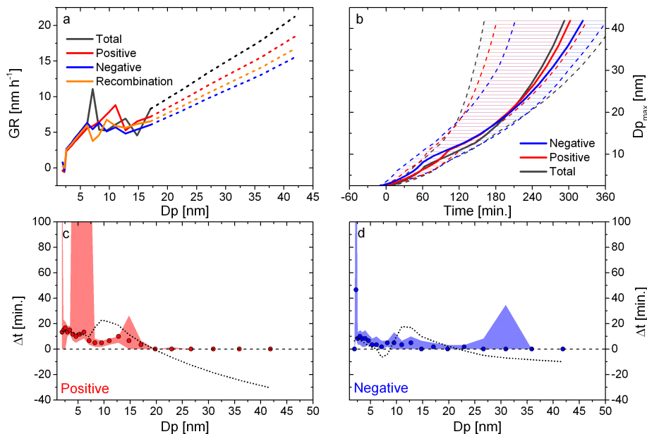
Fig. 8. Same as Fig. 7 but for four NPF events with \Delta t < 20 min.
