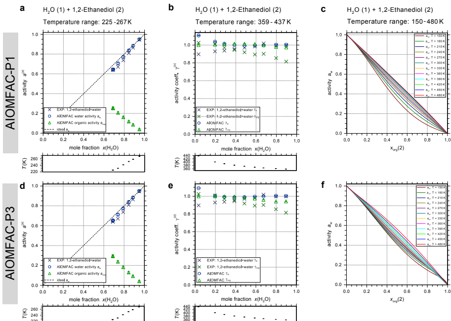
Figure 2. SLE and VLE measurements for water (1) + 1,2-ethanediol (2) solutions and corresponding calculations of AIOMFAC-P1 (a – c) or AIOMFAC-P3 (d – f). The coloured curves in (c, f) represent the temperature dependence of water activities predicted for the range 150 – 480 K. (a, d) Low temperature experimental SLE data (crosses) are compared with the predictions for water activity at the same compositions and temperatures (blue circles). Predictions of the corresponding organic activities are shown as well (green triangles). The dashed line represents the hypothetical water activity of an ideal mixture. The error bars represent the model sensitivity to a composition variation by x^{\text{tol}} = 0.01 . Panels (b, e) show the model predictions of the activity coefficients compared to VLE data covering temperatures significantly higher than room temperature. The temperatures of the individual data points are given in the boxes below the main panels. Experimental data: Ott et al. (1972) and Gmehling and Onken (2003a).
