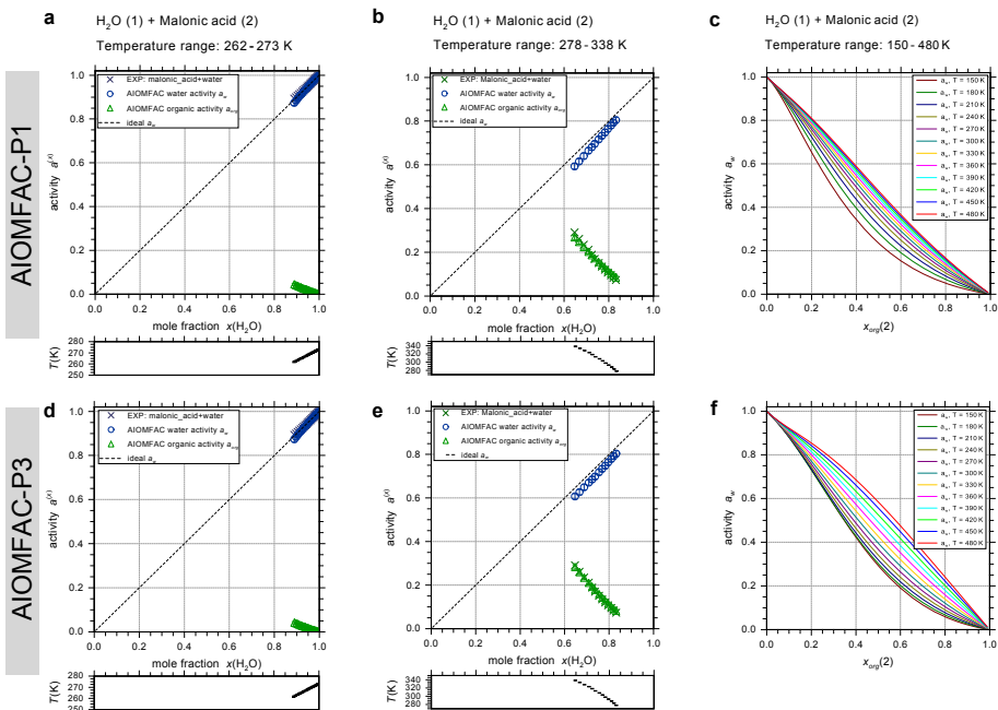
Figure 4. SLE measurements for water (1) + malonic acid (2) solutions and corresponding calculations of AIOMFAC-P1 (a – c) or AIOMFAC-P3 (d – f). Panels (c, f) show the temperature dependence of water activities predicted for the range 150 – 480 K. (a, d) Low temperature experimental SLE data (crosses) are compared with the predictions for water activity at the same compositions and temperatures (blue circles). Predictions of the corresponding organic activities are shown as well (green triangles) while (b, e) show analogous SLE data for the malonic acid melting curve. The error bars represent the model sensitivity to a composition variation by x^{\text{tol}} = 0.01 . The dashed line represents the hypotheticalal water activity of an ideal mixture. The temperatures of the individual data points are given in the boxes below the main panels. Experimental data: Braban et al. (2003) and Apelblat and Manzurola (1987).
